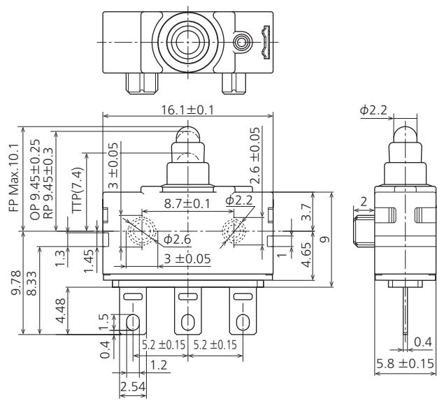
External dimensions
