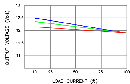
12V OUTPUT VOLTAGE VS. LOAD
