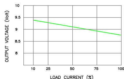
9V OUTPUT VOLTAGE VS. LOAD
