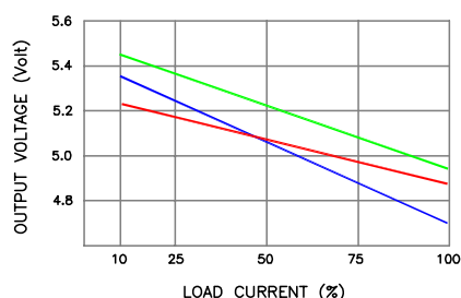
5V OUTPUT VOLTAGE VS. LOAD
