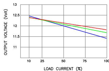
12V OUTPUT VOLTAGE VS. LOAD
