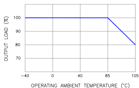
OUTPUT POWER DERATING
