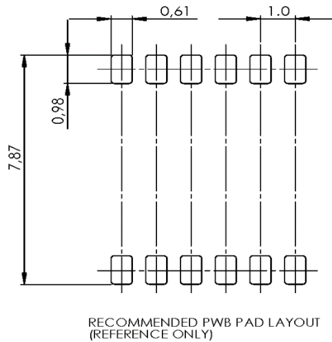
Figure 11 Recommended PWB pad layout for SCA3400-D01. All dimensions are in mm. The tolerances are according to ISO2768-f (see Table 9).
