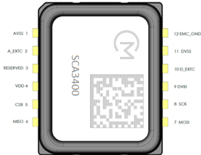
Figure 1 Pinout for SCA3400-D01.
