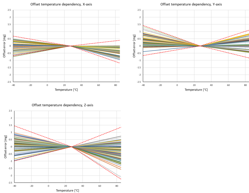
Figure 3 Accelerometer typical offset temperature behavior zeroed at +25°C. Dotted lines show the \pm 3\sigma variation of the population.
