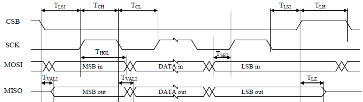
Figure 8 Timing diagram of SPI communication.
