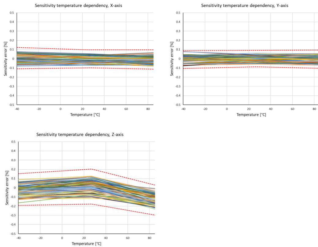
Figure 5 Accelerometer typical sensitivity temperature error in %. Dotted lines show the \pm 3\sigma variation of the population.
