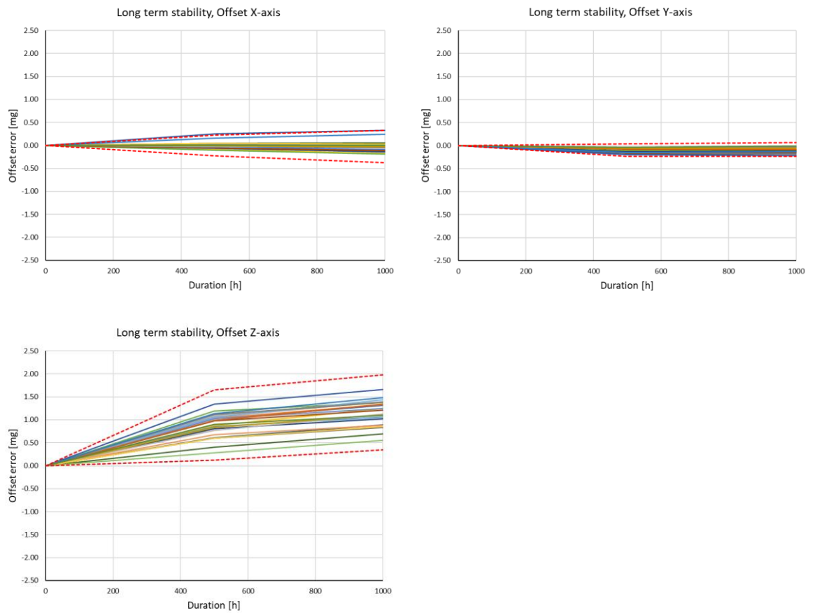
Figure 4 Example of long-term stability of accelerometer offset in 1000h HTOL test. Test condition = +85 °C, Vsupply = 3.6 V. Data measurement condition = +25°C. Dotted lines show the \pm 3\sigma variation of the population.
