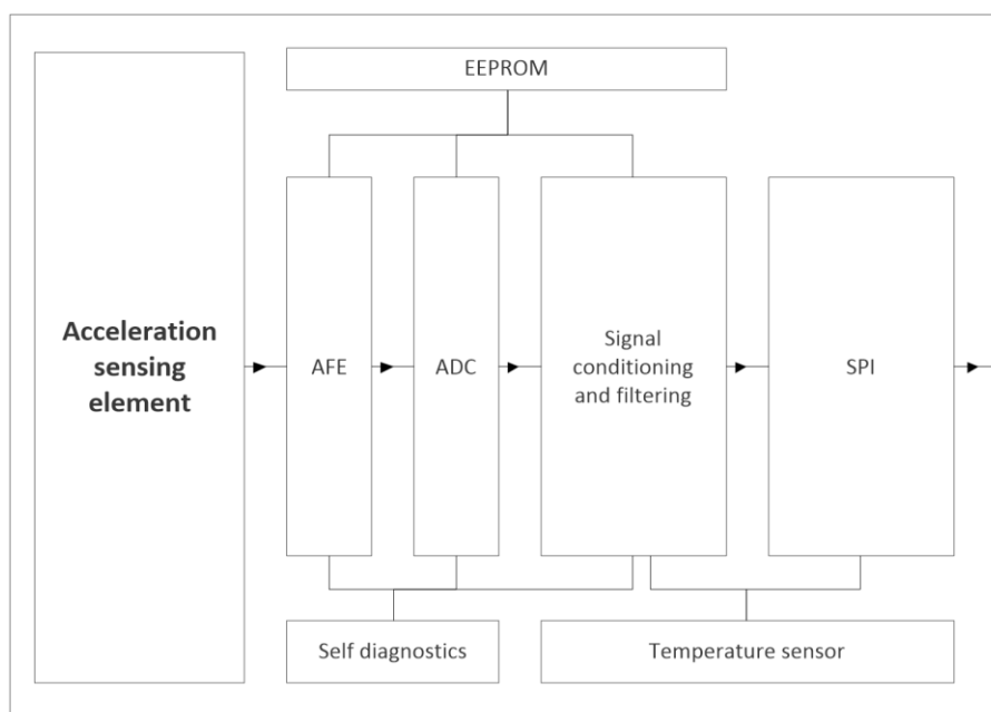
Figure 12 SCA3400-D01 component block diagram.
