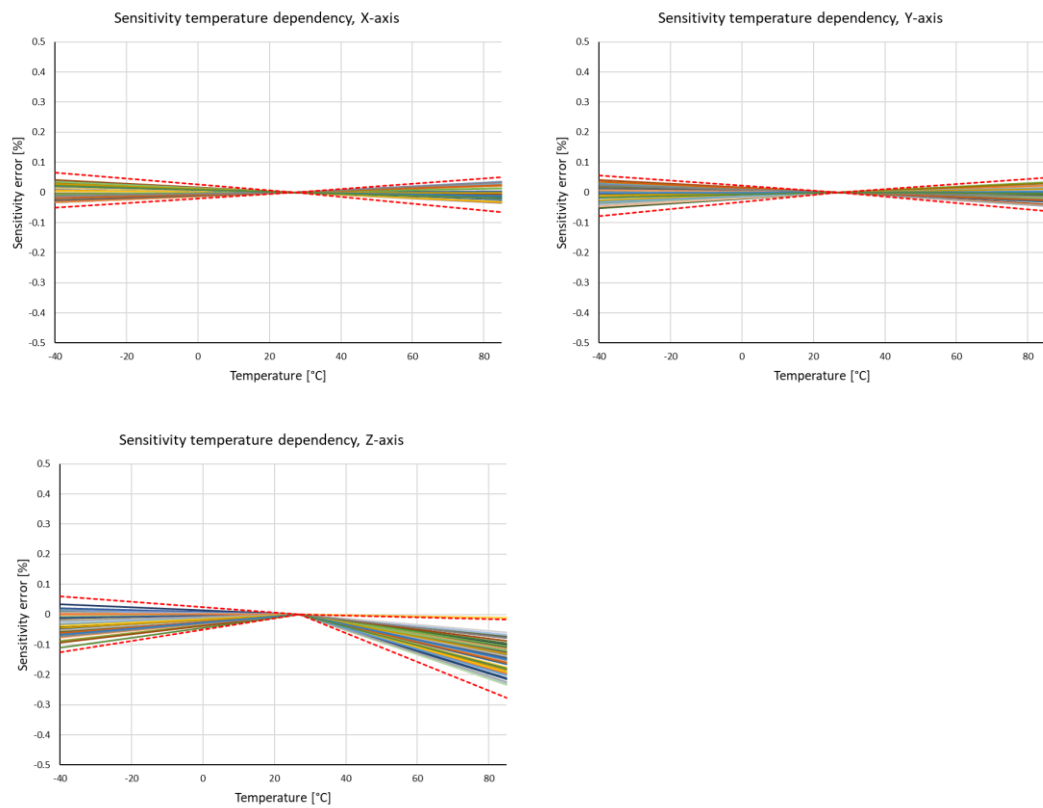
Figure 6 Accelerometer typical sensitivity temperature error in %, zeroed at +25°C. Dotted lines show the \pm 3\sigma variation of the population.
