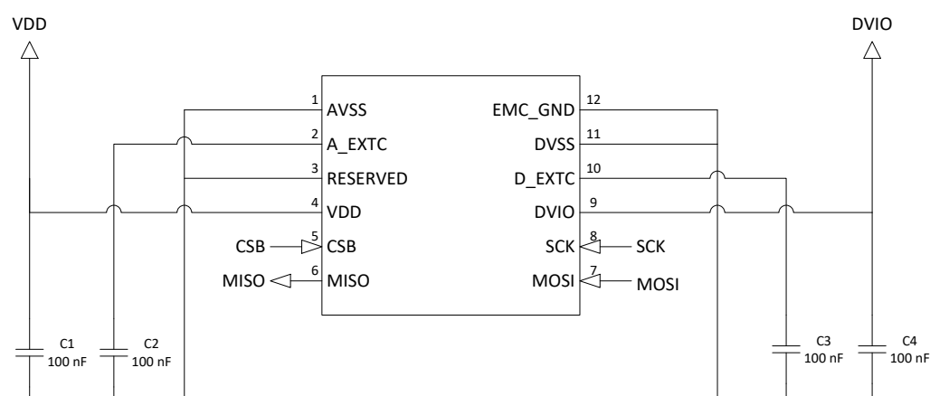
Figure 16 Application schematic.
