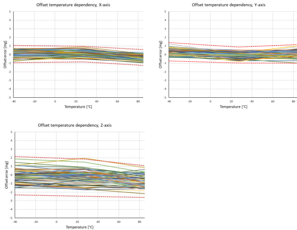
Figure 2 Accelerometer typical offset temperature behavior. Dotted lines show the \pm 3\sigma variation of the population.
