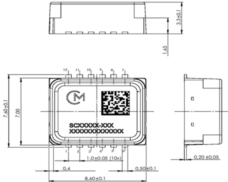
Figure 10 Package outline. The tolerances are according to ISO2768-f (see Table 9).
