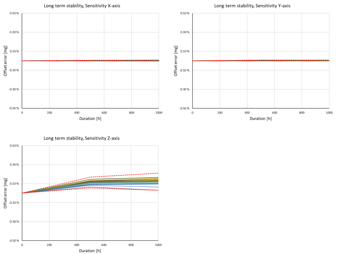
Figure 7 Example of long-term stability of accelerometer sensitivity in 1000h HTOL test. Test condition = +85 °C, Vsupply = 3.6 V. Data measurement condition = +25°C. Dotted lines show the \pm 3\sigma variation of the population.
