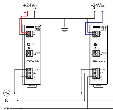
Fig. 31: Connection scheme for series operation with centre tap
