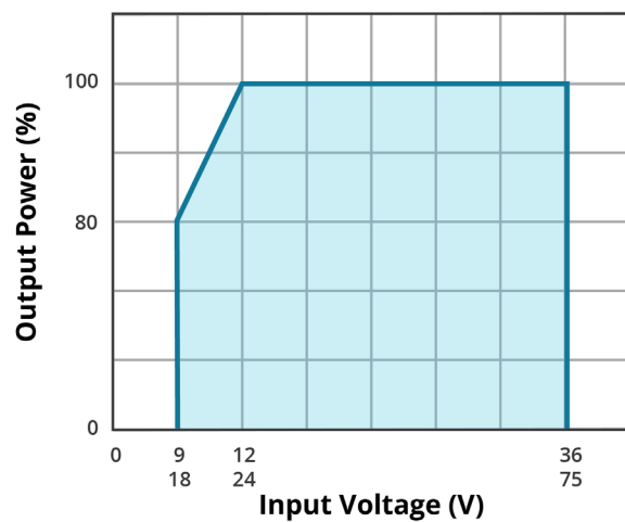
INPUT VOLTAGE DERATING CURVE (3.3, 5 & ±5 Vdc output models)
