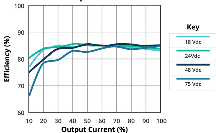
EFFICIENCY VS OUTPUT LOAD DRQ10-48-S5-S
