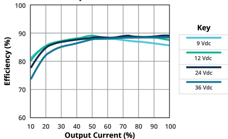
EFFICIENCY VS OUTPUT LOAD DRQ10-24-D15-S
