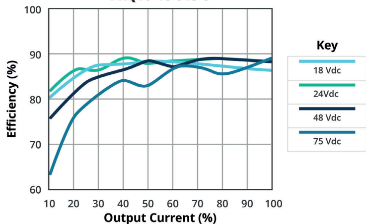
EFFICIENCY VS OUTPUT LOAD DRQ10-48-S15-S
