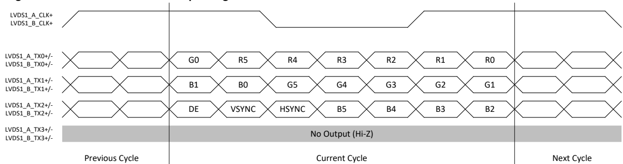
Figure 10: 18-bit Mode
