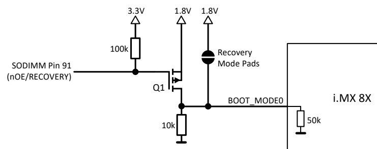
Figure 13: Recovery Mode Glue Logic
