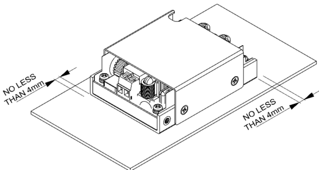
LFM200SXXXC installation diagram
