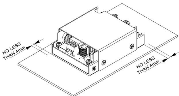
LFM200MXXXC installation diagram
