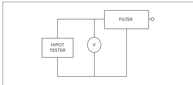
Figure 6. Typical Test Setup for Dielectric Withstand or Hi-Pot.
