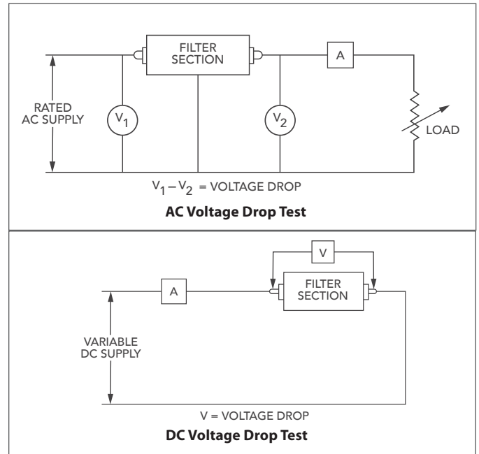
Figure 5. Typical Voltage Drop Test Configuration.
