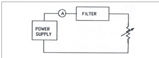
Figure 8. Temperature Rise Test Setup.
