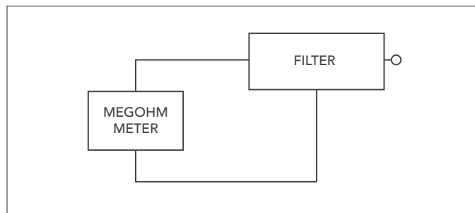
Figure 7. Setup for Insulation Resistance Test.
