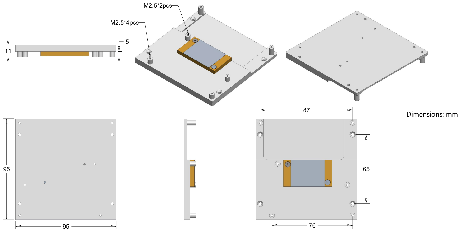
Figure 6 – Heatspreader: HTS
