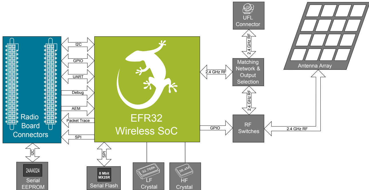
Figure 3.1. BRD4185A Block Diagram
