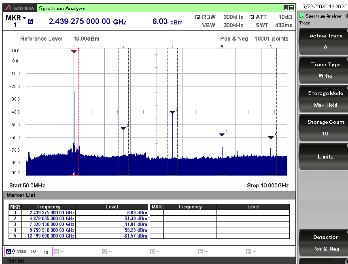
Figure 7.1. Typical Output Spectrum of the BRD4185A; PAVDD = 3.3 V
