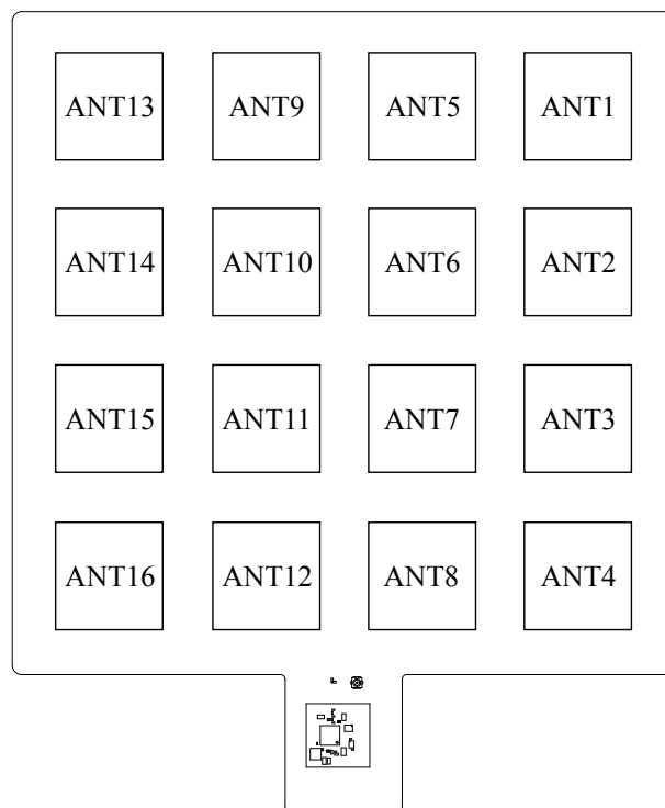
Figure 4.2. Antenna Selection
