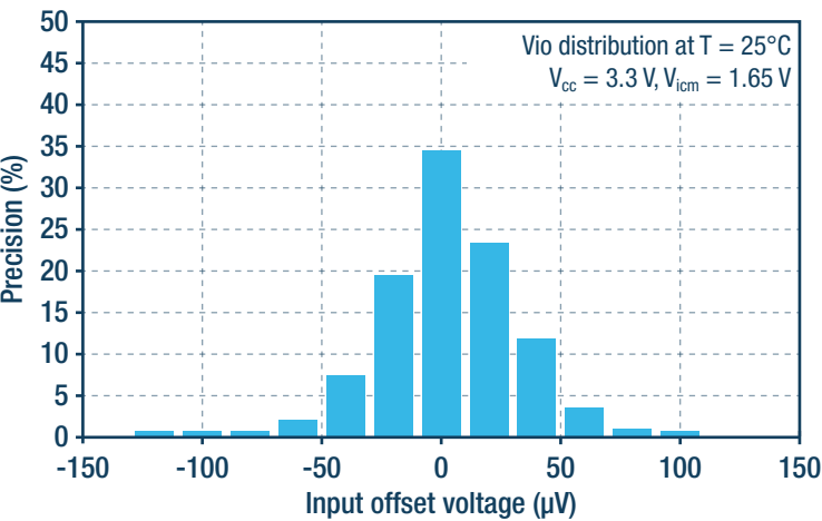
Input offset voltage distribution
