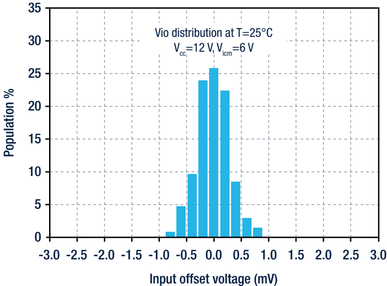
Input offset distribution
