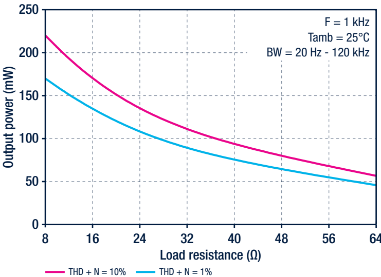
Output power vs. load resistance V_{CC} = 5\text{ V}
