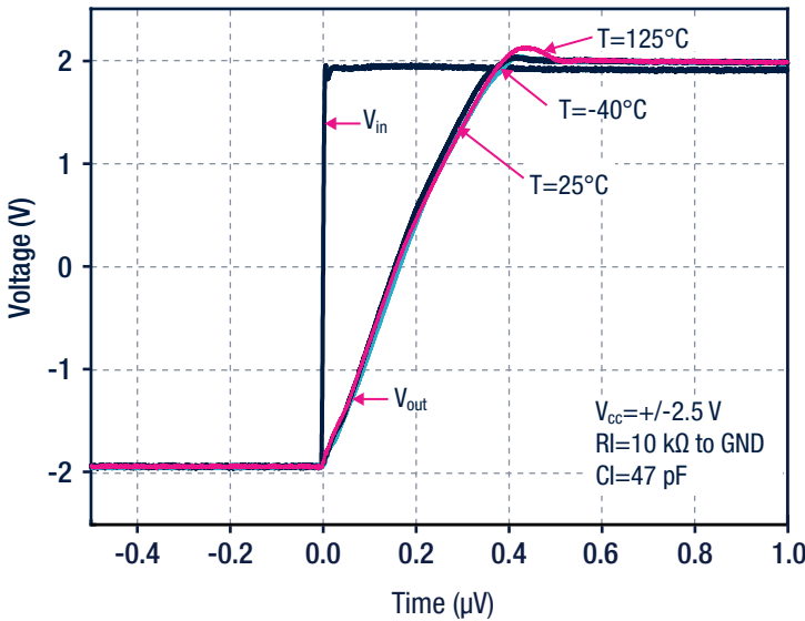
Positive slew rate at V CC = 5 V
