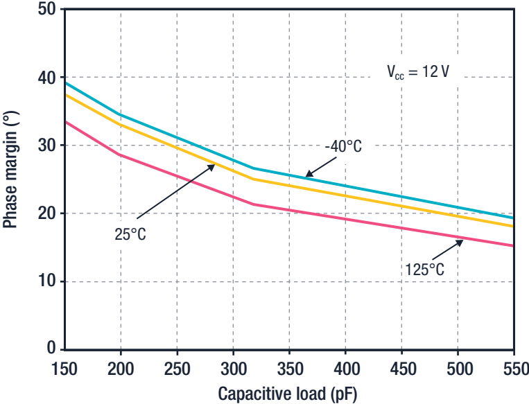
Phase margin vs. capacitive load
