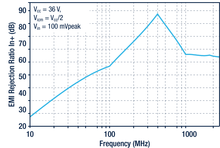
EMI rejection ratio V_{cc} = 36 V
