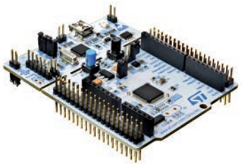
STM32 Nucleo-64 development board STM32F4 MCU
