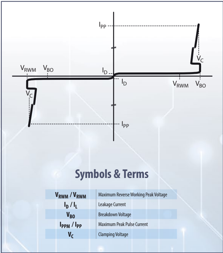
Typical TVS Diode V-I Characteristic (Bidirectional)
