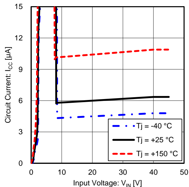
Figure 52. Circuit Current vs Input Voltage - Enlarged view ( I_{OUT} = 50\text{ mA} )
