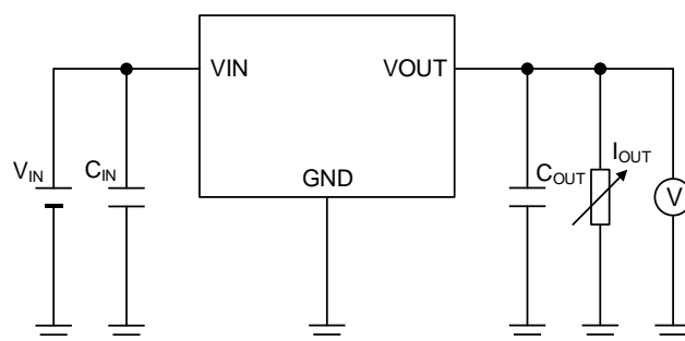
Measurement Setup for Figure 11, 12, 25, 26, Figure 40, 41, 55, 56
