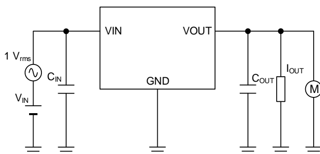
Measurement Setup for Figure 14, 29, 44, 59
