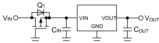
Figure 68. Protection against Reverse Polarity 2
