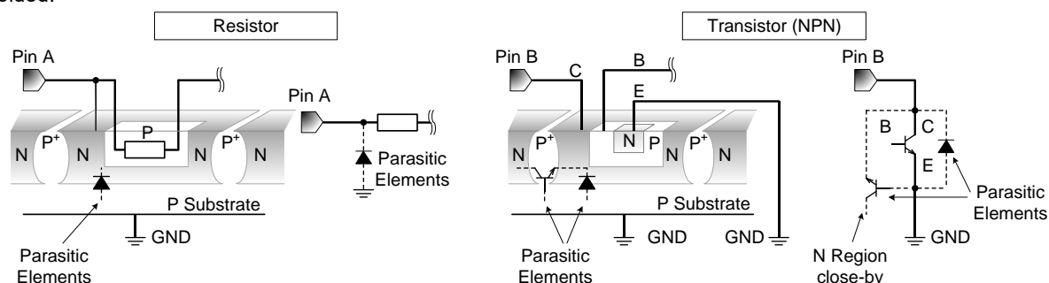
Figure 72. Example of Monolithic IC Structure
