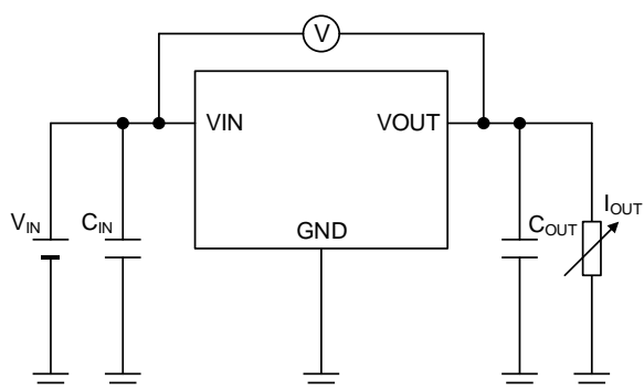
Measurement Setup for Figure 27, 42, 57
