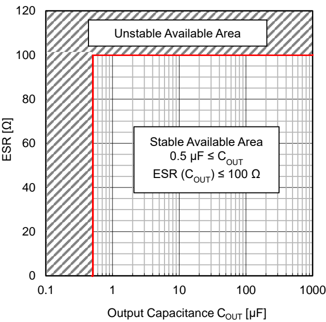
Figure 60. Output Capacitance C_{OUT} , ESR Stable Available Area
