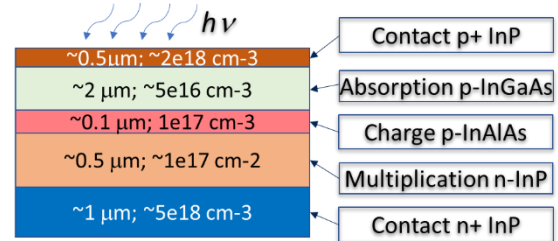
Figure 6. Ge-Si APDs with Separate Absorption and Charge Multiplication regions
