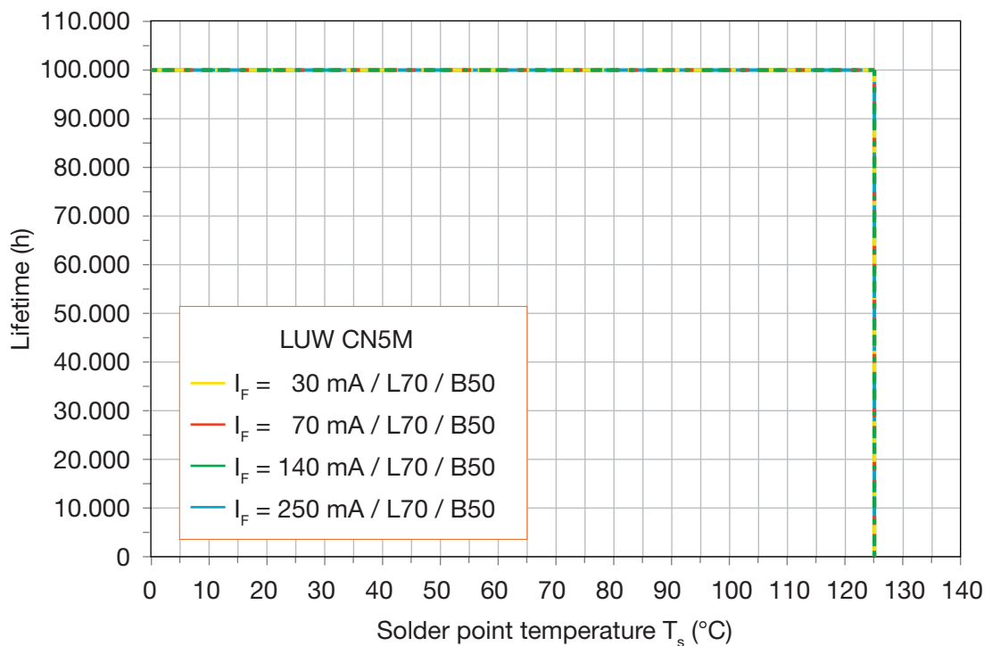
Figure 5: Lifetimes [1] of the OSOLON ® types (SX) with ThinGaN technology with respect to T_S
