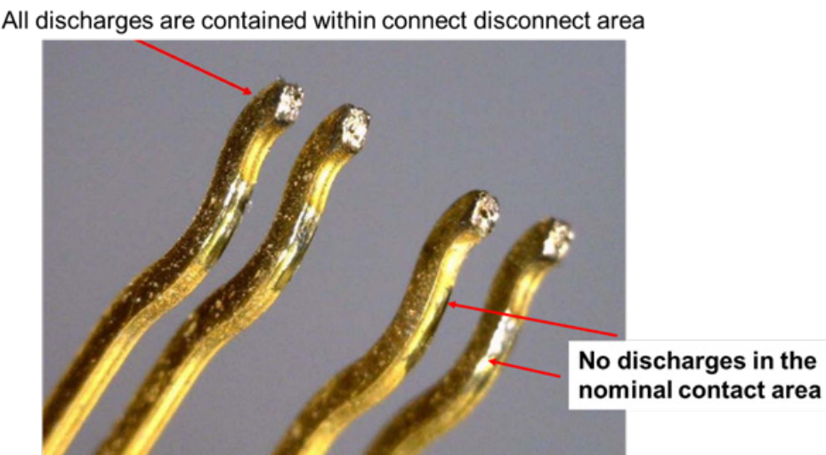
Figure 15. RJ point five electrical discharge effect
