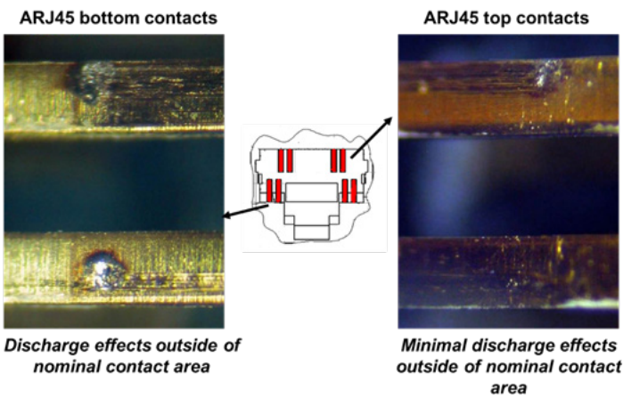
Figure 11. ARJ45 electrical discharge effects
