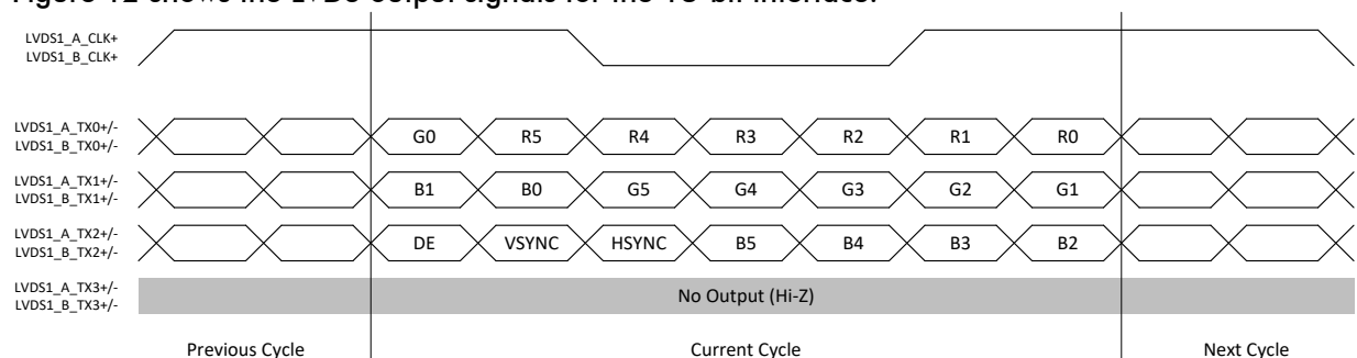
Figure 12: 18-bit Mode
