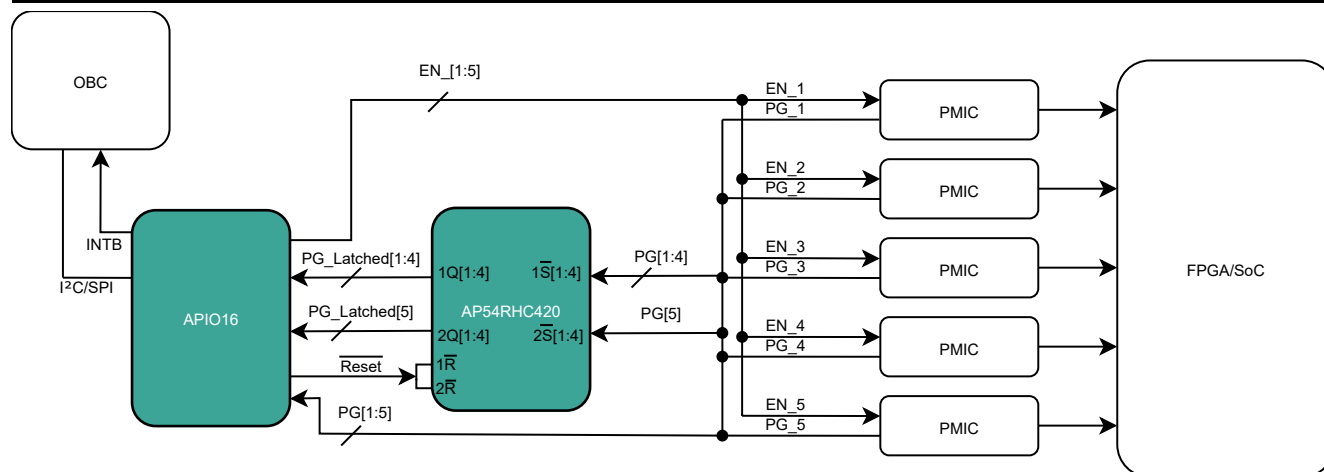
Figure 10: Latched and Unlatched PMIC Fault Detection
