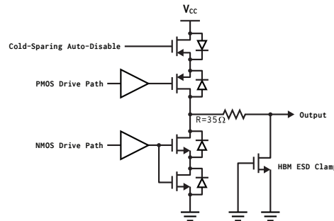
Figure 6: Output Pin Structure
