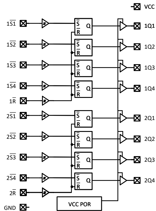
Figure 1: AP54RHC420 Logic Diagram
