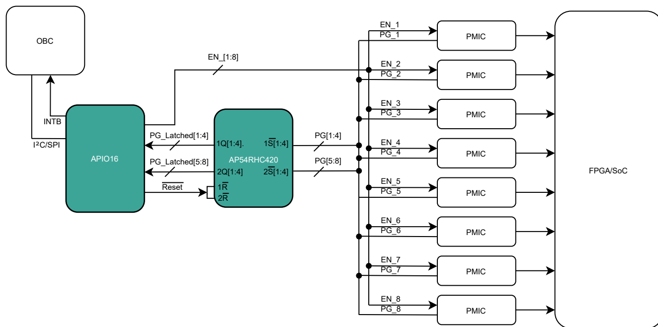
Figure 11: Latched PMIC Fault Detection
