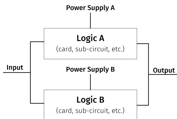
Figure 9: Two-Path Cold-Sparing Configuration
