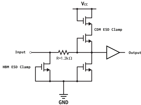
Figure 5: Input Pin Structure
