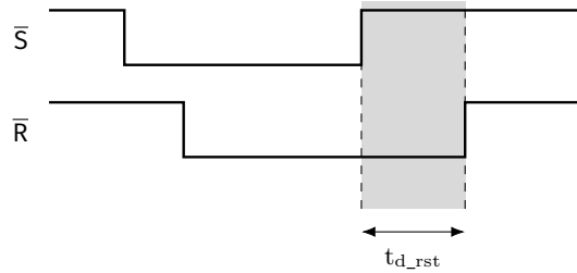
Figure 7: Overlapping pulses with long set
