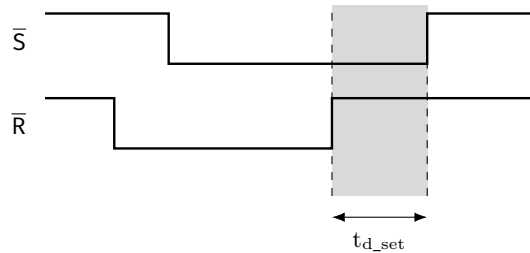
Figure 8: Overlapping pulses with long reset
