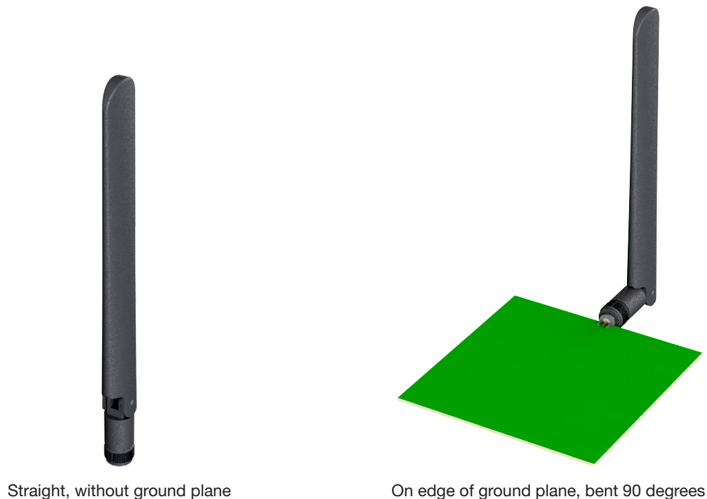
Figure 2. ANT-W63WS4-ccc Test Orientation
