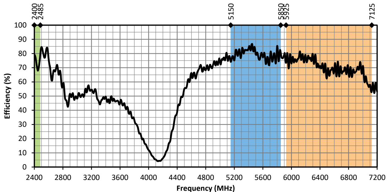
Figure 8. ANT-W63WS4-ccc Antenna Efficiency, Straight
