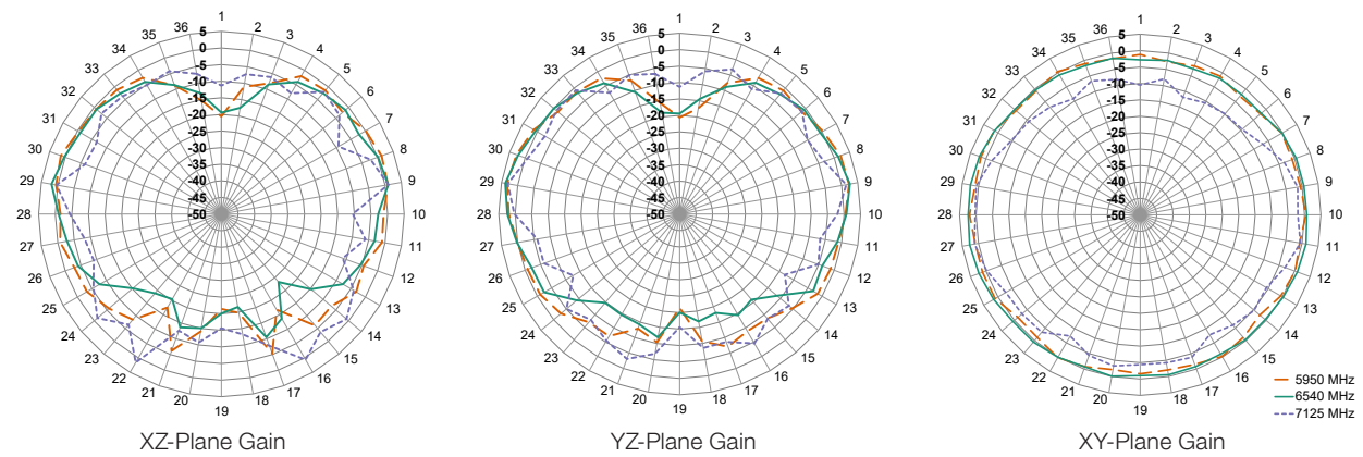
Figure 9. Radiation Patterns for ANT-W63WS4-ccc, Straight
