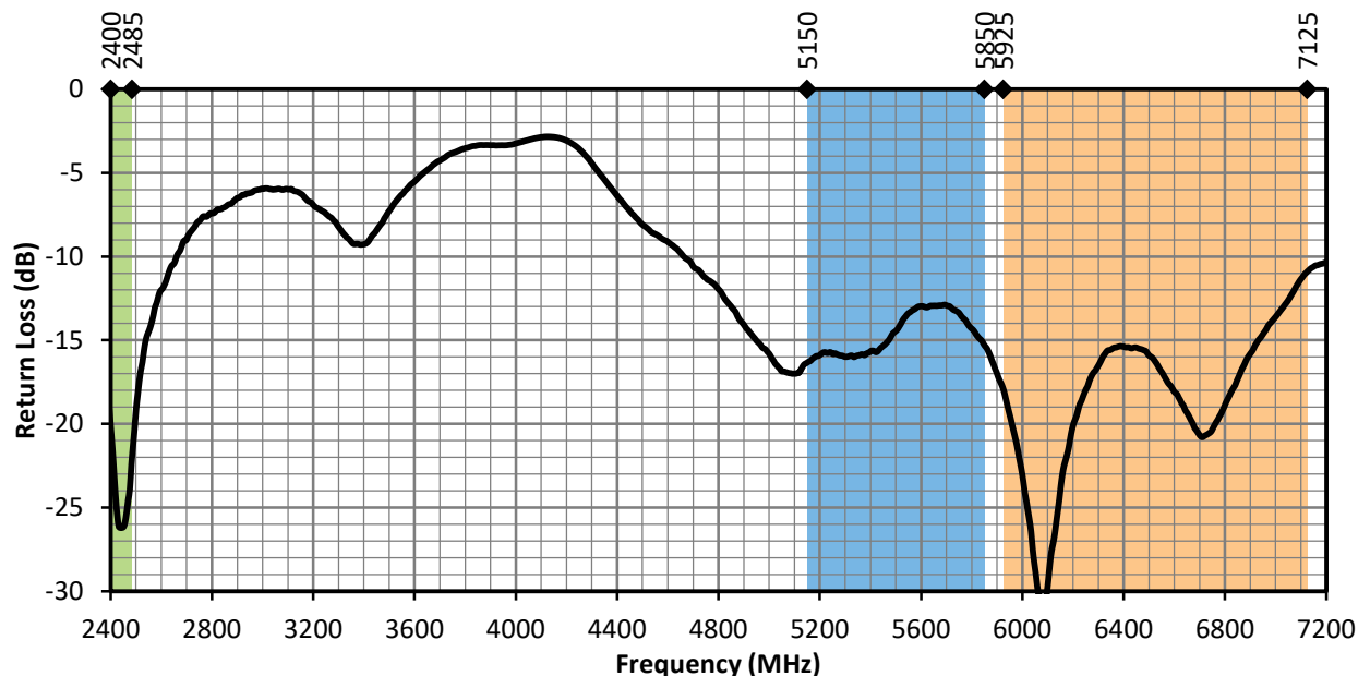
Figure 5. ANT-W63WS4-ccc Return Loss, Straight
