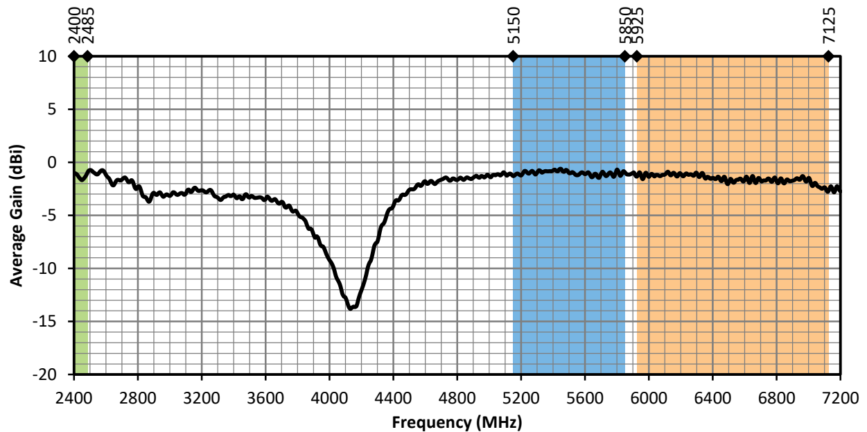
Figure 7. ANT-W63WS4-ccc Antenna Average Gain, Straight
