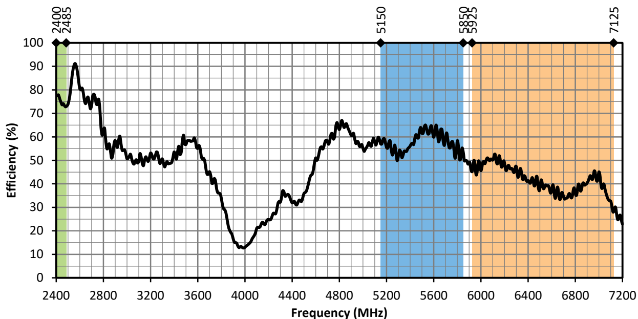
Figure 15. ANT-W63WS4-ccc Antenna Efficiency, Edge-Bent
