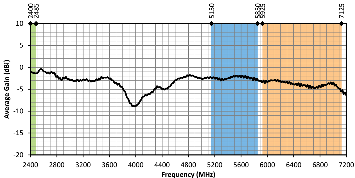
Figure 14. ANT-W63WS4-ccc Antenna Average Gain, Edge-Bent
