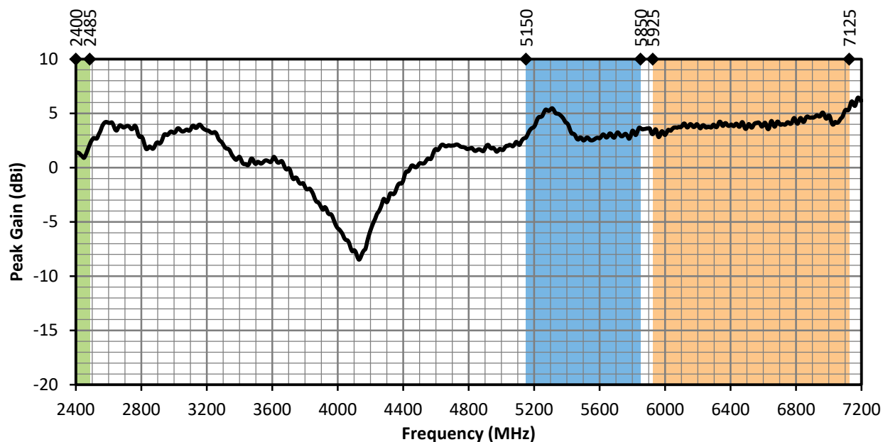
Figure 6. ANT-W63WS4-ccc Peak Gain, Straight
