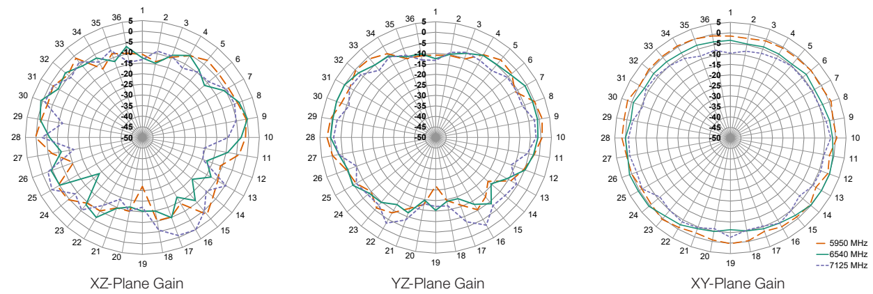
Figure 16. Radiation Patterns for ANT-W63WS4-ccc, Edge-Bent
