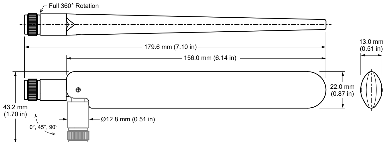
Figure 1. ANT-W63WS4-ccc Antenna Dimensions
