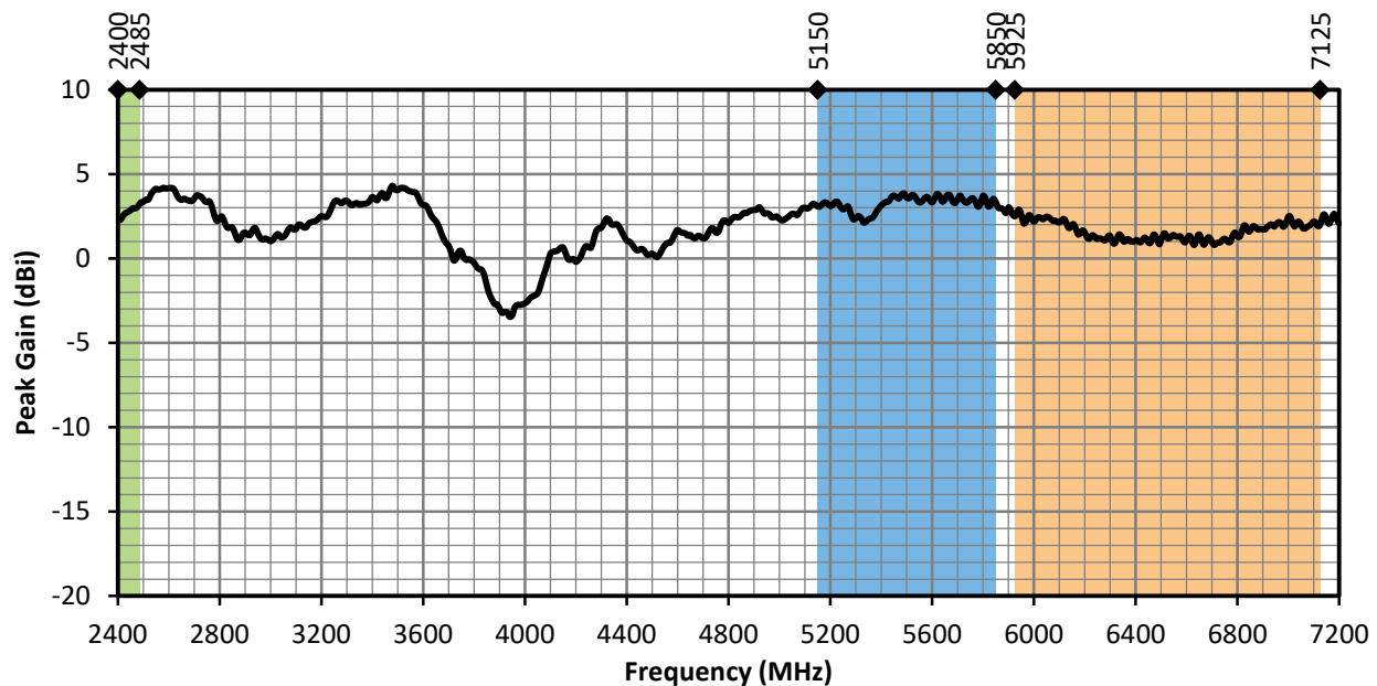
Figure 13. ANT-W63WS4-ccc Peak Gain, Edge-Bent
