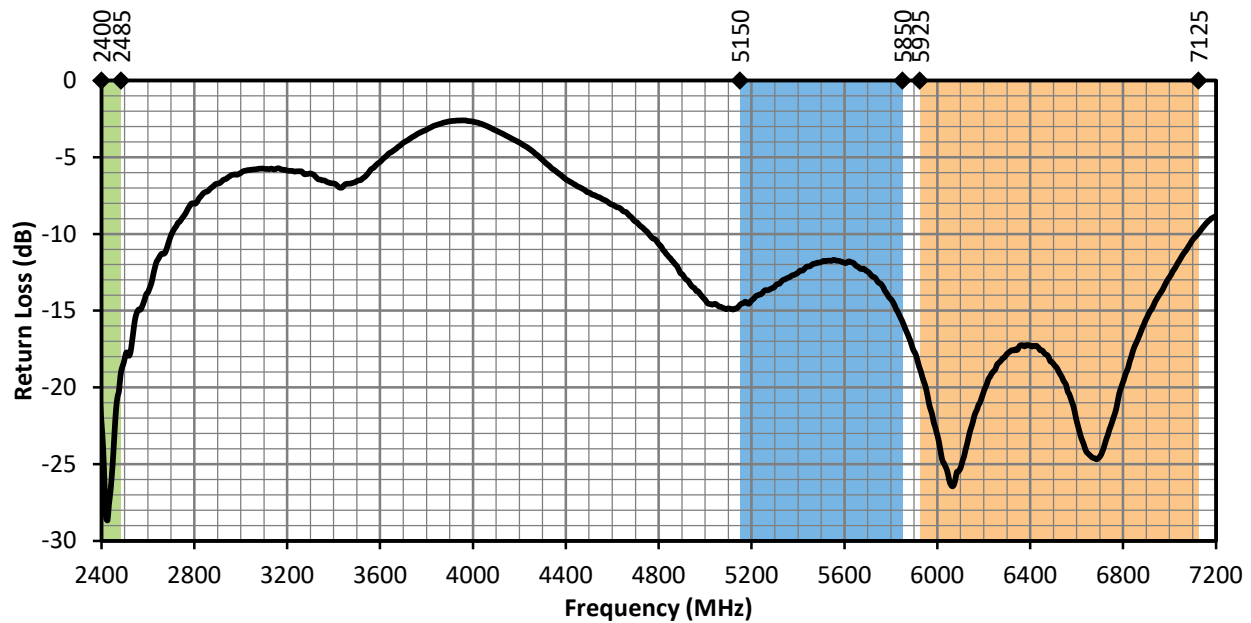
Figure 12. ANT-W63WS4-ccc Return Loss, Edge-Bent
