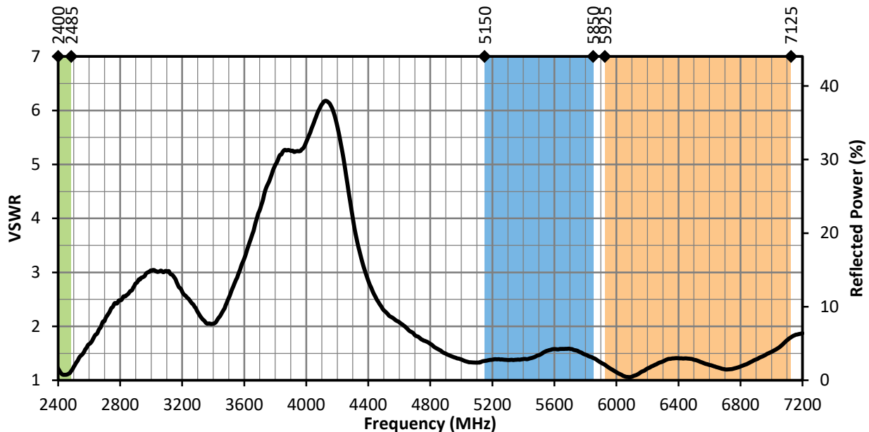
Figure 4. ANT-W63WS4-ccc VSWR, Straight
