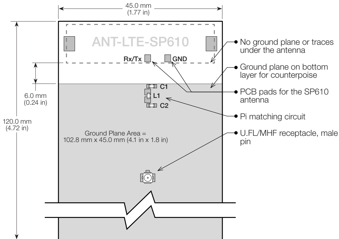
Figure 9. SP610 Recommended Layout.
