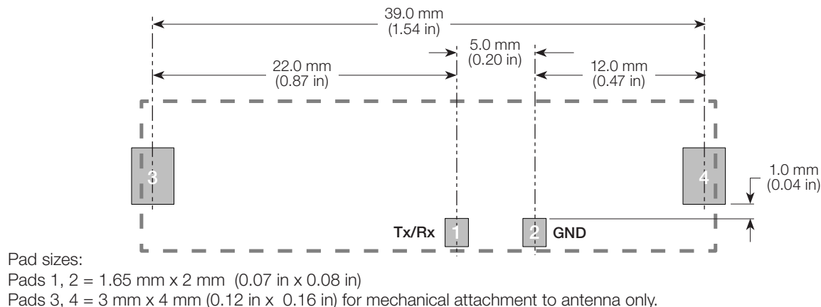
Figure 11. SP610 Placement on PCB
