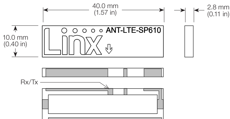
Figure 6. SP610 Dimensions
