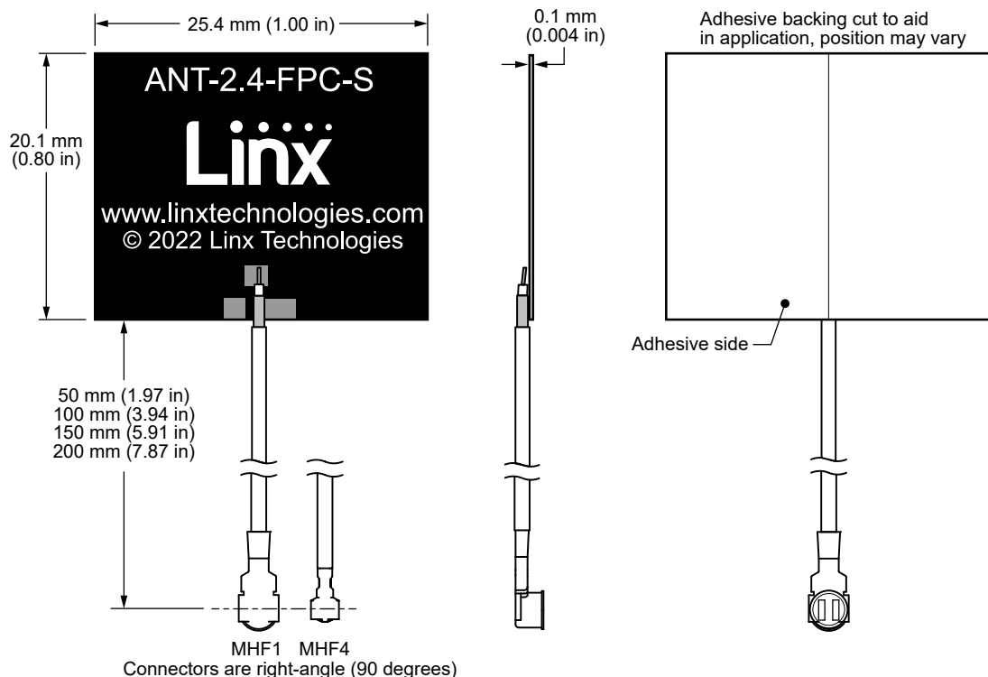
Figure 1. ANT-2.4-FPC-SH Series Antenna Dimensions
