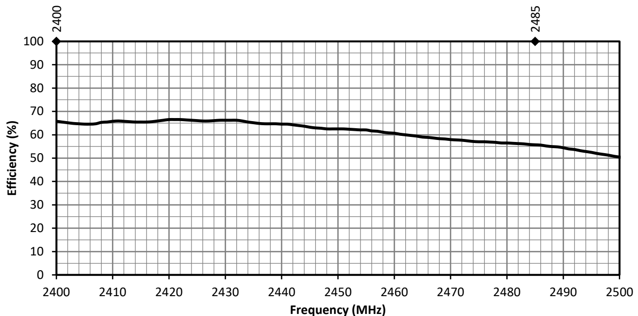
Figure 6. ANT-2.4-FPC-SF Antenna Radiation Efficiency
