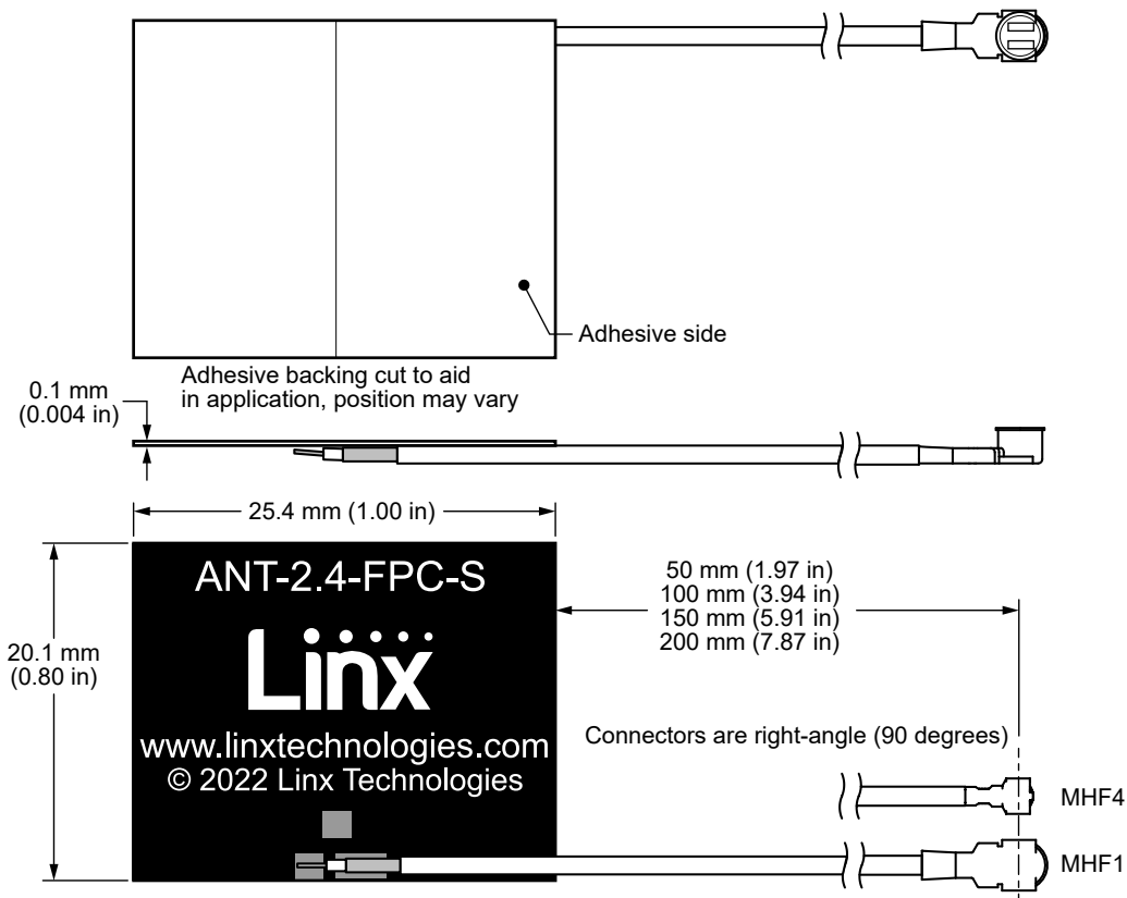
Figure 1. ANT-2.4-FPC-SF Series Antenna Dimensions
