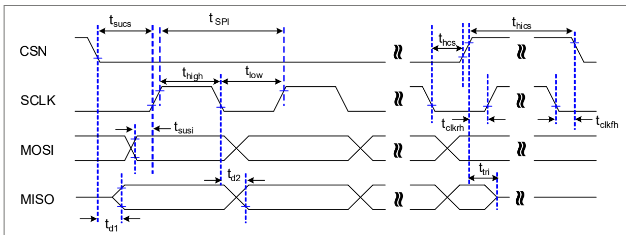
Figure 23: SPI timing diagram
