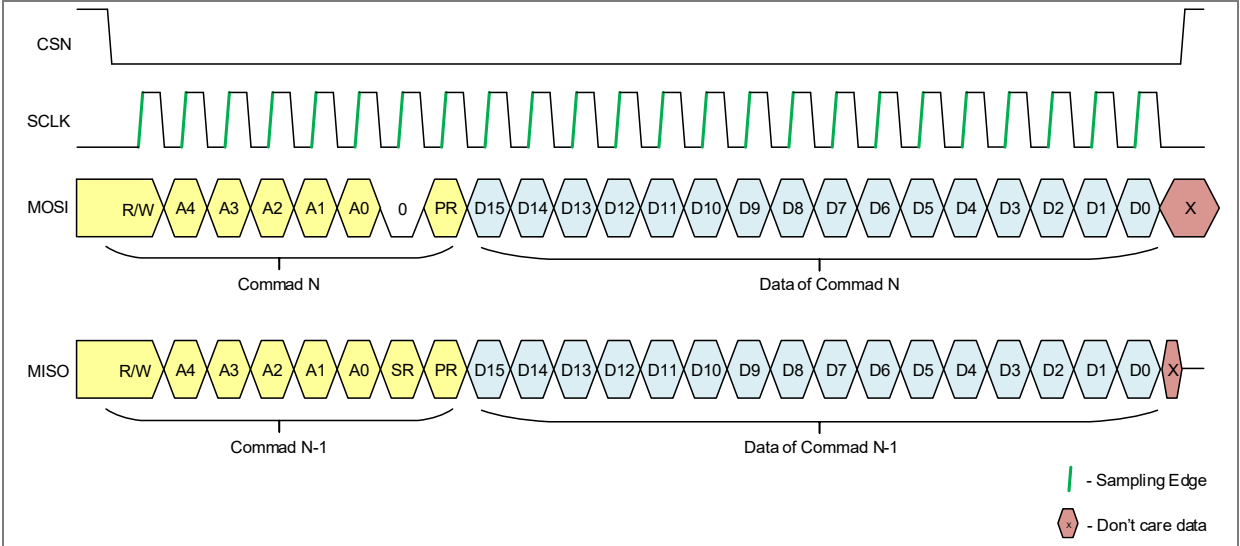
Figure 18: SPI transaction detailed diagram
