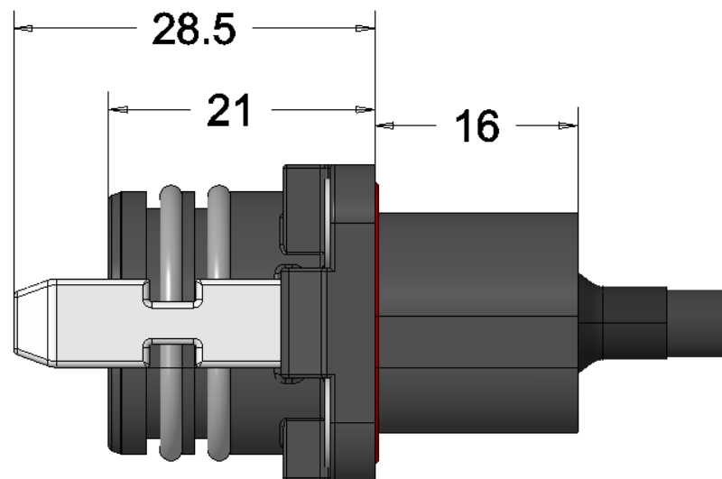
Battery side connector
