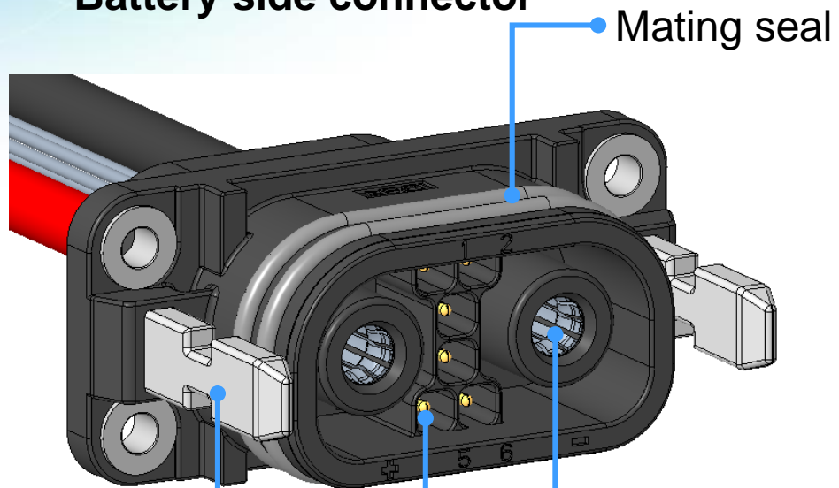
Battery side connector
