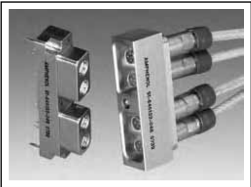
Compliant Pin Quadrax Board Level Connector
