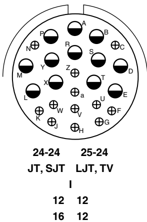
front face of pin inserts illustrated
