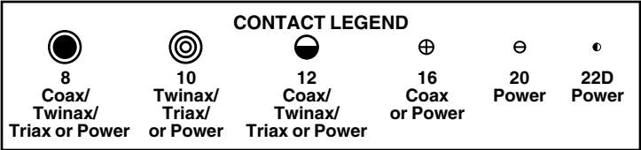
front face of pin inserts illustrated
