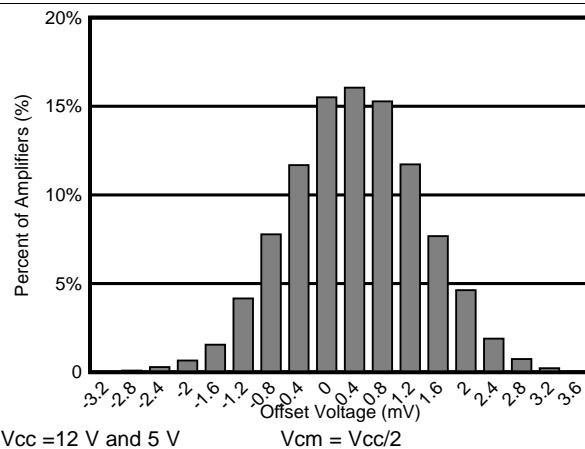
Figure 20. Offset Voltage Production Distribution
