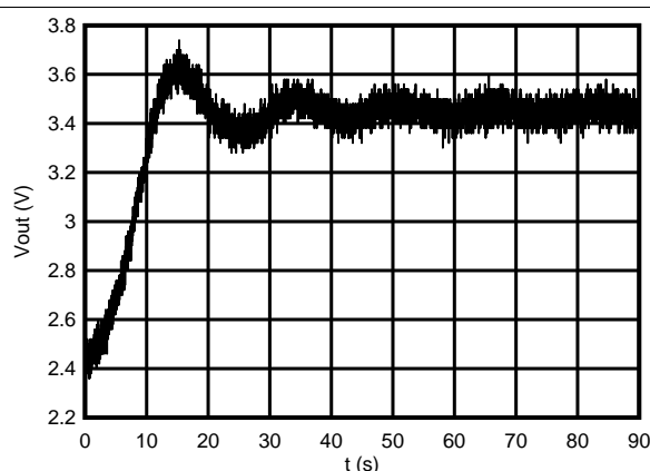
Figure 27. Output Pulse Response ( C_L = 2.2 \mu\text{F} and R_L = 100 \Omega )
