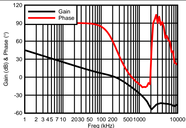
Figure 8. Gain and Phase ( C_L = 200\text{ nF} and R_L = 50\ \Omega )
