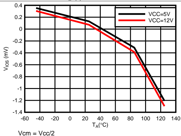
Figure 19. Input Offset vs. Temperature
