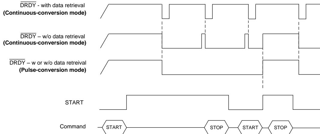
Figure 36. \overline{\text{DRDY}} Operation
