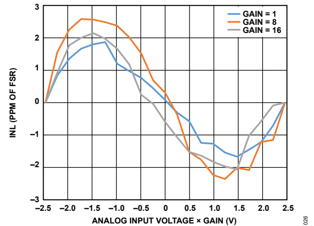
Figure 26. INL vs. Differential Input Signal (Analog Input × Gain), ODR = 50 SPS, External 2.5 V Reference
