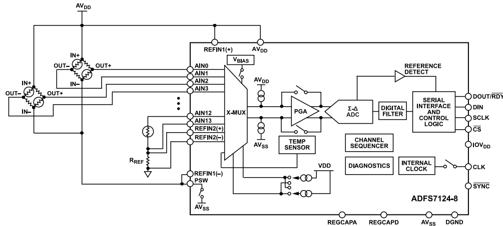
Figure 128. Flowmeter Application
