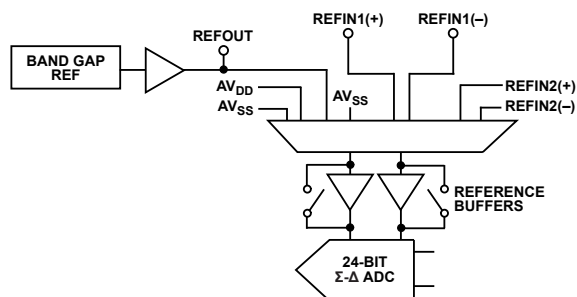
Figure 75. Reference Connections
