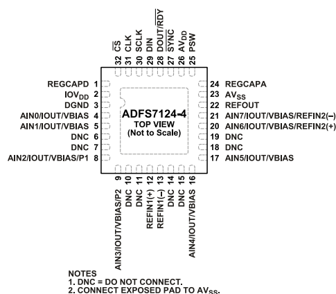
Figure 9. 32-Lead LFCSP Pin Configuration
