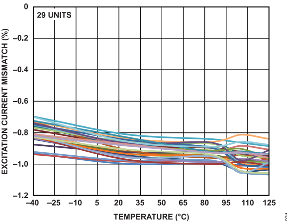
Figure 33. Excitation Current Drift Matching (500 µA)
