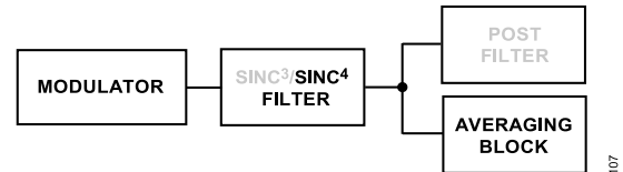
Figure 97. Fast Settling Mode, Sinc 4 + Sinc 1 Filter
