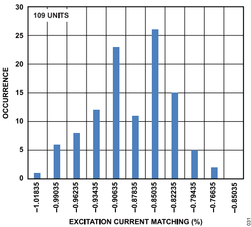
Figure 31. IOUTx Current Initial Matching Histogram (500 µA)
