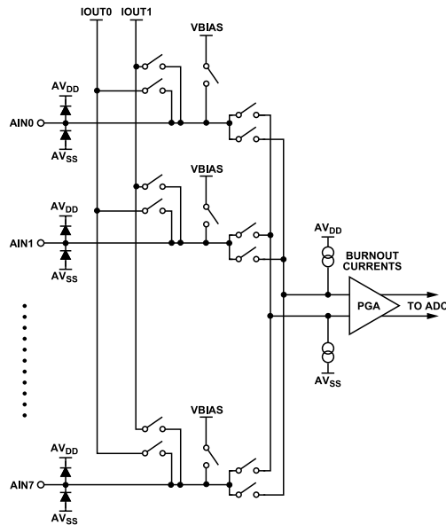
Figure 77. Excitation Current and Bias Voltage Connections
