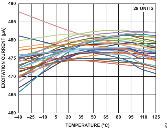
Figure 32. Excitation Current Drift (500 µA)
