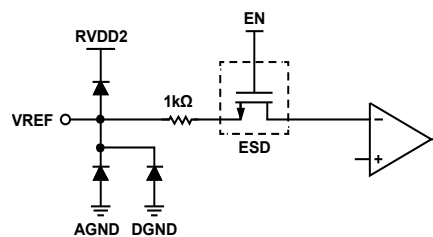
Figure 86. VREF
