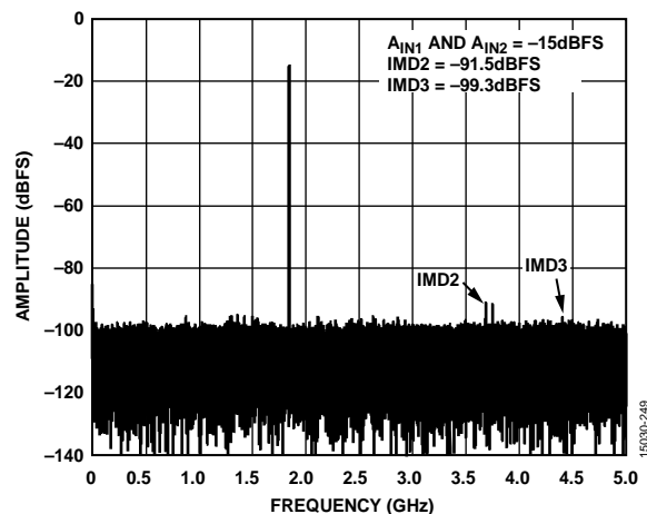
Figure 62. Two-Tone FFT, f_{IN1} = 1841.5\text{ MHz} , f_{IN2} = 1846.5\text{ MHz} , A_{IN1} and A_{IN2} = -15\text{ dBFS} , 10 GSFS
