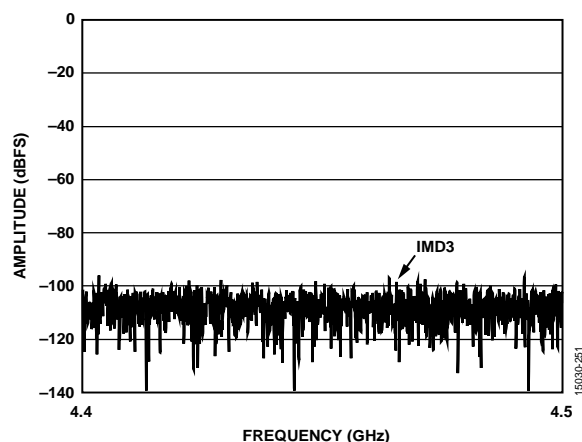
Figure 64. Two-Tone FFT, IMD3 Zoom In, f_{IN1} = 1841.5\text{ MHz} , f_{IN2} = 1846.5\text{ MHz} , A_{IN1} and A_{IN2} = -15\text{ dBFS} (see Figure 62), 10 GSFS
