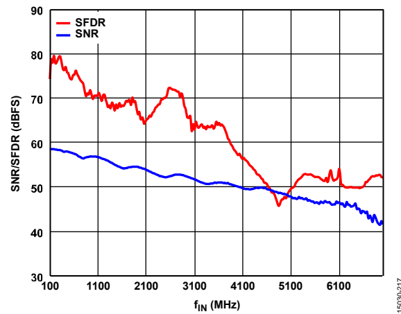
Figure 19. SNR/SFDR vs. f_{IN} , A_{IN} = -1 dBFS, 6 GSPS
