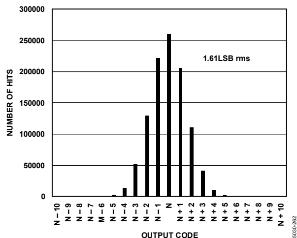
Figure 33. Input Referred Noise Histogram
