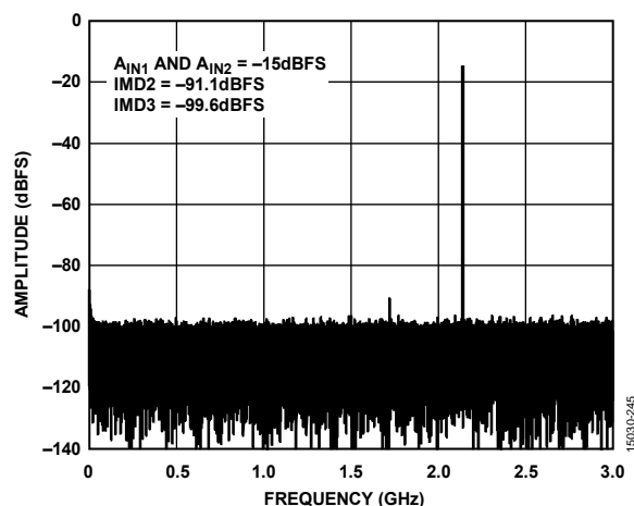
Figure 30. Two-Tone FFT, f_{IN1} = 2137.5 MHz, f_{IN2} = 2142.5 MHz, A_{IN1} and A_{IN2} = -15 dBFS, 6 GSPS
