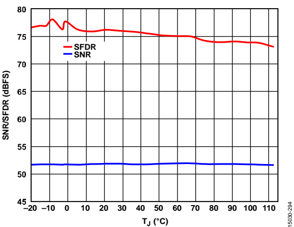
Figure 37. SNR/SFDR vs. T_J , f_{IN} = 2600 MHz, 6 GSPS
