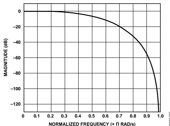
Figure 103. HB5 Filter Response
