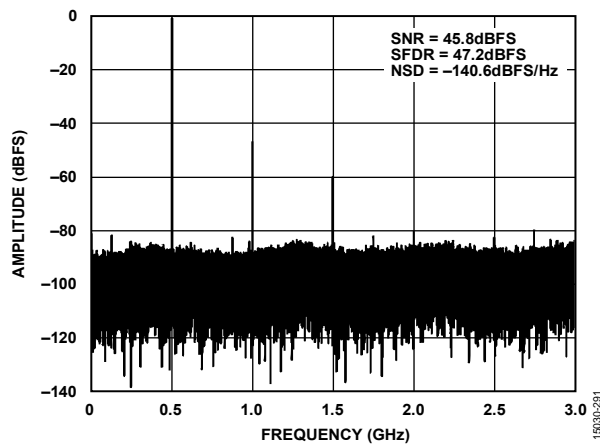
Figure 13. Single-Tone FFT with f_{IN} = 6.5 GHz, 6 GSPS
