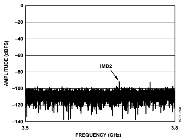
Figure 63. Two-Tone FFT, IMD2 Zoom In, f_{IN1} = 1841.5\text{ MHz} , f_{IN2} = 1846.5\text{ MHz} , A_{IN1} and A_{IN2} = -15\text{ dBFS} (see Figure 62), 10 GSFS
