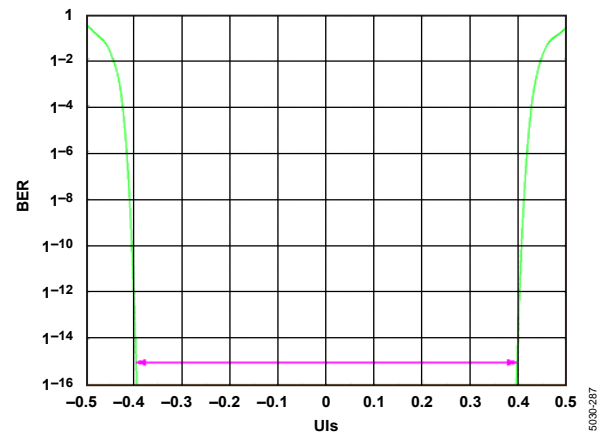
Figure 121. Digital Outputs Bathtub Curve, External 100 \Omega Terminations at 16 Gbps
