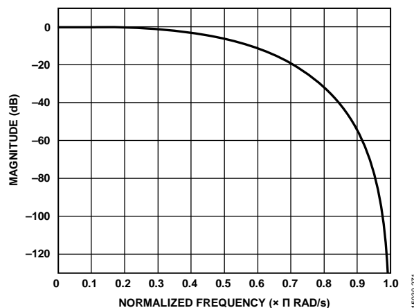
Figure 102. HB6 Filter Response
