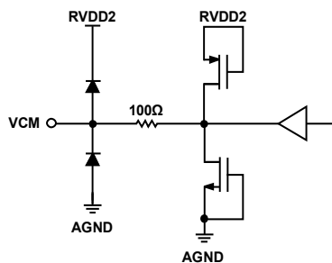
Figure 82. VCM
