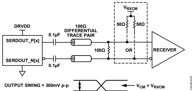
Figure 118. AC-Coupled Digital Output Termination Example
