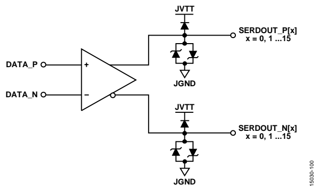
Figure 76. Digital Outputs
