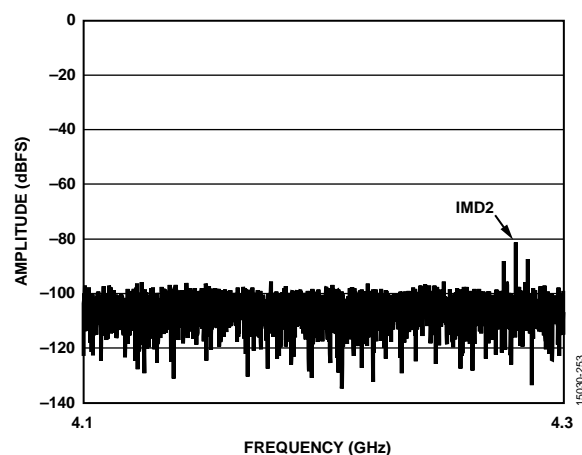
Figure 66. Two-Tone FFT, IMD2 Zoom In, f_{IN1} = 2137.5\text{ MHz} , f_{IN2} = 2142.5\text{ MHz} , A_{IN1} and A_{IN2} = -7\text{ dBFS} (see Figure 65), 10 GSFS
