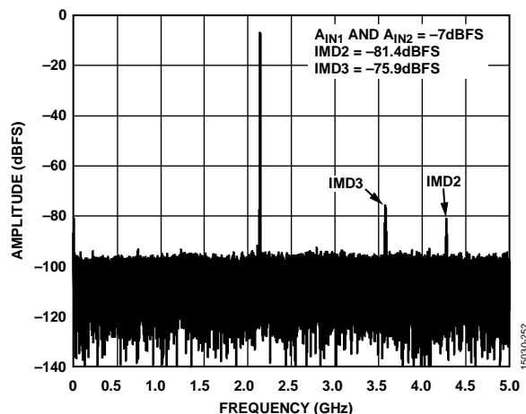
Figure 65. Two-Tone FFT, f_{IN1} = 2137.5\text{ MHz} , f_{IN2} = 2142.5\text{ MHz} , A_{IN1} and A_{IN2} = -7\text{ dBFS} , 10 GSFS
