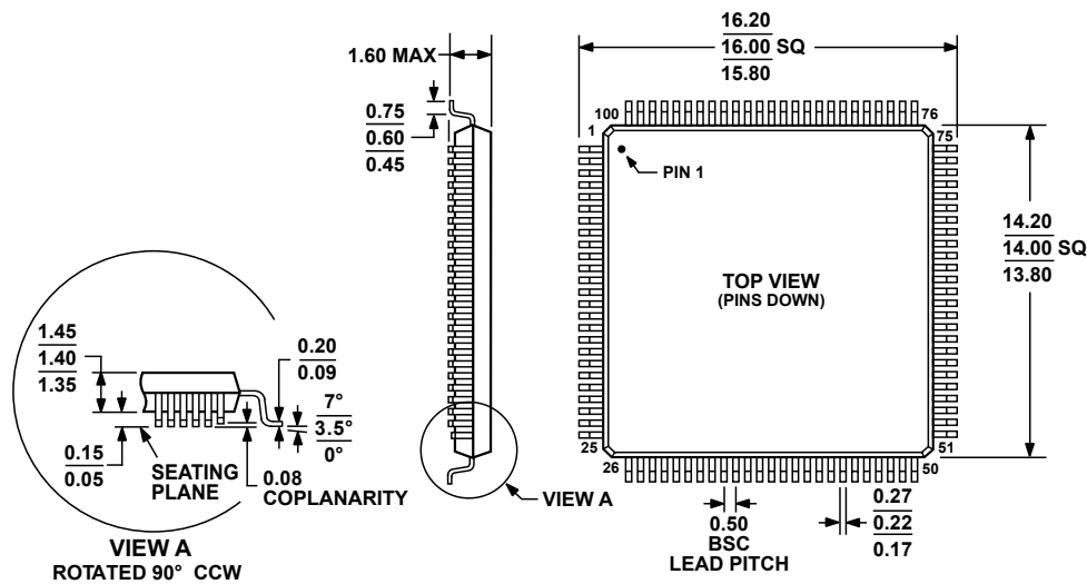
Figure 8. 100-Lead Low Profile Quad Flat Package [LQFP] (ST-100-1) Dimensions shown in millimeters
