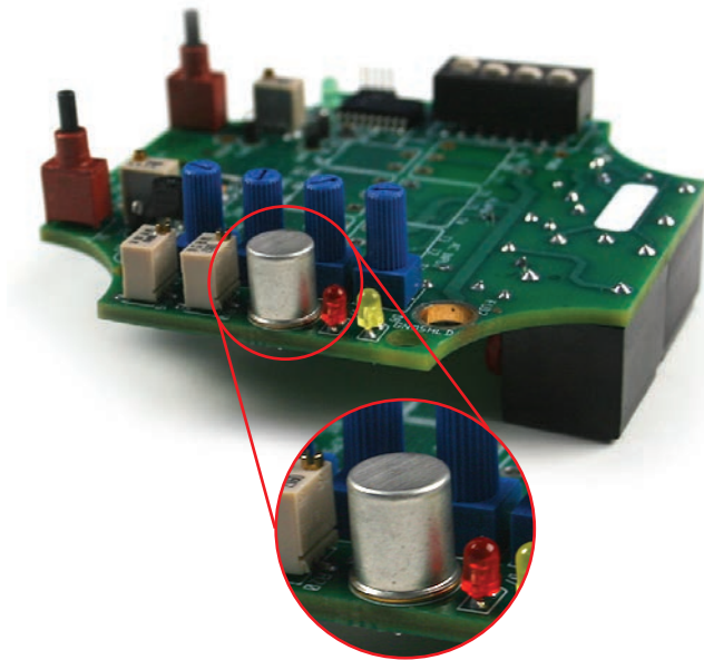
Example of a T0-5 accelerometer mounted on a circuit board
