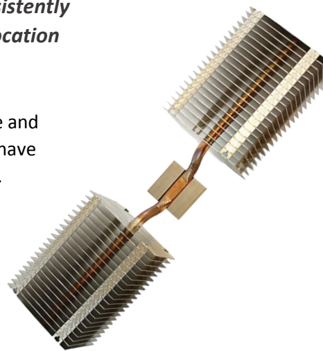
Above: Example of a heat pipe being used with the heat source at the center and the evaporators at either end.
