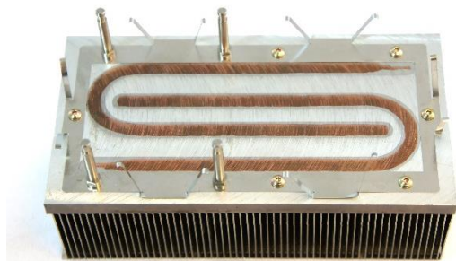
Above: Embedded heat pipes to enable a much smaller heat sink.
