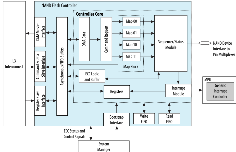
The following figure shows integration of the NAND flash controller in the HPS.
