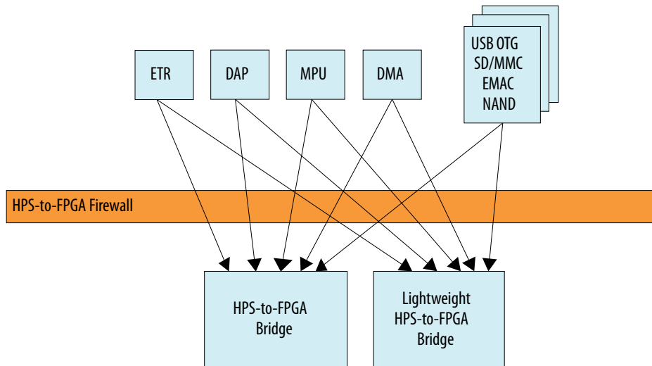
Figure 32. HPS-to-FPGA Bridge Connections
