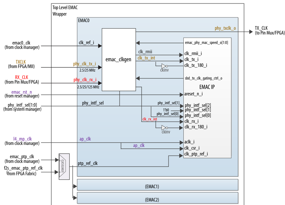
Figure 102. emac_clkgen Module
