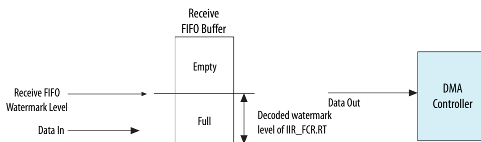
Figure 150. Receive FIFO Buffer
