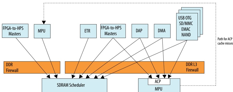
Figure 33. SDRAM Connections
