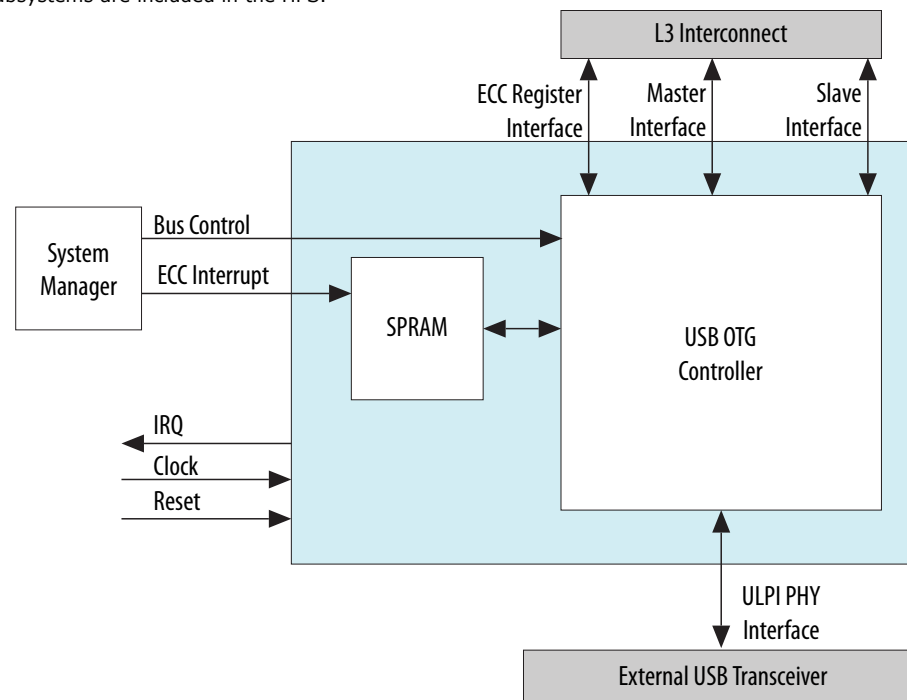
Figure 104. USB OTG Controller System Integration
