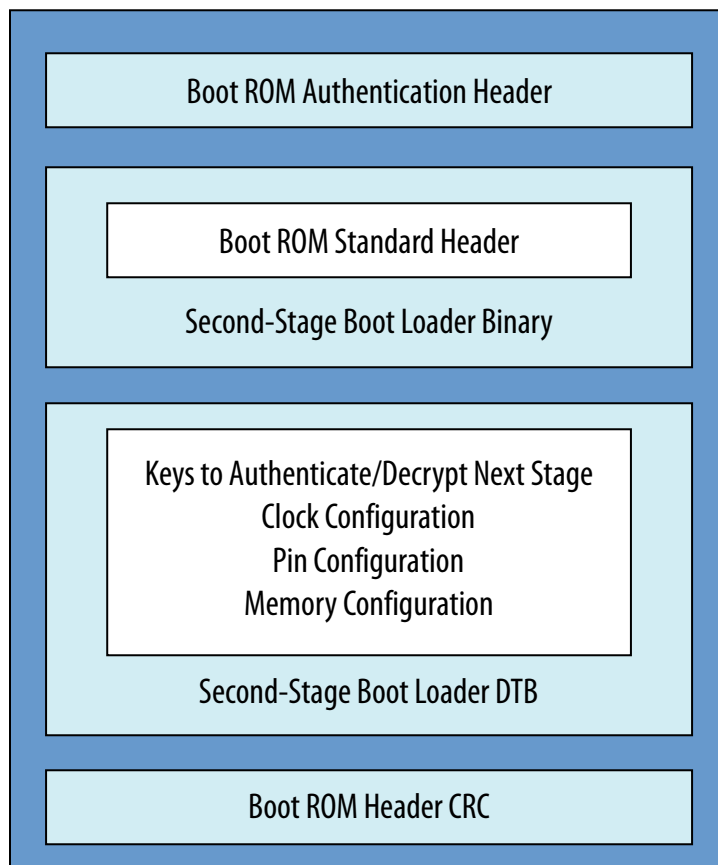
Figure 171. High-Level Diagram of Second-Stage Boot Loader Image
