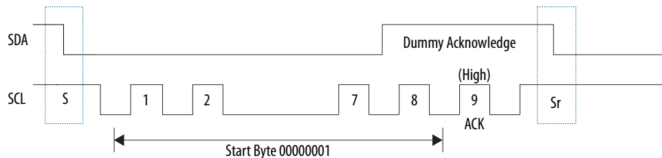
Figure 134. START BYTE Transfer †
