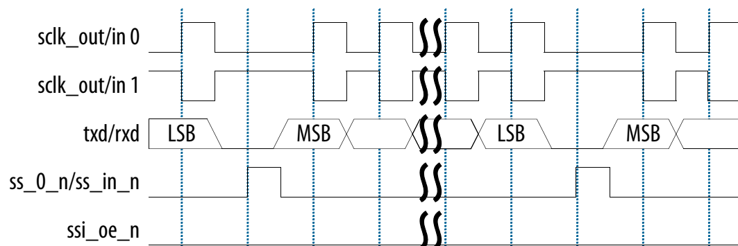
Figure 114. Serial Format Continuous Transfers ( SCPH = 0 and SCPOL = 0 )
