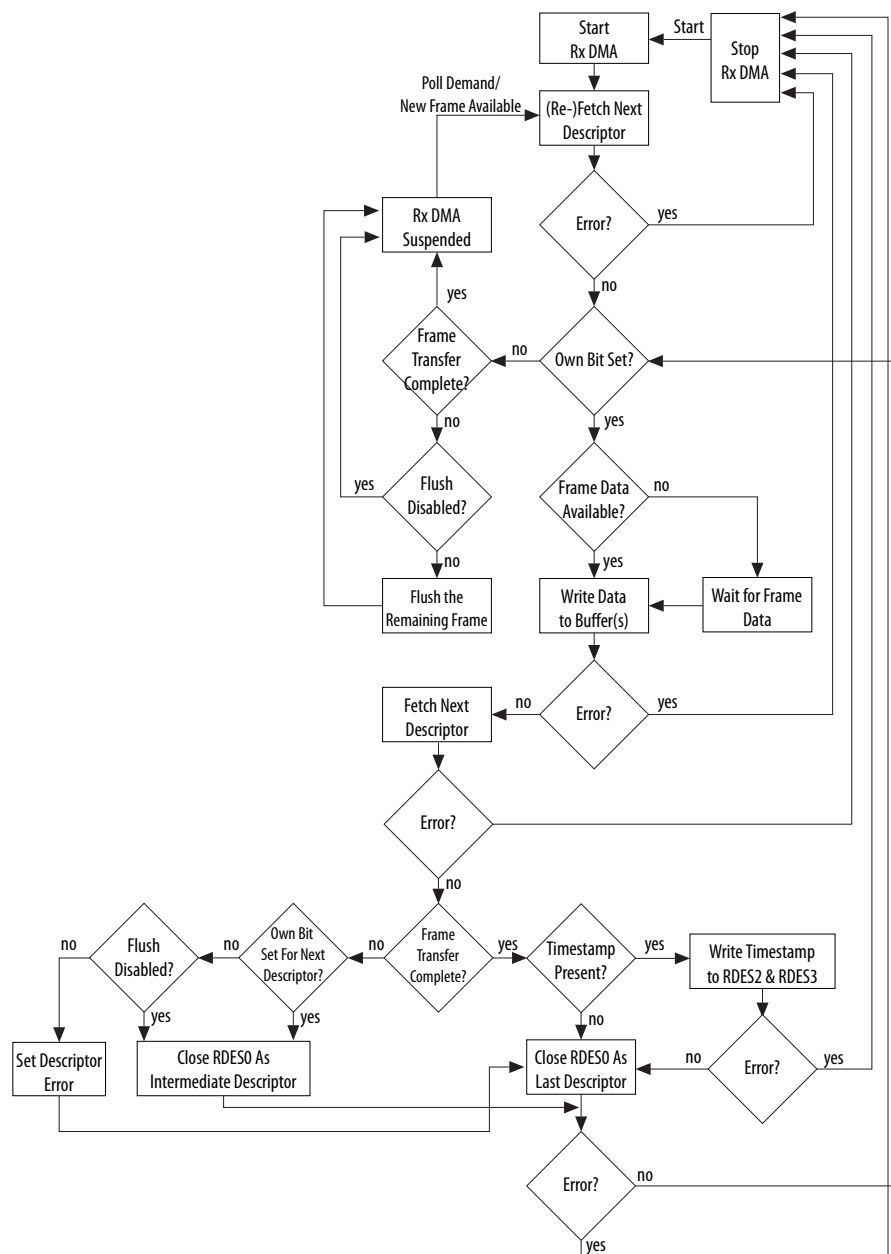
Figure 94. Receive DMA Operation
