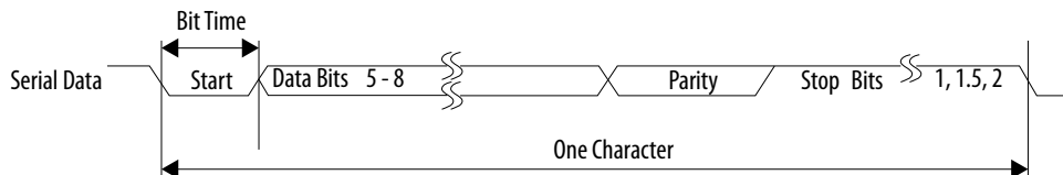
Figure 142. Serial Data Format
