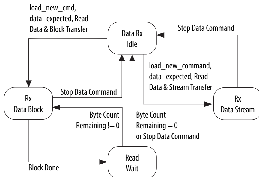
Figure 72. Data Receive State Machine †
