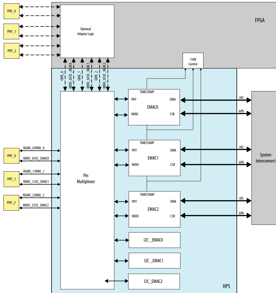
Figure 87. EMAC System Integration
