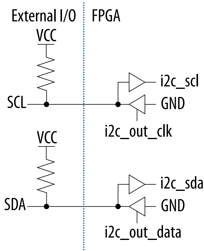
Figure 127. I 2 C Interface in FPGA Fabric
