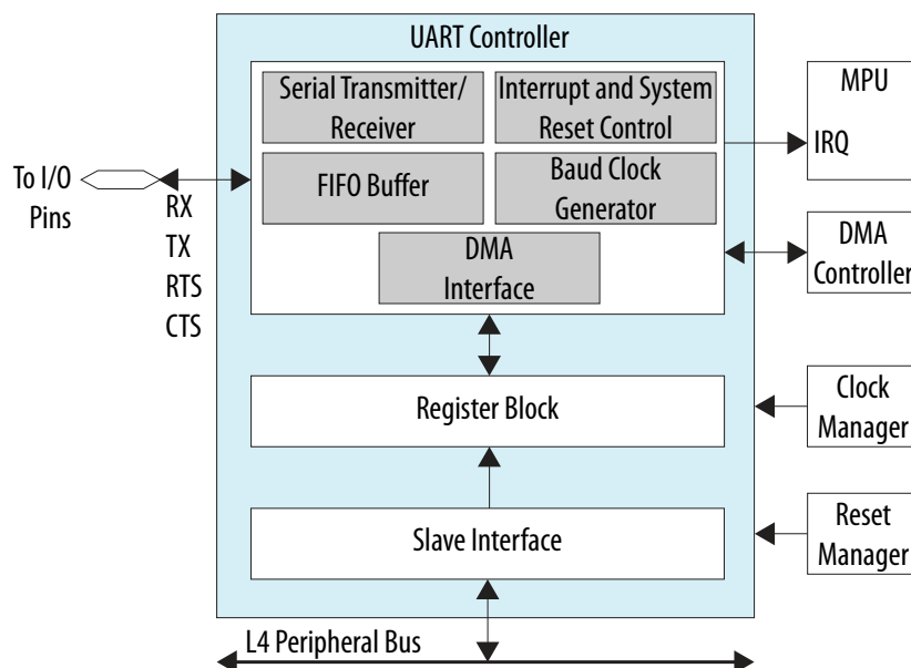
Figure 141. UART Block Diagram
