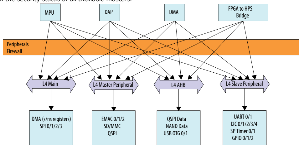
Figure 21. Peripheral Firewall
