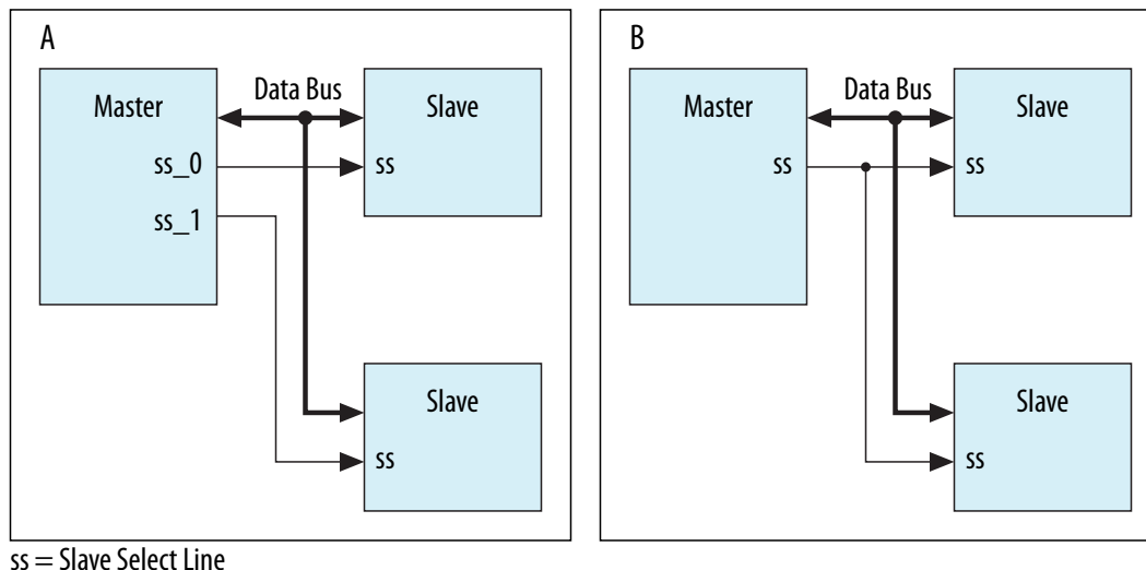
Figure 107. Hardware/Software Slave Selection
