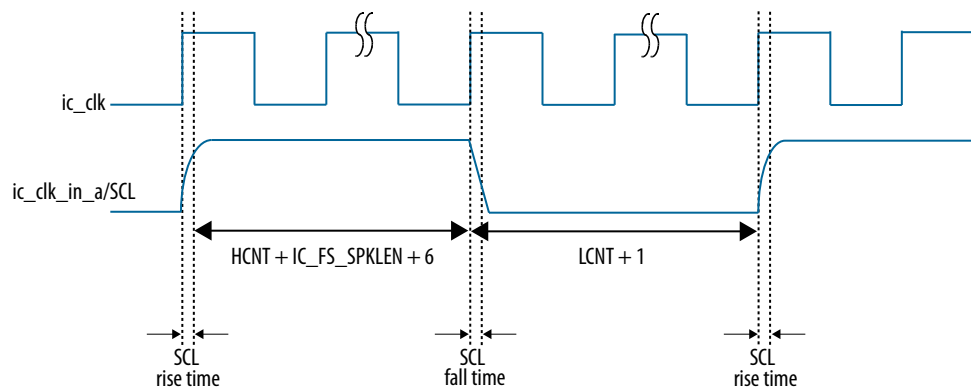
Figure 137. Impact of SCL Rise Time and Fall Time on Generated SCL
