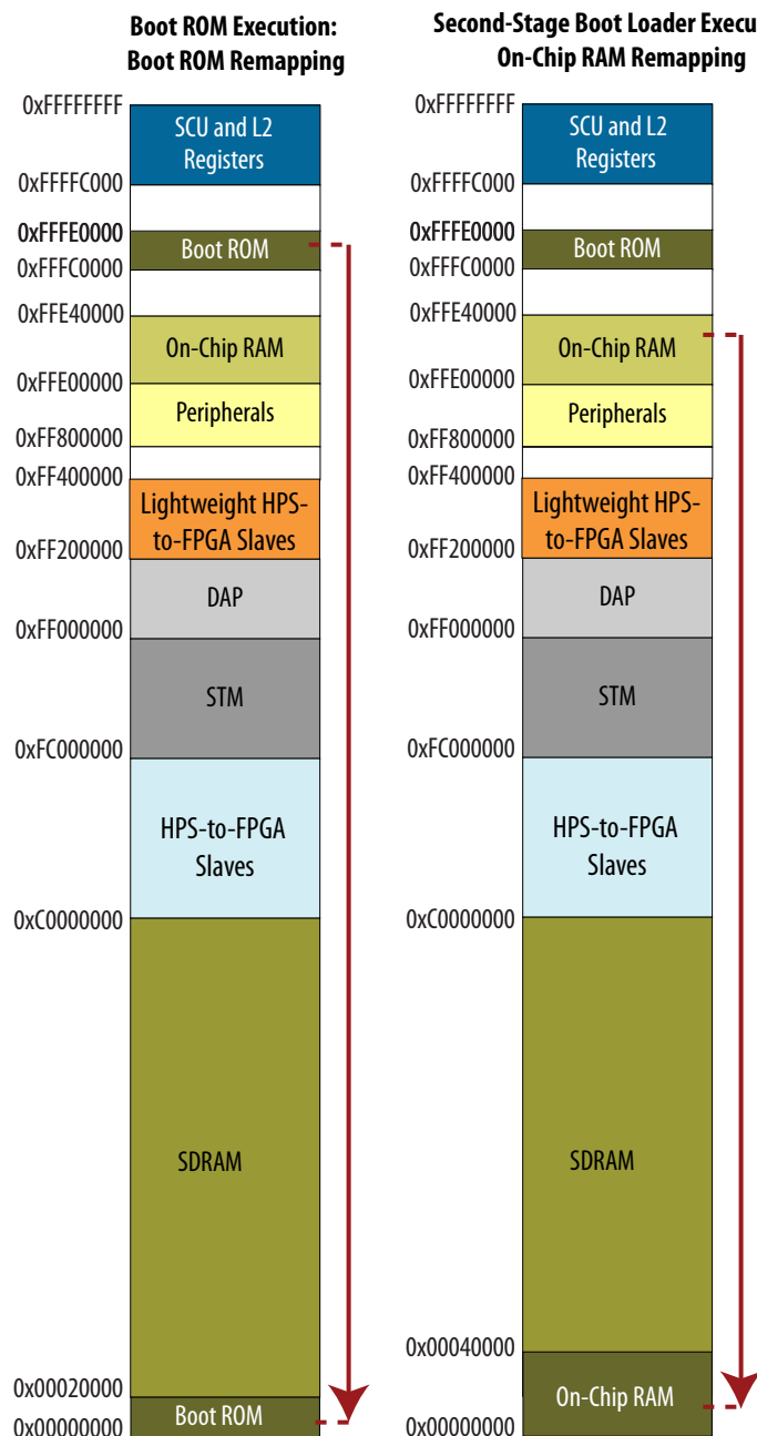
Figure 176. Remapping the On-Chip RAM
