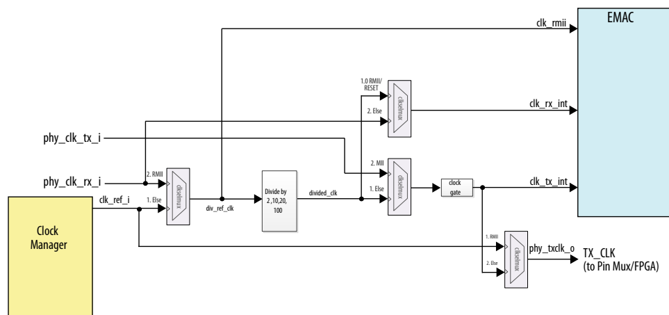
Figure 102. emac_clkgen Module
