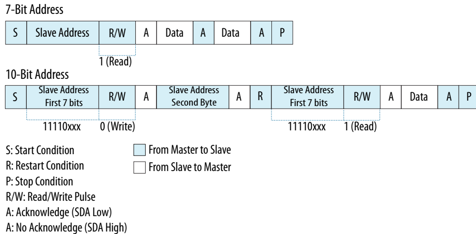
Figure 133. Master-Receiver Protocol †
