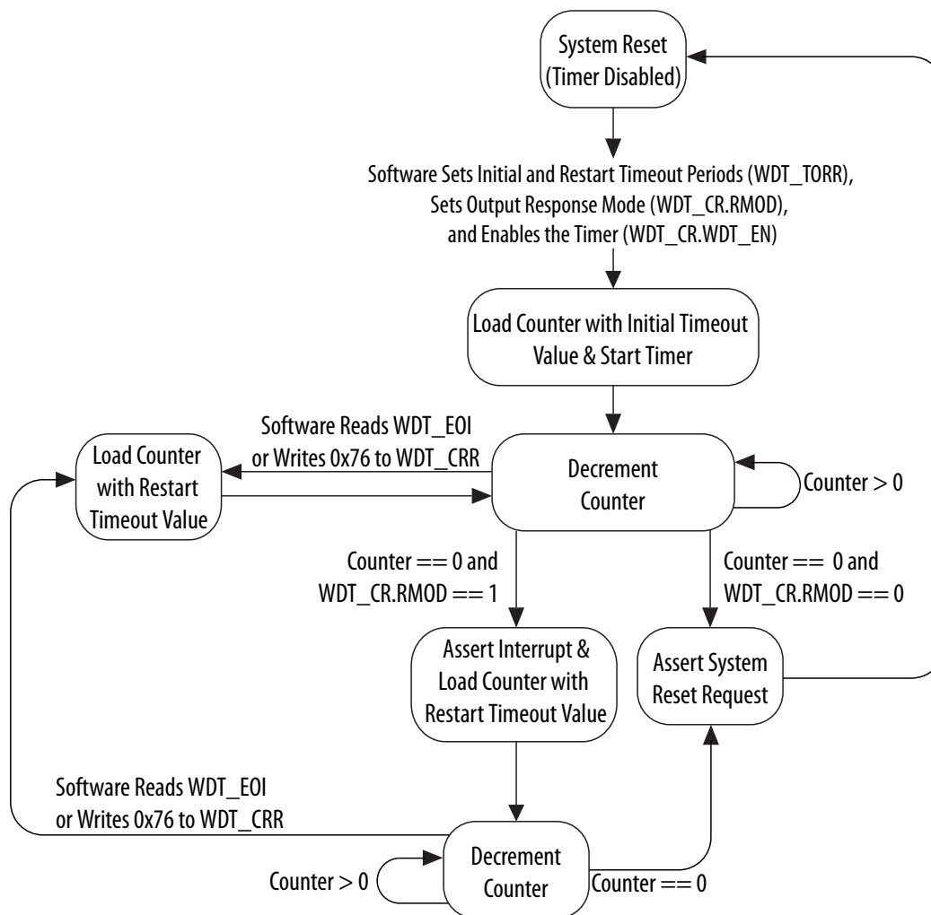
Figure 155. Watchdog Timer State Machine
