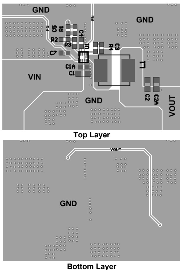
Figure 5: Recommended Layout
