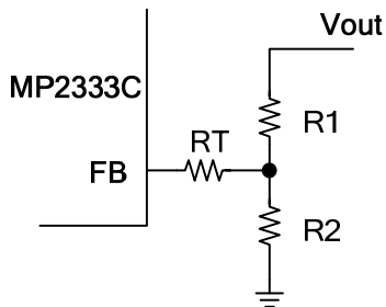
Figure 4: Feedback Network
