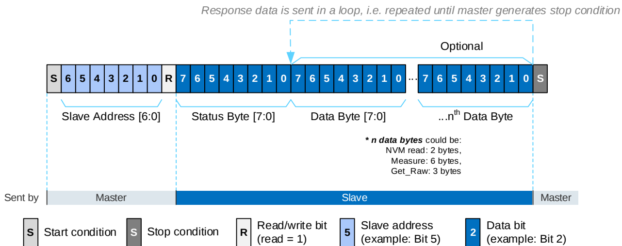
Figure 18. OWI Response by ZSSC3241
