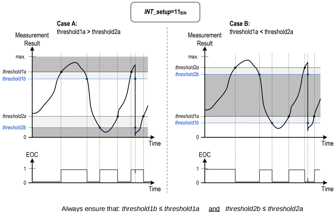
Figure 26. EOC and Dual-Interrupt Thresholds with Hysteresis ( \text{eoc\_hyst\_on}=1_{\text{BIN}} )
