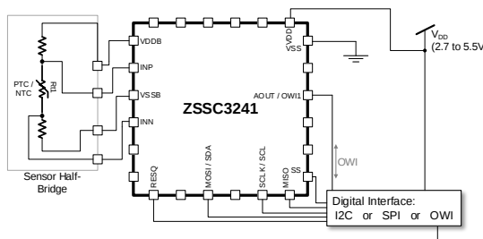
Digital Half-Bridge Sensor, e.g. PT100
