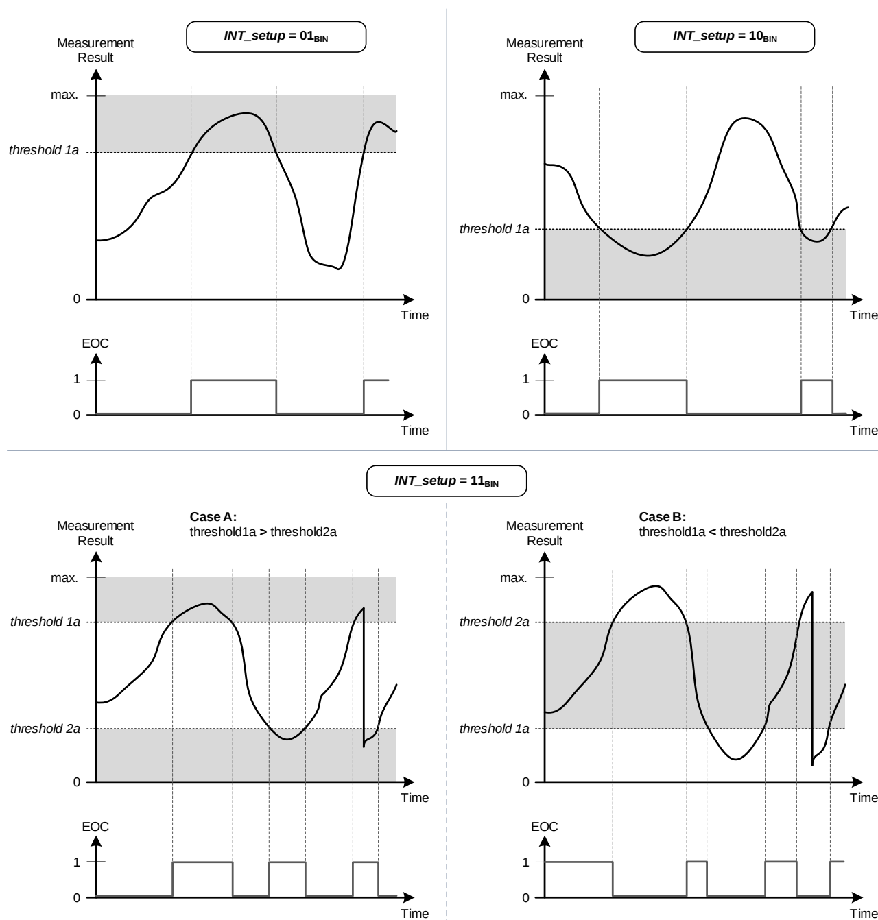
Figure 24. EOC and Interrupt Thresholds without Hysteresis ( eoc\_hyst\_on=0_{BIN} )
