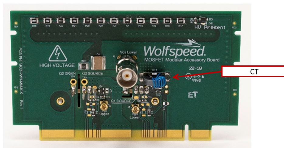
FIGURE 13: POWER DAUGHTER CARD POPULATED WITH CT USED FOR DRAIN CURRENT SENSING
