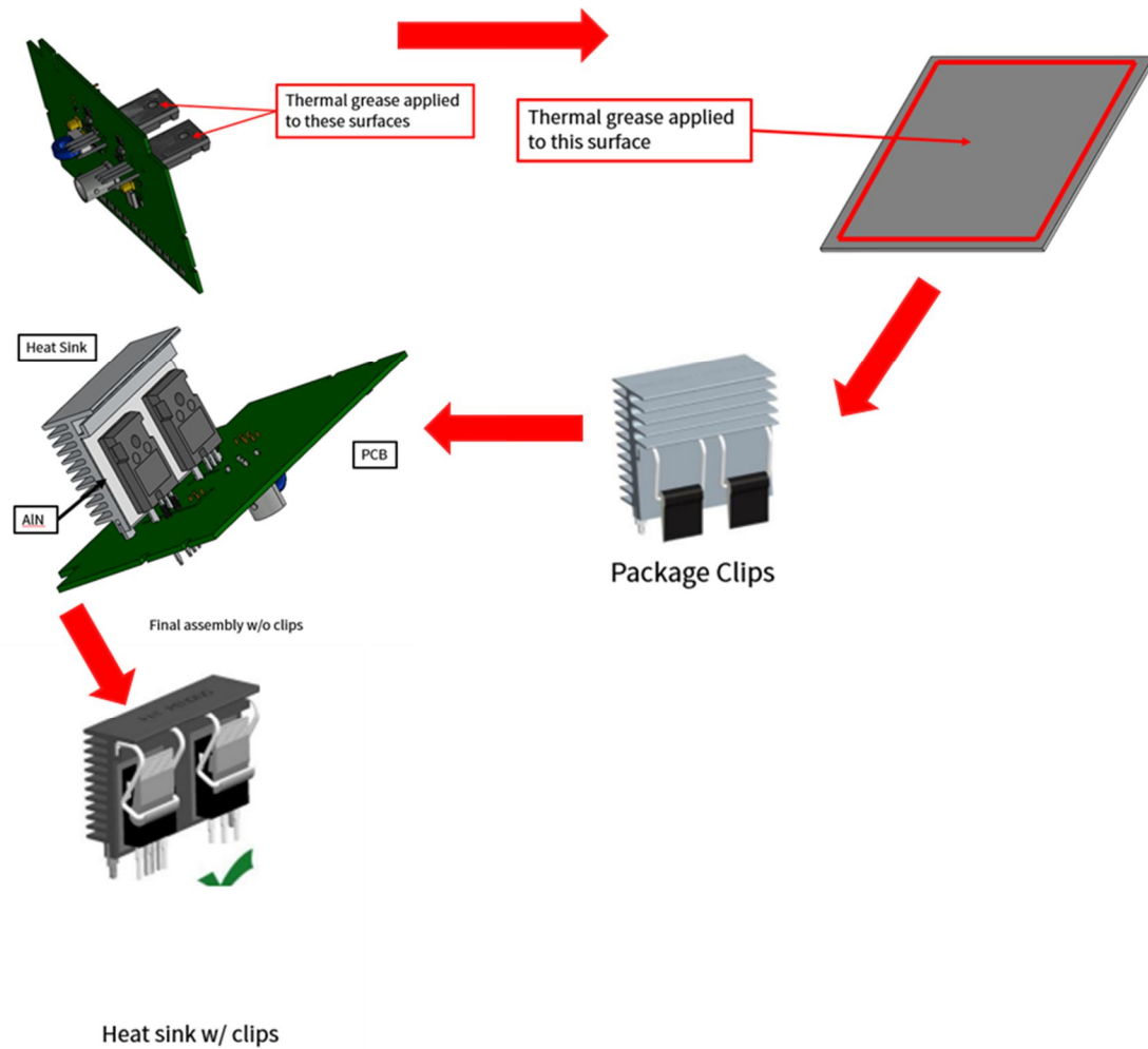
FIGURE 14: ASSEMBLY PROECEDURE FOR MOSFETS AND HEATSINK
