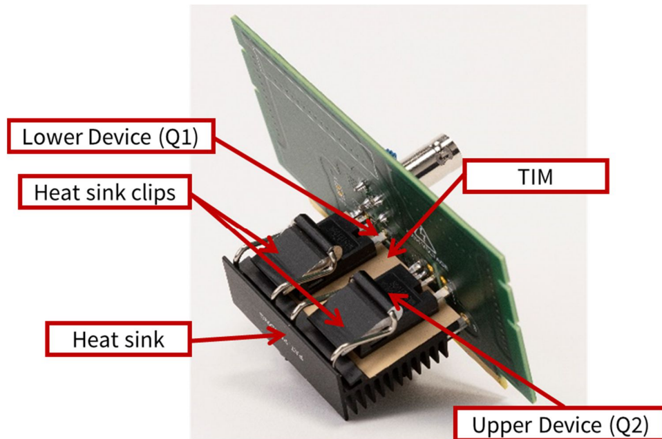
FIGURE 4: POWER DAUGHTER CARD: BACK VIEW SHOWING DEVICES AND THERMAL MANAGEMENT SYSTEM
