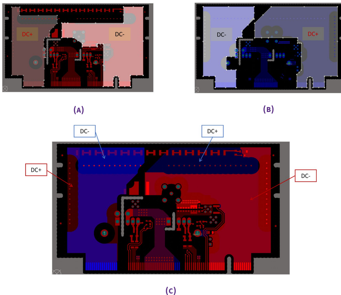
FIGURE 7: THE COPPER POURS FOR THE DC LINK CONNECTIONS BETWEEN THE MOTHERBOARD AND POWER DAUGHTER CARD. THESE IMAGES SHOW HOW THE LOOP INDUCTANCE IN DC LINK IS REDUCED.
