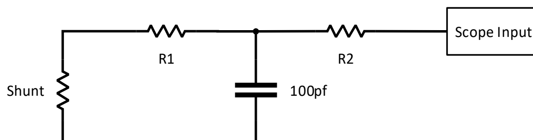
FIGURE 12: POWER TESTING OPTIMIZED SHUNT: USE VALUES OF R1 AND R2 FROM TABLE 1
