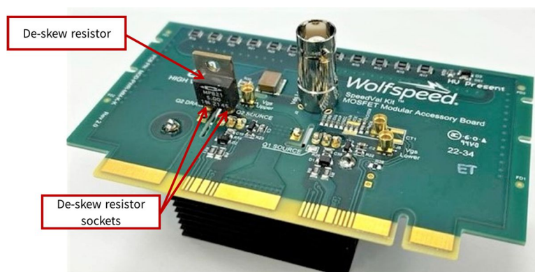
FIGURE 9: DESKEW RESISTOR POSITION ON THE POWER TO-247-4 POWER DAUGHTER CARD
