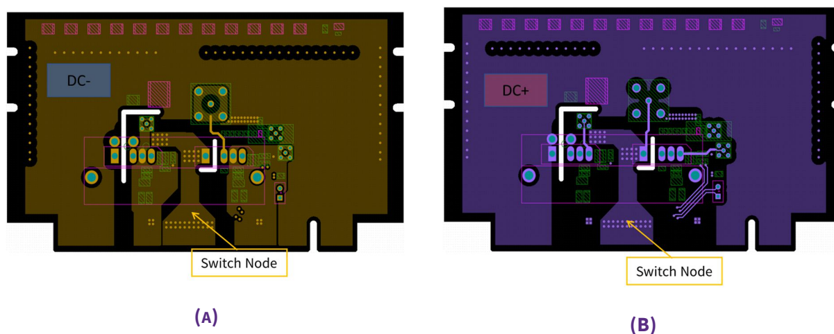
FIGURE 8: COPPER POURS FOR THE +/- VBUS IN THE INNER TWO LAYERS OF THE PCB TO MINIMIZE THE LOOP INDUCTANCE BETWEEN THE CONNECTION POINTS ON THE BOARD.
