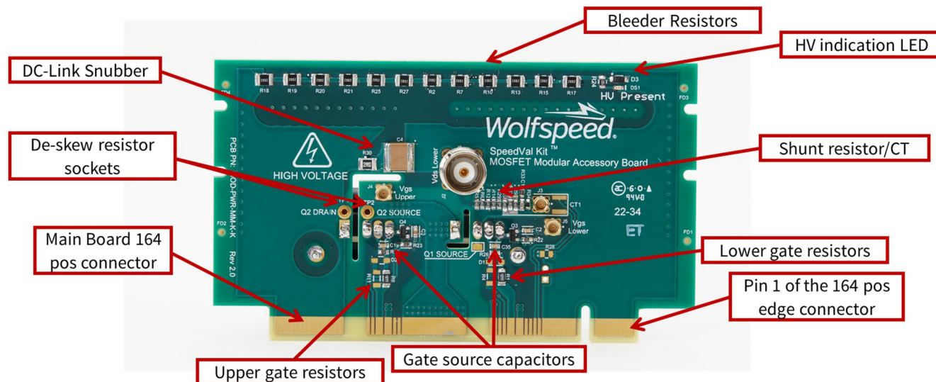
FIGURE 5: POWER DAUGHTER CARD: FRONT VIEW SHOWING VARIOUS COMPONENTS AND FEATURES OF THE BOARD
