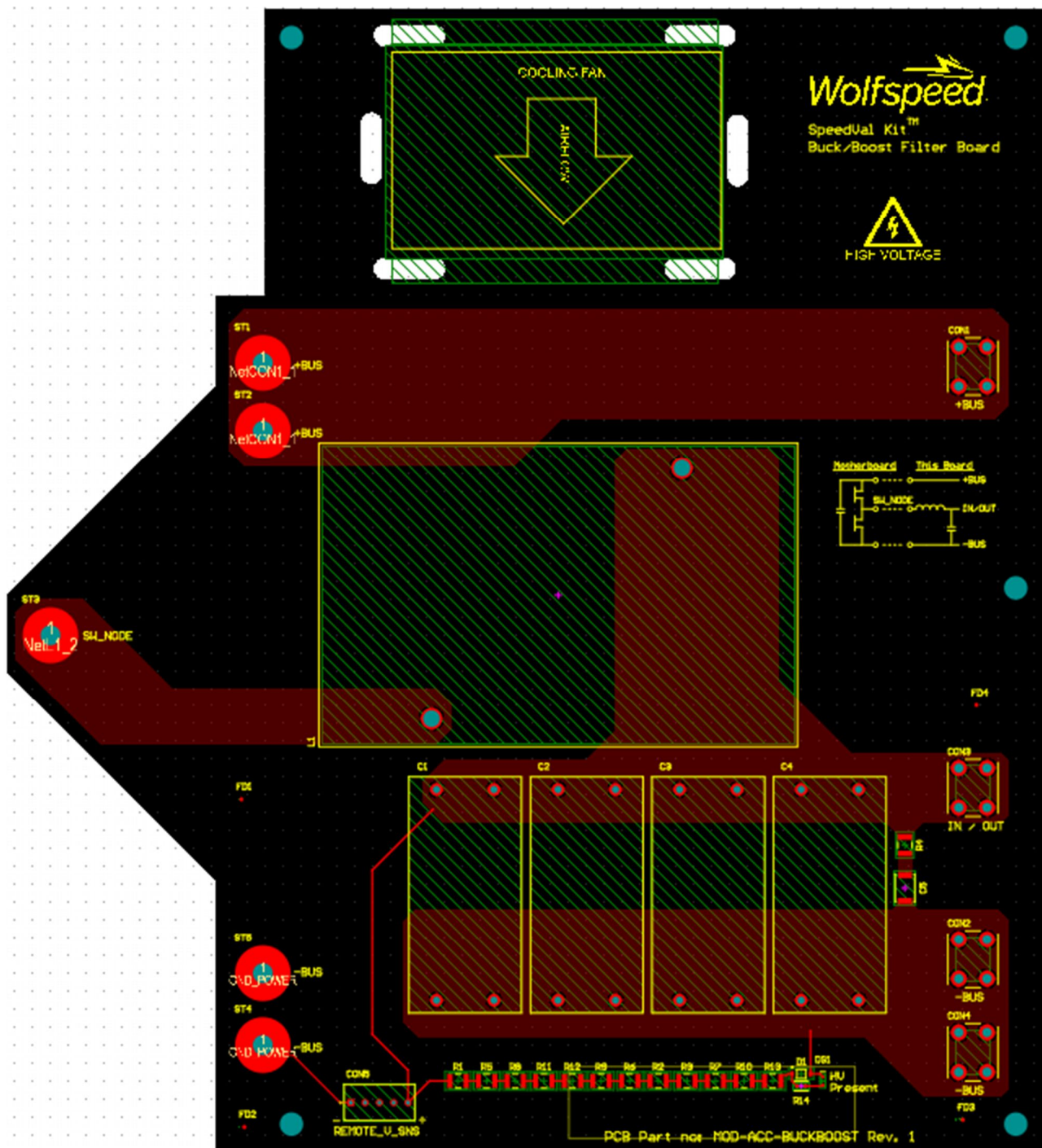
FIGURE 9: PCB LAYOUT- TOP LAYER
