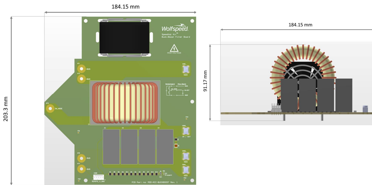
FIGURE 3: DIMENSIONS OF THE BUCK/BOOST FILTER BOARD
