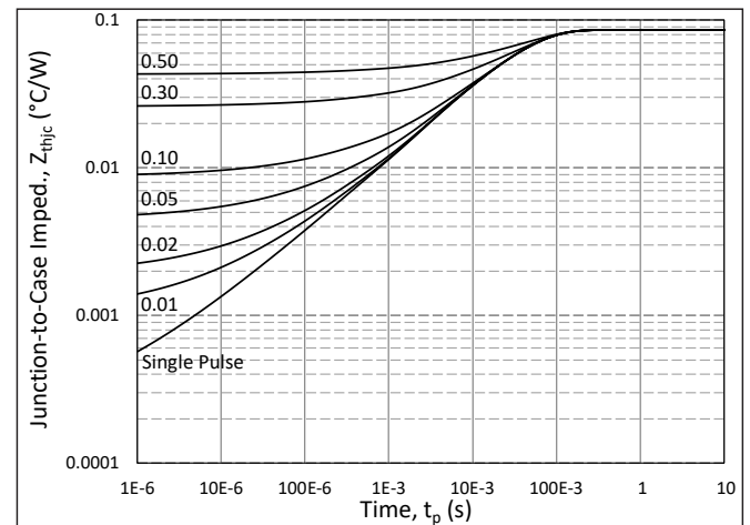
Figure 18. Diode Junction to Case Transient Thermal Impedance, Z_{\text{thjc}} ( ^{\circ}\text{C/W} )
