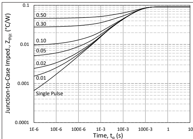
Figure 17. MOSFET Junction to Case Transient Thermal Impedance, Z_{\text{thjc}} ( ^{\circ}\text{C/W} )
