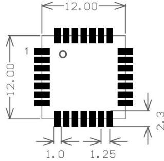
Figure 11 PCB footprint
