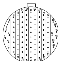
22-35 (M) Size 22 100#22
