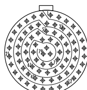
20-35 (M) Size 20 79#22
