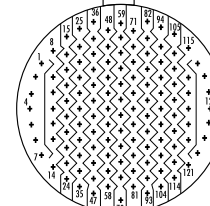
24-35 (M) Size 24 128#22
