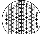
18-35 (M) Size 18 66#22
