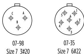
INSERT ARRANGEMENTS
