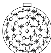
20-41 (I) Size 20 41#20
