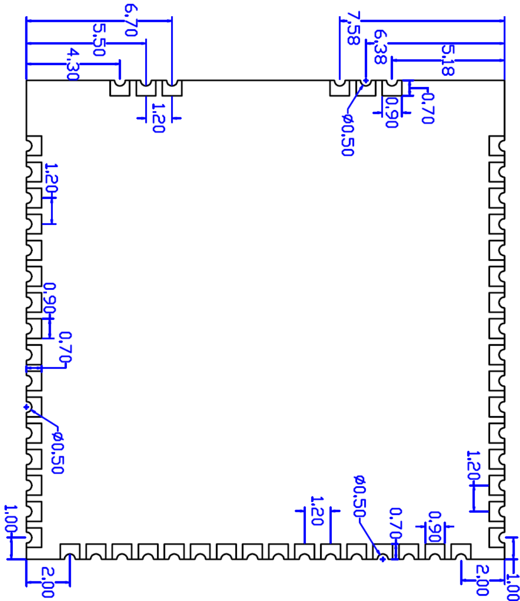
Bottom View
