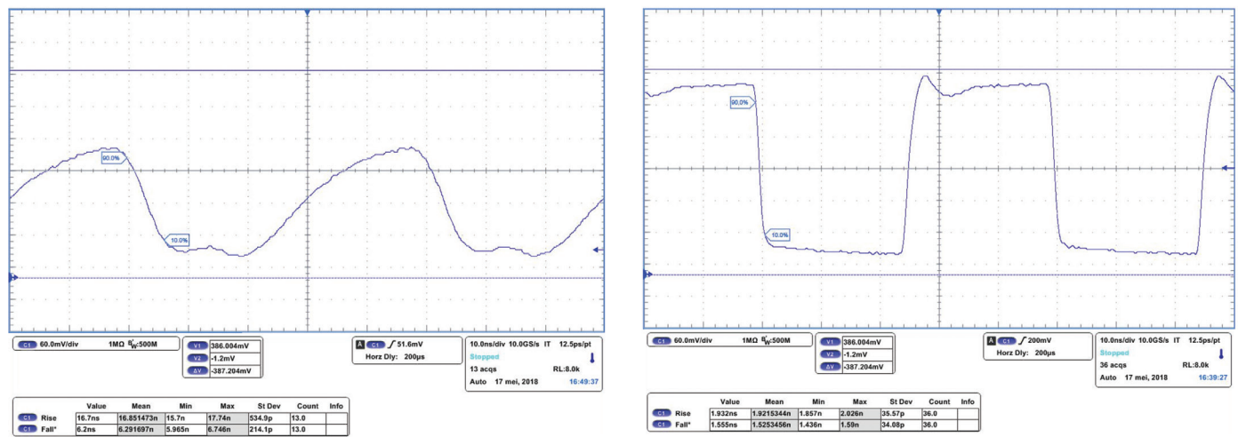
Figure 12. Pulsed behavior of a LUXEON L110 – 0940xxx emitter in a Melexis TOF evaluation kit (left) vs VCSEL (right). Modulation frequency 20MHz, integration time 400μs.
