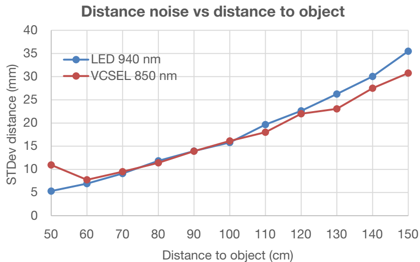
Figure 15. Distance noise measured for VCSEL and LED TOF system, at 12MHz modulation frequency, as a function of the distance to the object being measured
