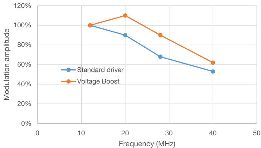
Figure 14. Modulation amplitude vs modulation frequency with and without voltage boost. The modulation amplitude at 12MHz is used as reference (integration time = 150 \mu s, drive current = 3.5A).
