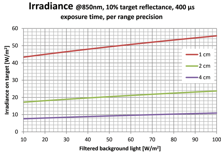
Figure 5. Irradiance on target required to reach different measurement precision values (1, 2 and 4cm respectively) as a function of filtered ambient background light levels. Note: Irradiance values shown here correspond to average irradiance within a burst.
