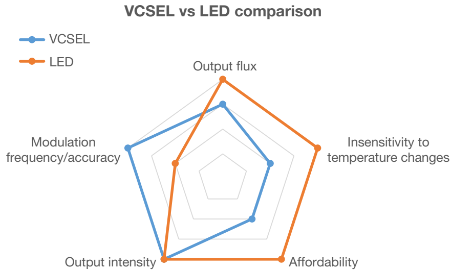
Figure 17. Qualitative comparison of IR VCSELs versus LEDs
