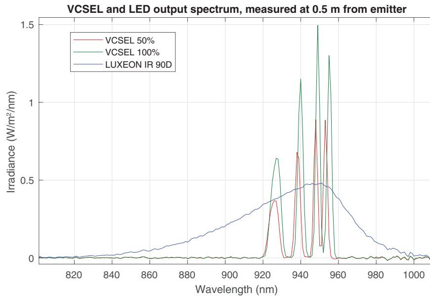
Figure 8. Measured spectra for VCSEL (driven at 50% and 100% of maximum current) and LED emitters (250µs burst length, 20MHz modulation frequency). Note: the spectrometer resolution (~2.5nm) is not good enough to resolve the VCSEL spectral width (< 1nm). The VCSEL shift in wavelength when increasing the drive current is due to temperature increase at higher current.
