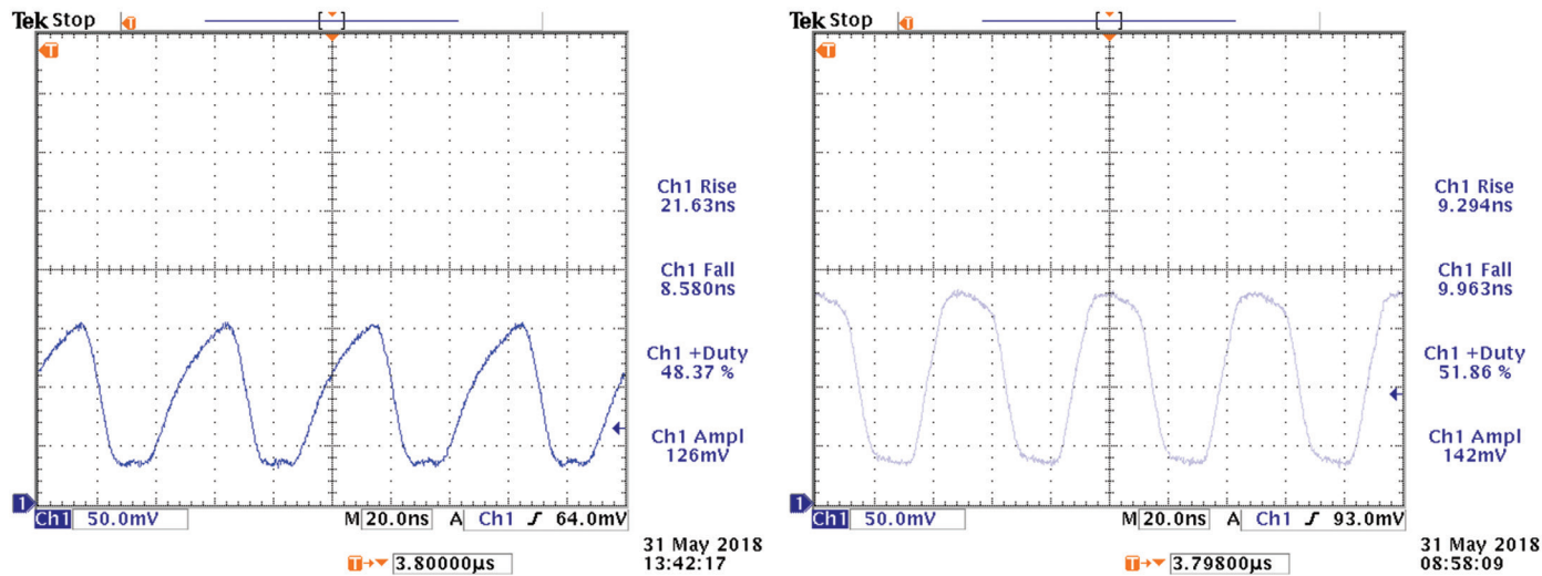
Figure 13. Pulsed behavior of a LUXEON L110 – 0940xxx emitter without (left) and with voltage booster circuit (right). Modulation frequency 20MHz, integration time 150μs, drive current = 3.5A.
