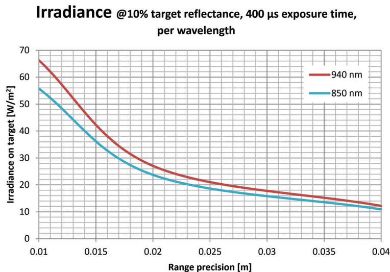
Figure 6. Irradiance on target required to reach a certain precision at 850nm and 940nm, at 100 klux ambient light condition. Note: Irradiance values shown here correspond to average irradiance within a burst.
