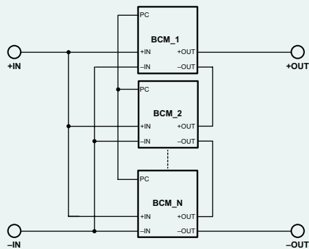
Figure 3: BCMs with outputs connected in series for higher output voltage.
