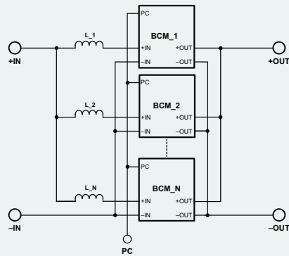
Figure 2: BCM converters in a parallel array.
