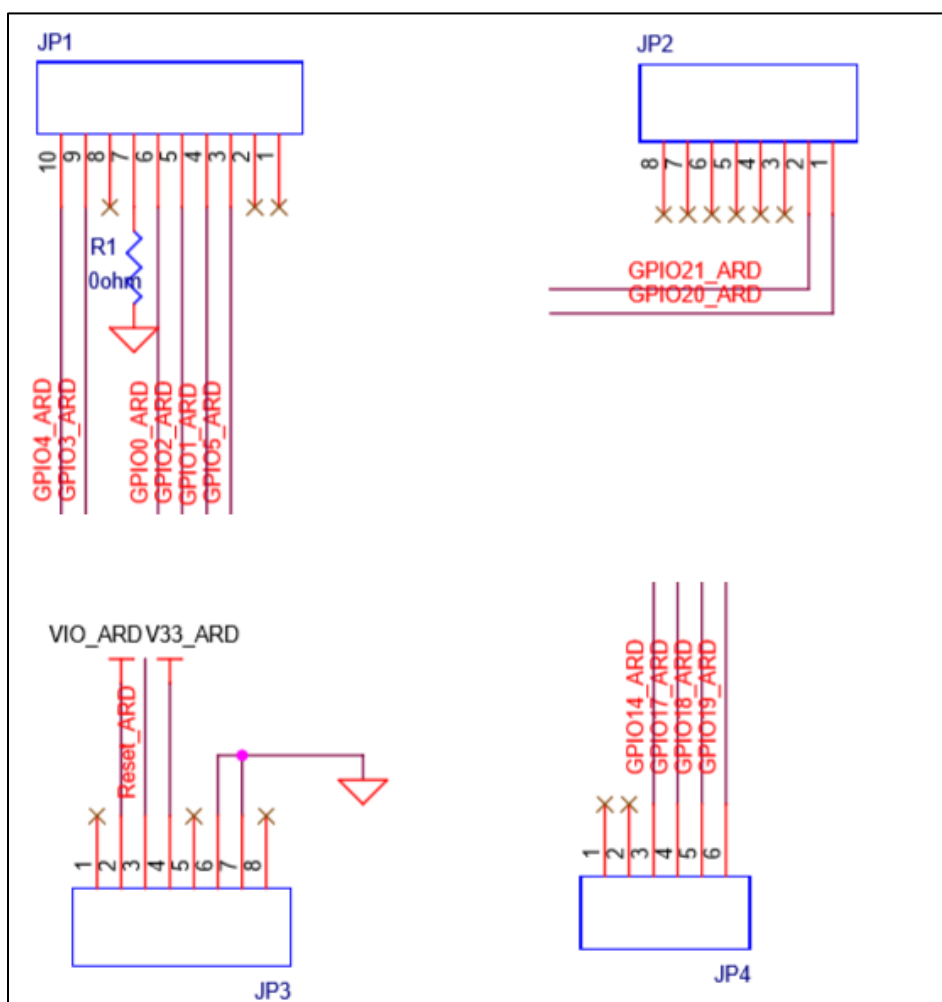
Figure 6: Arduino UNO shield compatible jumpers
