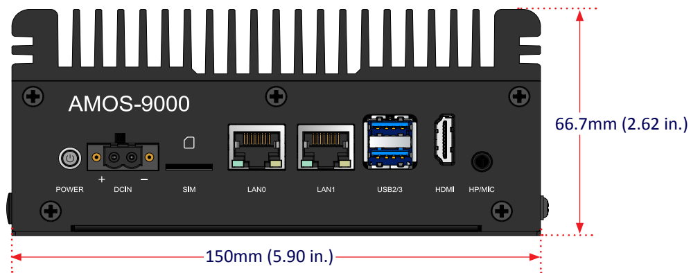
Figure 05: Dimensions of the VIA AMOS-9000 system (front panel I/O)
