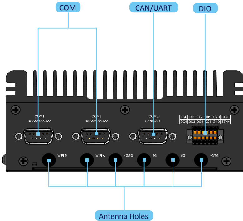
Figure 02: VIA AMOS-9000 system back panel I/O
