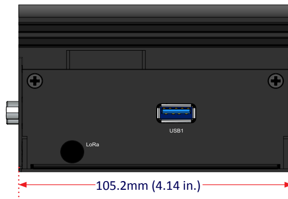
Figure 06: Dimensions of the VIA AMOS-9000 system (left panel I/O)
