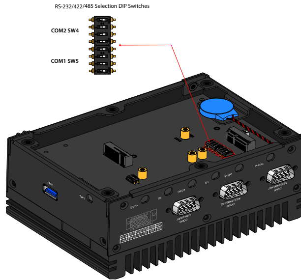
Figure 25: Location of the RS-232/422/485 selection DIP switches
