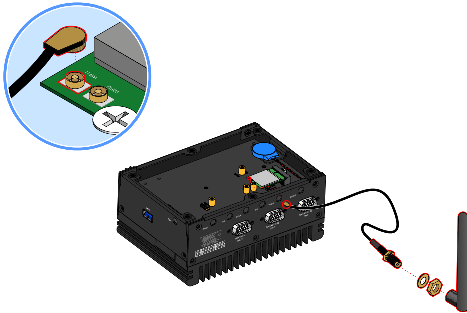
Figure 32: Installing the antennas
