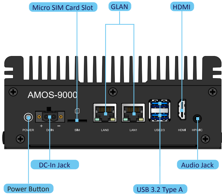
Figure 01: VIA AMOS-9000 system front panel I/O
