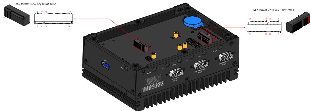
Figure 23: Location of the M.2 slots
