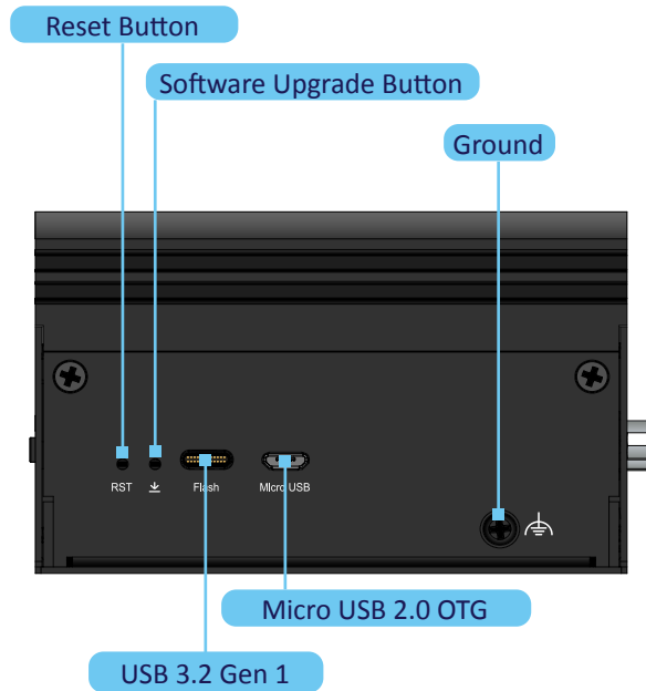
Figure 04: VIA AMOS-9000 system right panel I/O
