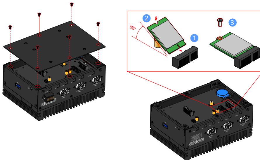
Figure 31: Installing and securing the Wi-Fi module
