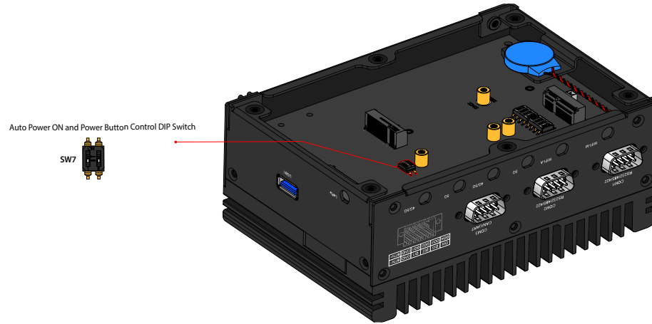
Figure 27: Location of the auto power ON and power button control DIP switch
