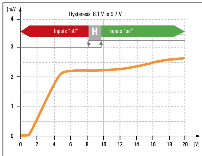
Current-voltage characteristic of P-switching digital inputs
