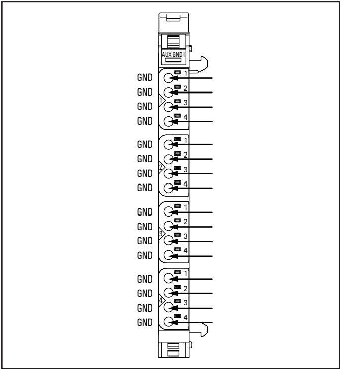
Connection diagram UR20-16AUX-GND-I
