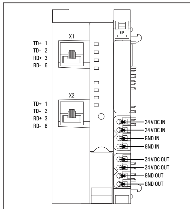
Connection diagram UR20-FBC-EIP-V2
