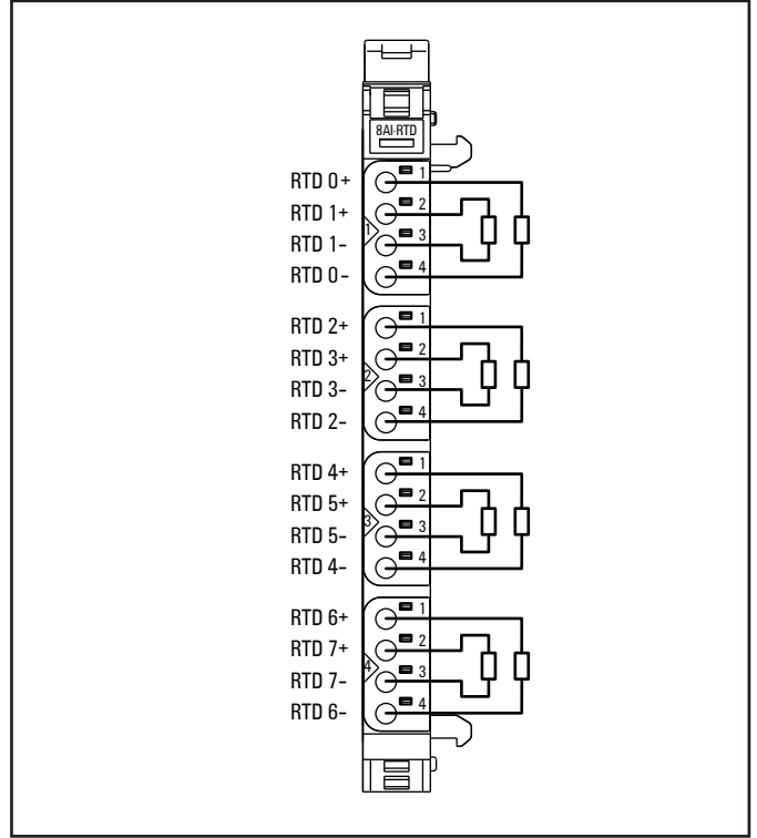
Connection diagram UR20-8AI-RTD-DIAG-2W
