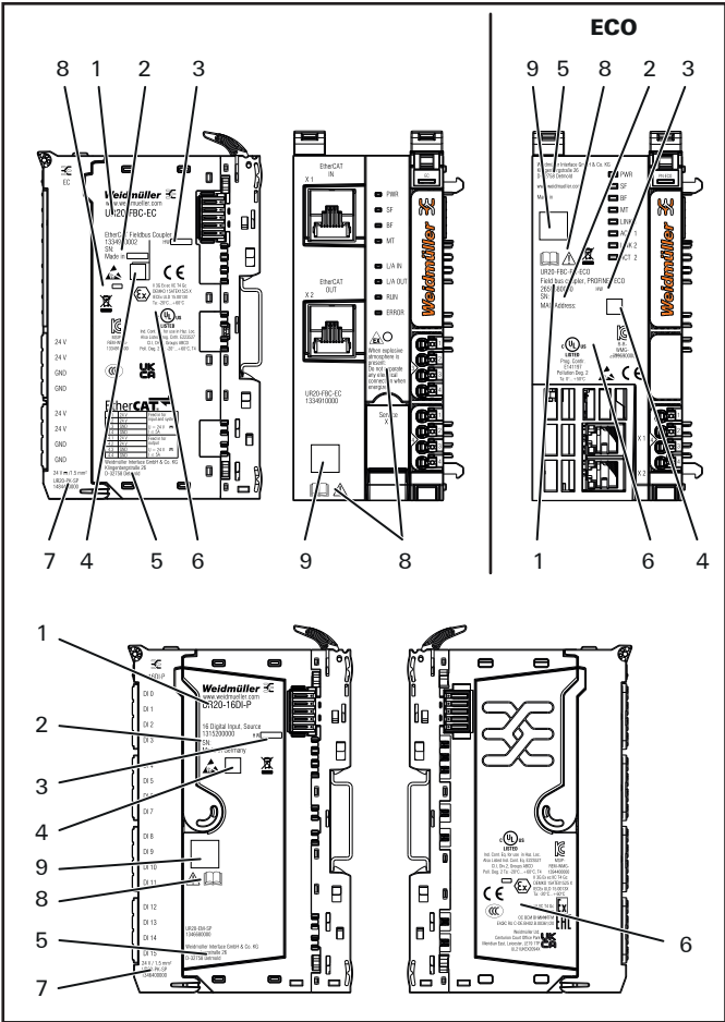
Type plate (examples)
