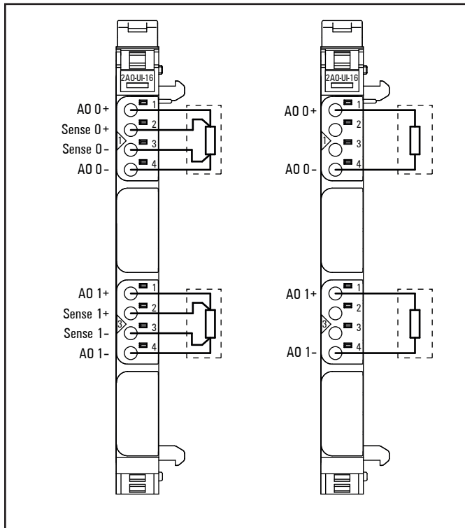
Connection diagram UR20-2AO-UI-16
