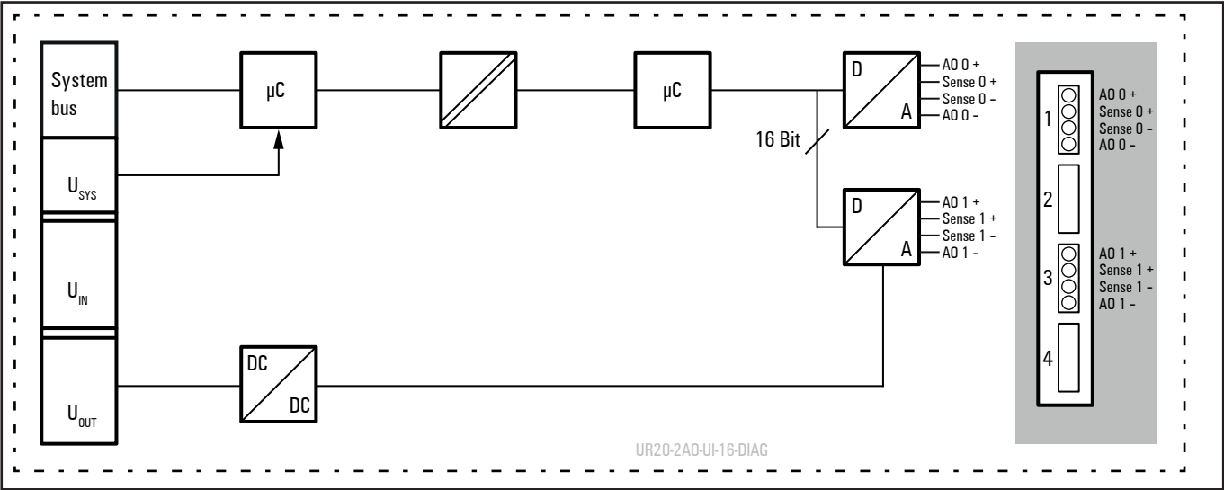
Block diagram UR20-2AO-UI-16-DIAG
