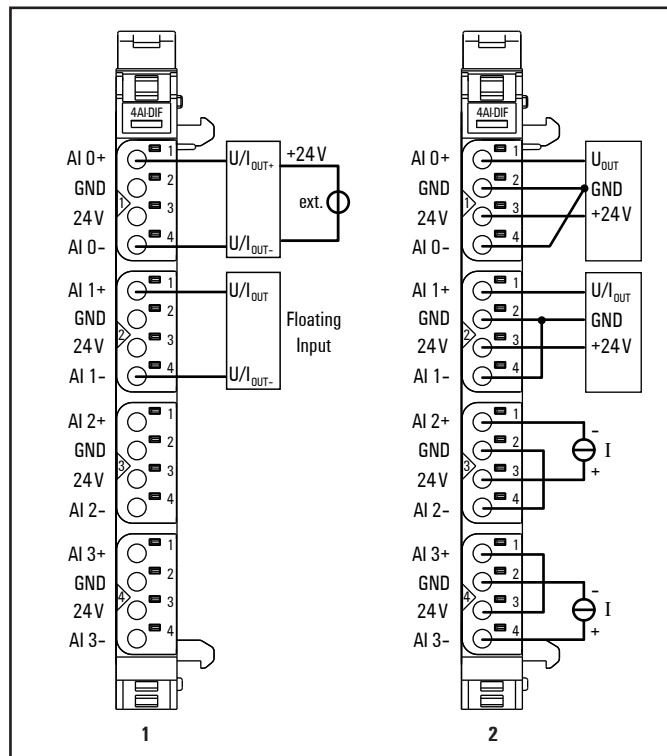
Connection diagramm UR20-4AI-UI-DIF-16-DIAG (1 = Standard, 2 = alternative option)
