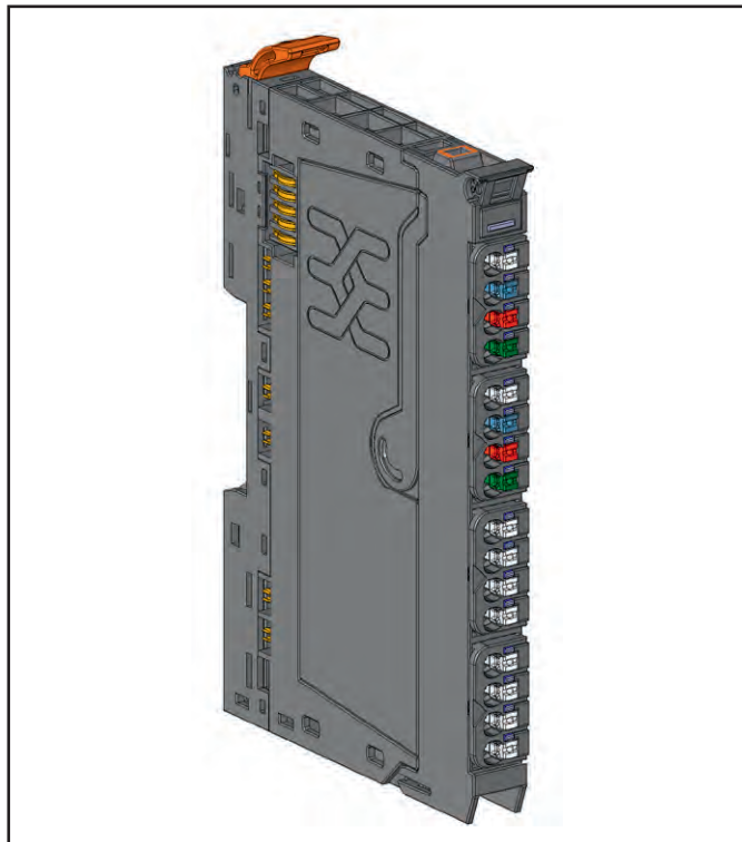
Current controlled PWM module UR20-2PWM-I-2.5A-2DI-P (Order No. 2697910000)
