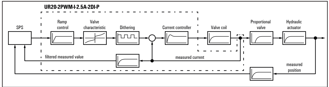
Example: current-controlled PWM module in cascade control for positioning a hydraulic actuator
