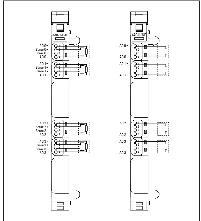
Connection diagram UR20-4AO-UI-16-DIAG-HD
