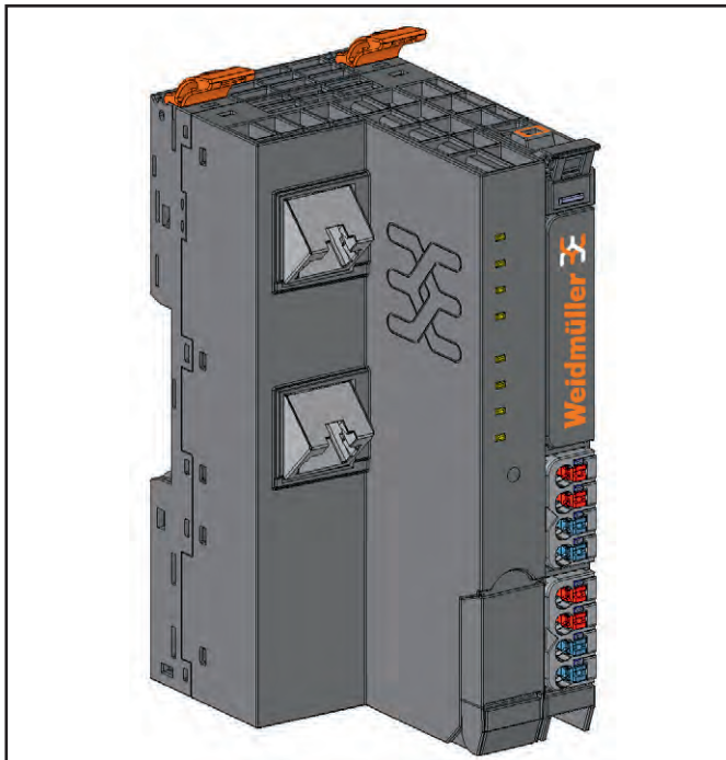
Fieldbus coupler UR20-FBC-EIP-V2 (Order No. 1550550000)
