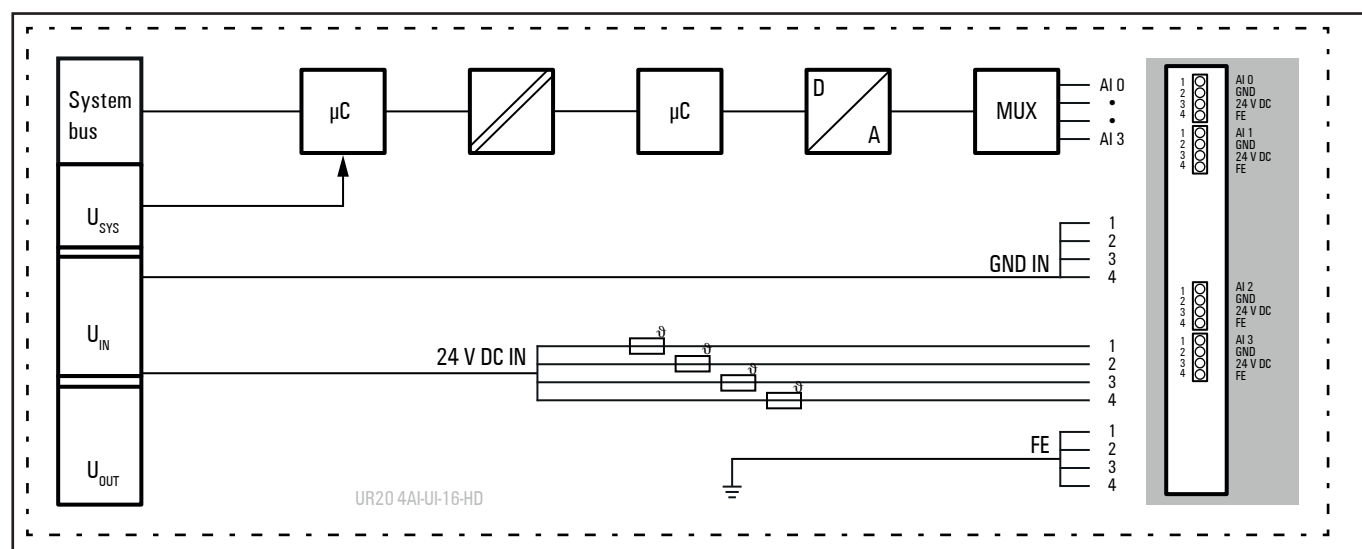
Block diagram UR20-4AI-UI-16-HD
