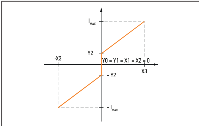
Characteristic curve for dead zone compensation
