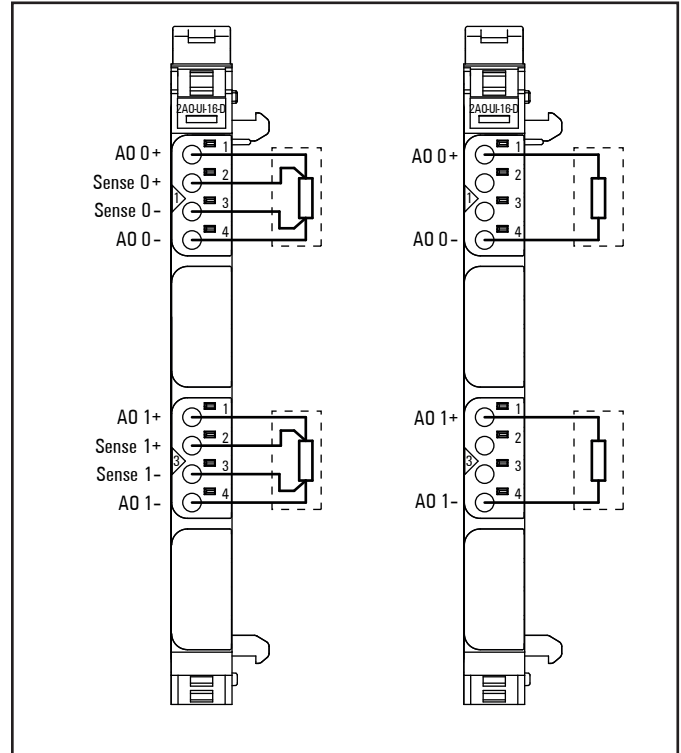
Connection diagram UR20-2AO-UI-16-DIAG
