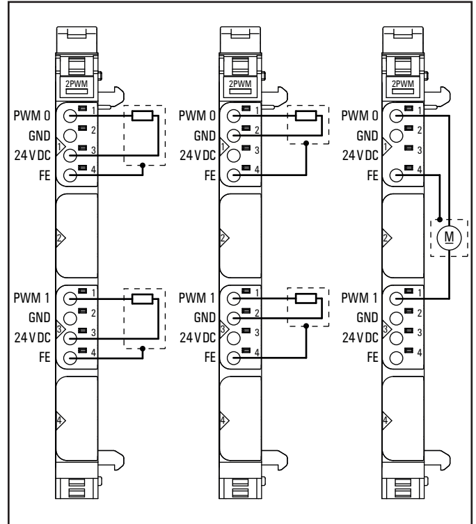
Connection diagram UR20-2PWM-PN-0.5A
