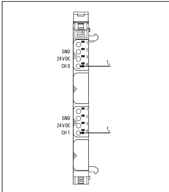
Connection diagram UR20-2FCNT-100
