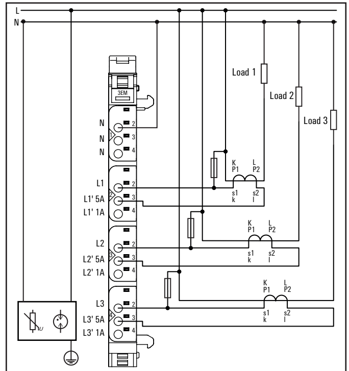
Connection diagram UR20-3EM-230V-AC: Single phase measurement with current transformer
