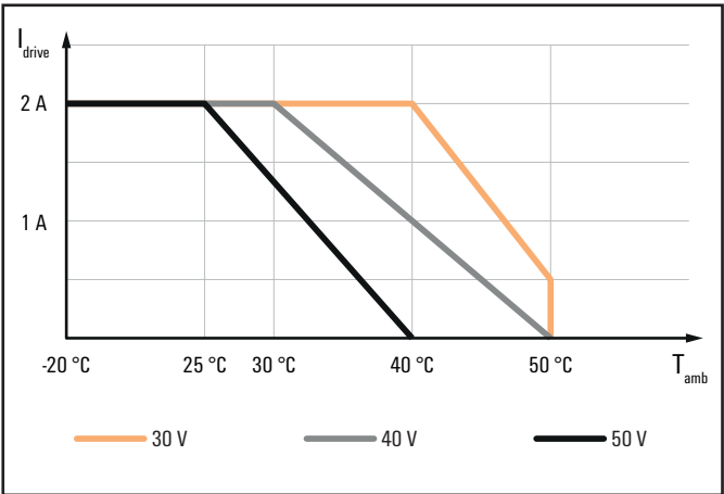
Derating curve UR20-1SM-50W-6DI2D0-P with vertical installation
