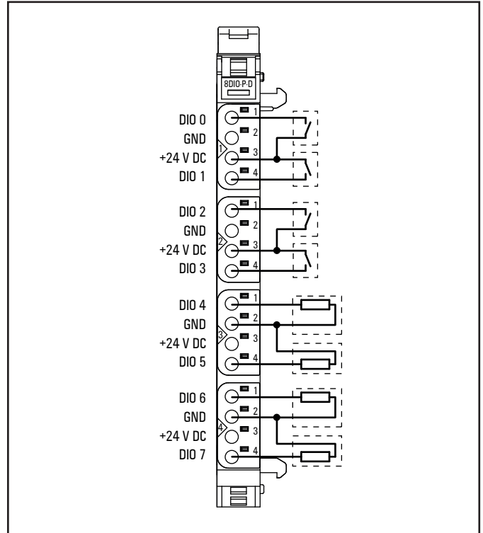
Connection diagram UR20-8DIO-P-3W-DIAG (Example: 4 inputs, 4 outputs)
