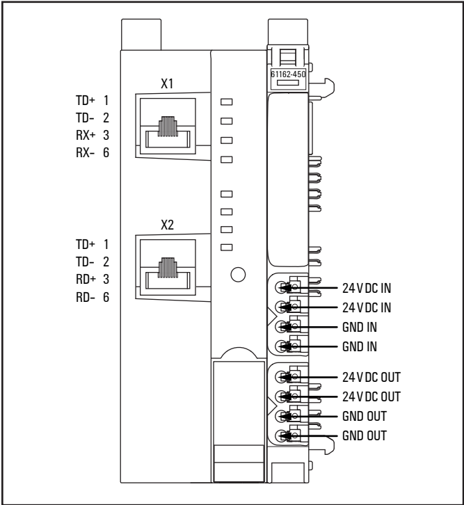
Connection diagram UR20-FBC-IEC61162-450
