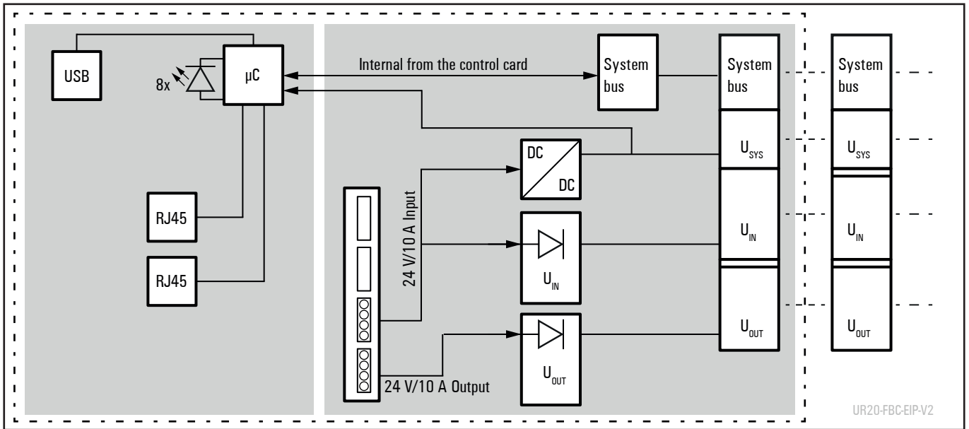
Block diagram UR20-FBC-EIP-V2
