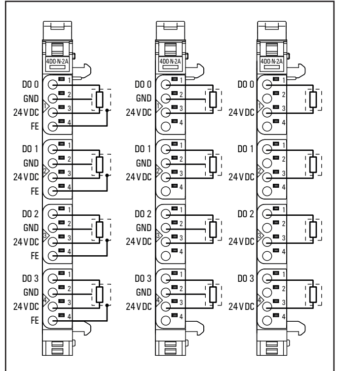
Connection diagram UR20-4DO-N-2A
