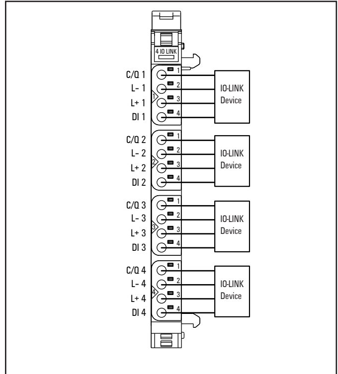
Connection diagram UR20-4COM-IO-LINK-V2
