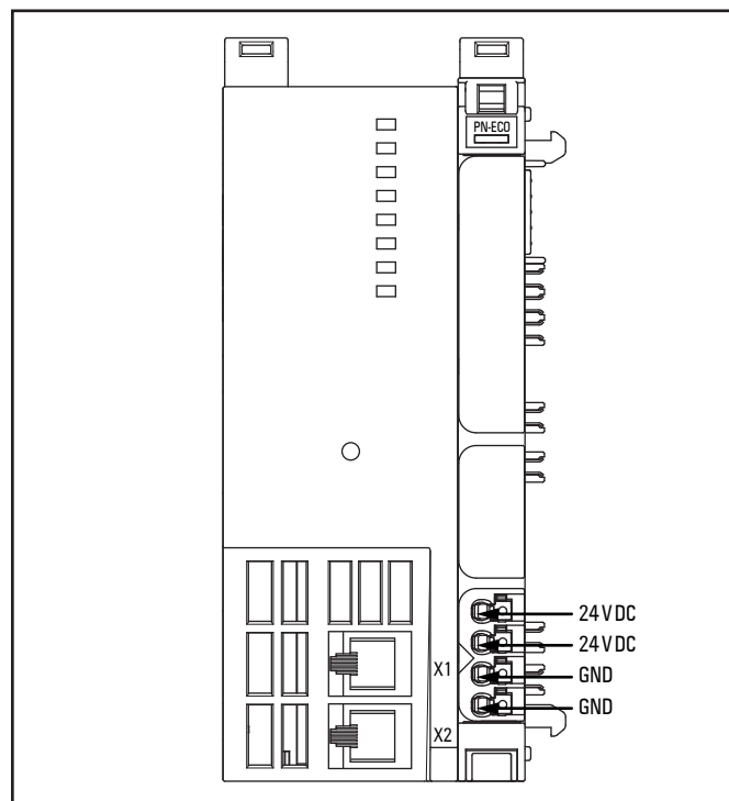
Connection diagram UR20-FBC-PN-ECO
