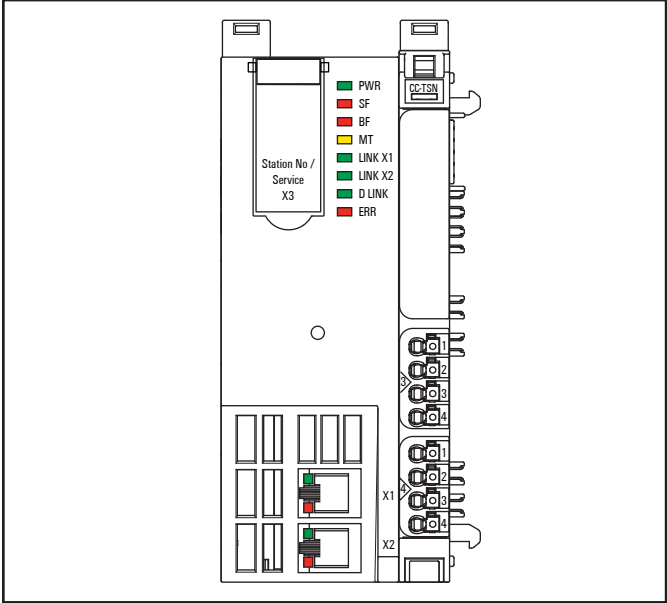
LED status indicators UR20-FBC-CC-TSN, error messages see chapter 12
