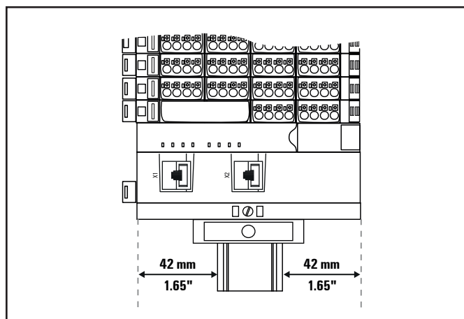
Installation position of the u-remote station on the DIN rail (vertical installation)
