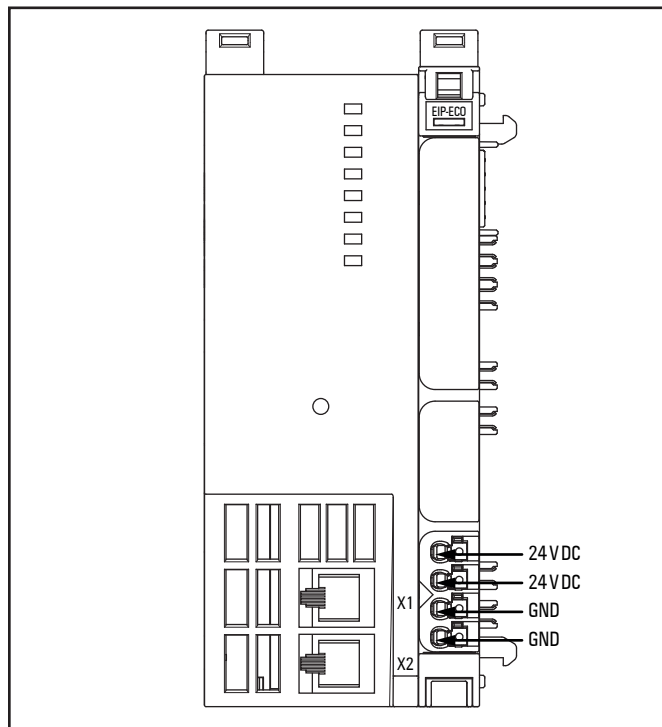
Connection diagram UR20-FBC-EIP-ECO
