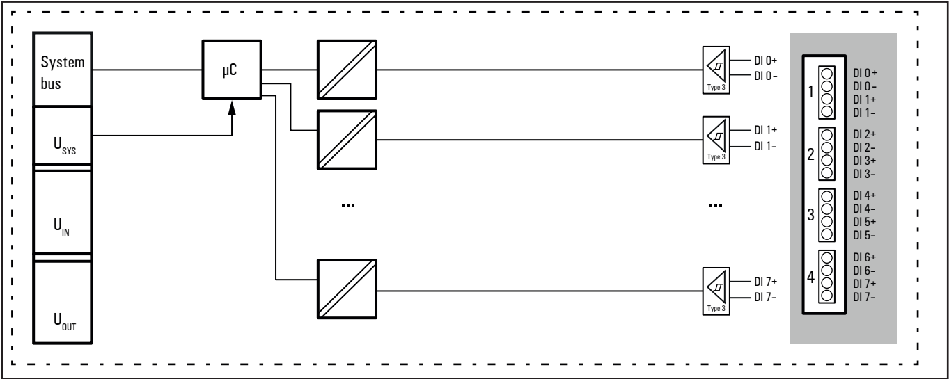
Block diagram UR20-8DI-IS0-2W
