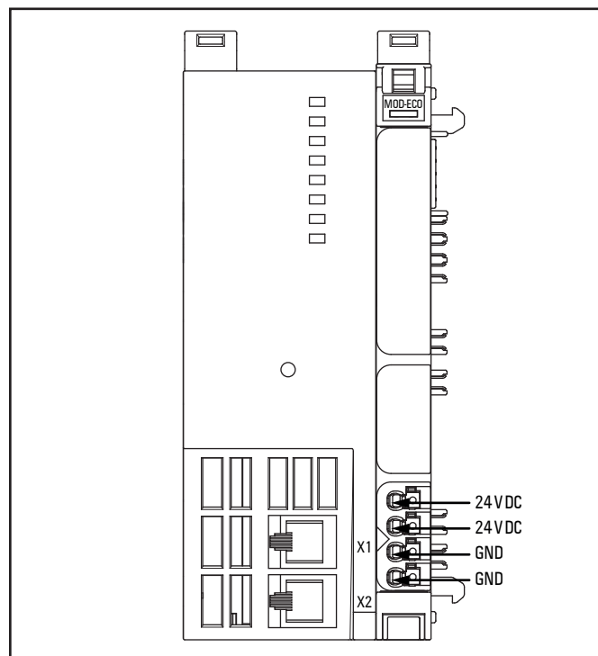
Connection diagram UR20-FBC-MOD-TCP-ECO
