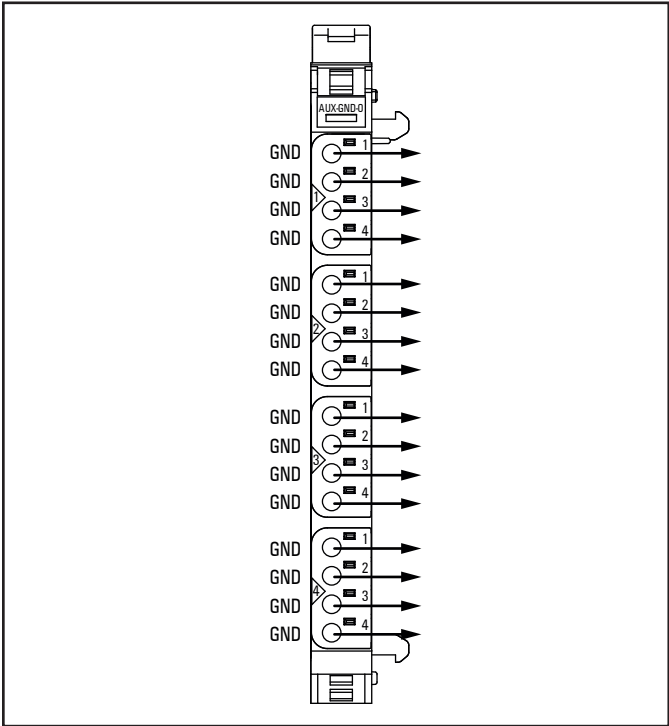
Connection diagram UR20-16AUX-GND-O
