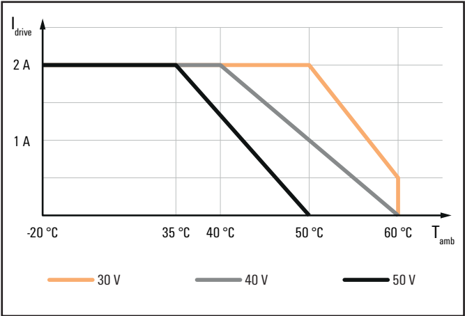
Derating curve UR20-1SM-50W-6DI2D0-P with horizontal installation
