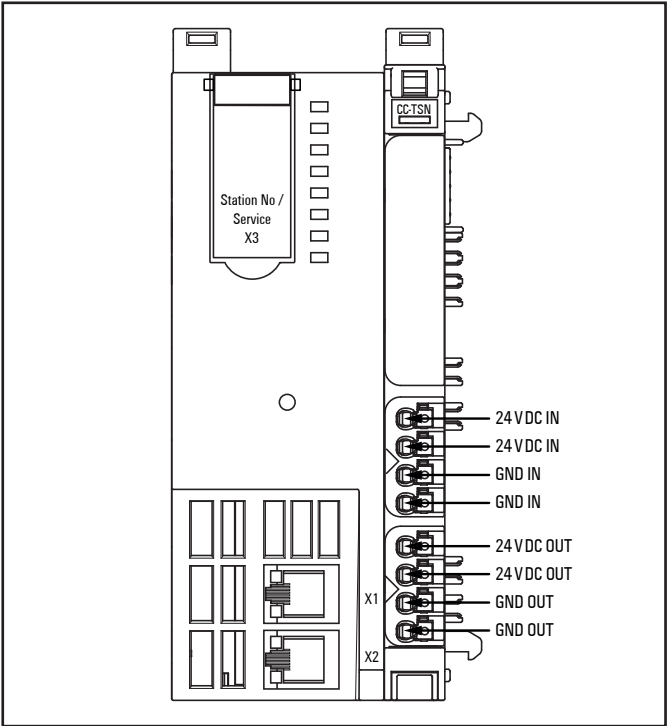
Connection diagram UR20-FBC-CC-TSN
