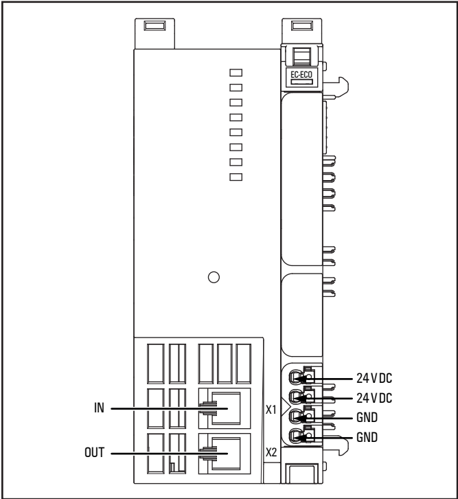
Connection diagram UR20-FBC-EC-ECO
