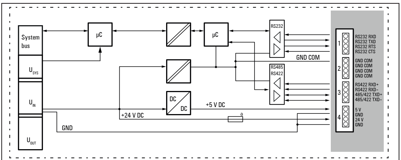
Block diagram UR20-1COM-232-485-422-V2
