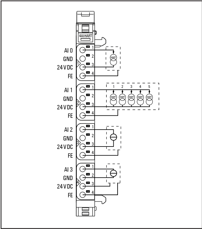
Connection diagram UR20-4AI-I-HART-16-DIAG showing several variants
