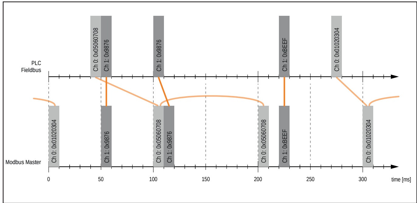
Modbus timing diagramm according to example
