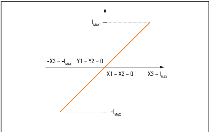
Characteristic curve for 1:1 scaling
