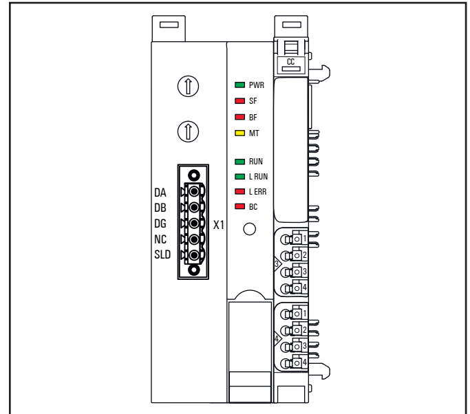
LED status indicators UR20-FBC-CC, error messages see chapter 12
