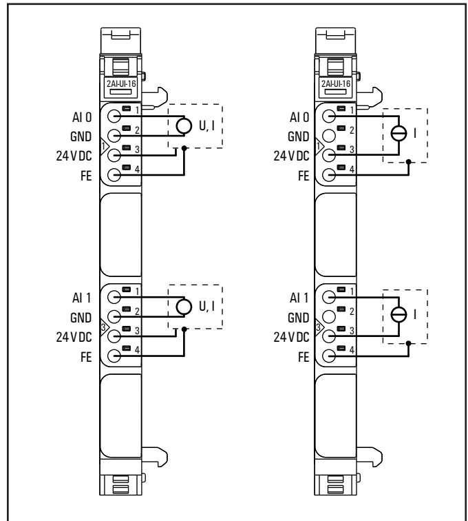
Connection diagram UR20-2AI-UI-16 (left 3/4-wire sensor with sensor wiring via electronics, right: 2-wire sensor with sensor wiring via electronics)
