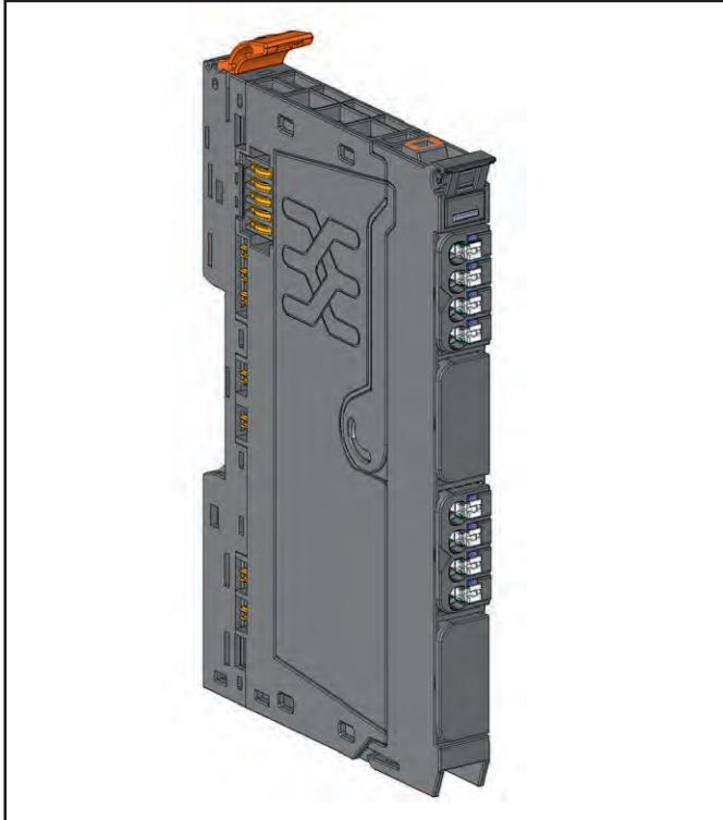
Analogue output module UR20-2AO-UI-16-DIAG (Order No. 2566100000)
