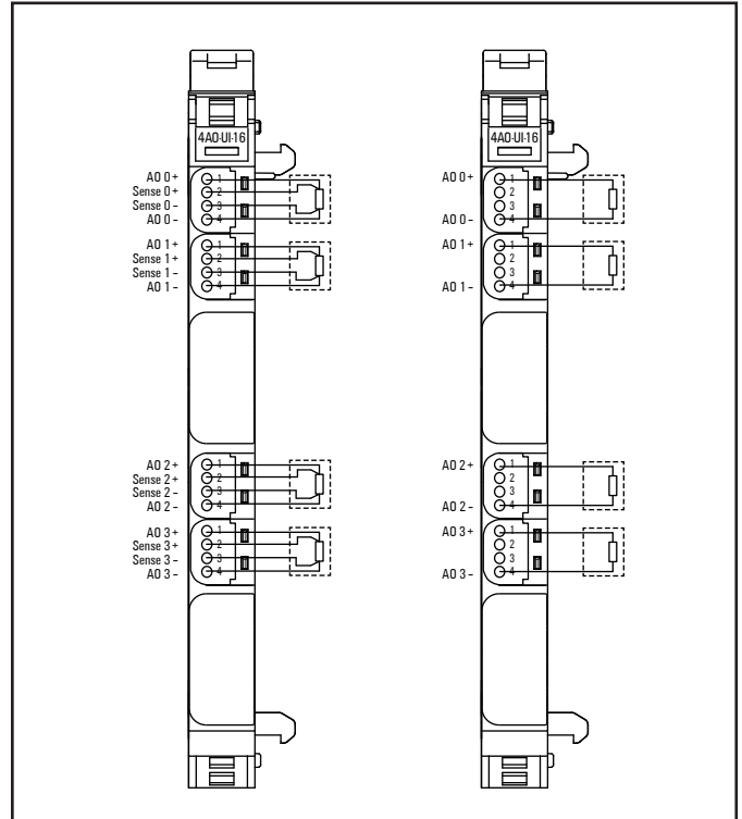
Connection diagram UR20-4AO-UI-16-HD
