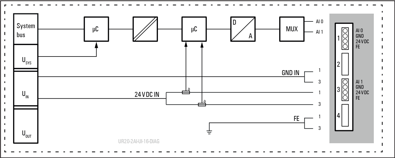
Block diagram UR20-2AI-UI-16-DIAG
