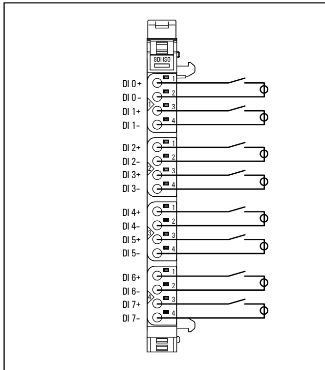
Connection diagram UR20-8DI-ISO-2W
