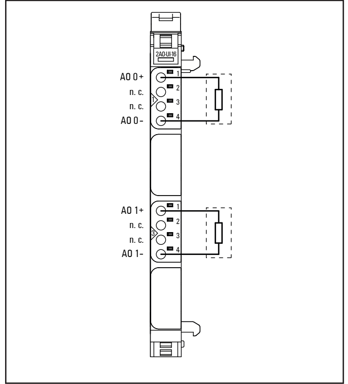
Connection diagram UR20-2AO-UI-ISO-16-DIAG
