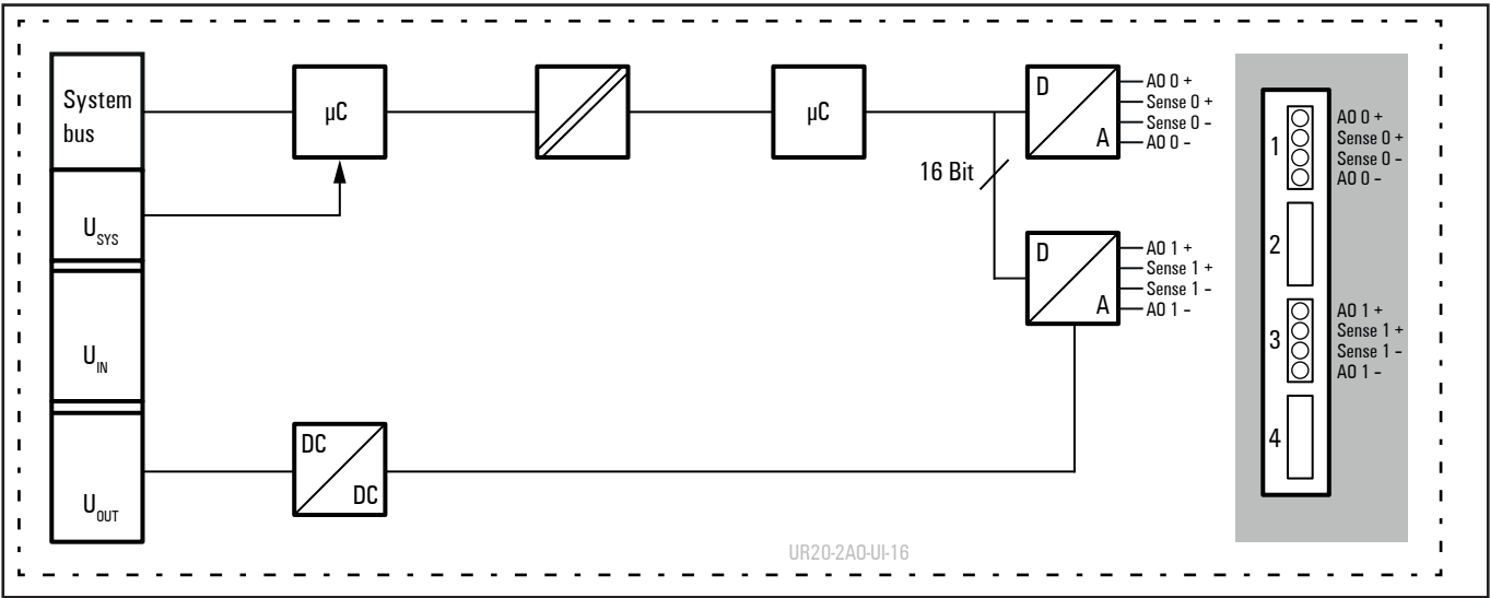
Block diagram UR20-2AO-UI-16
