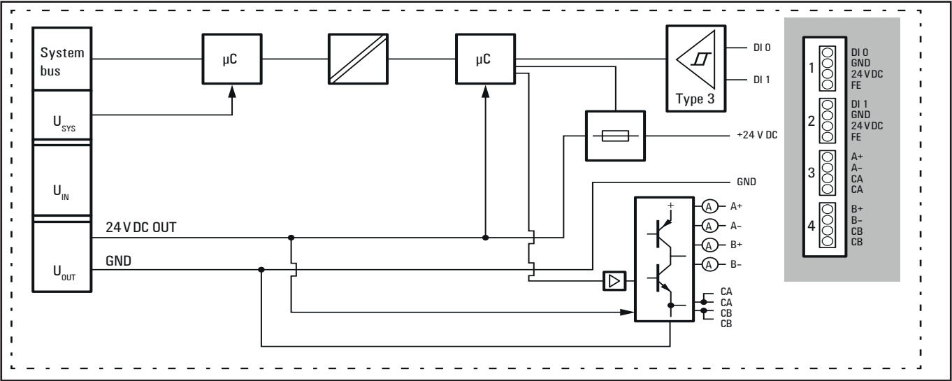
Block diagram UR20-2PWM-I-2.5A-2DI-P
