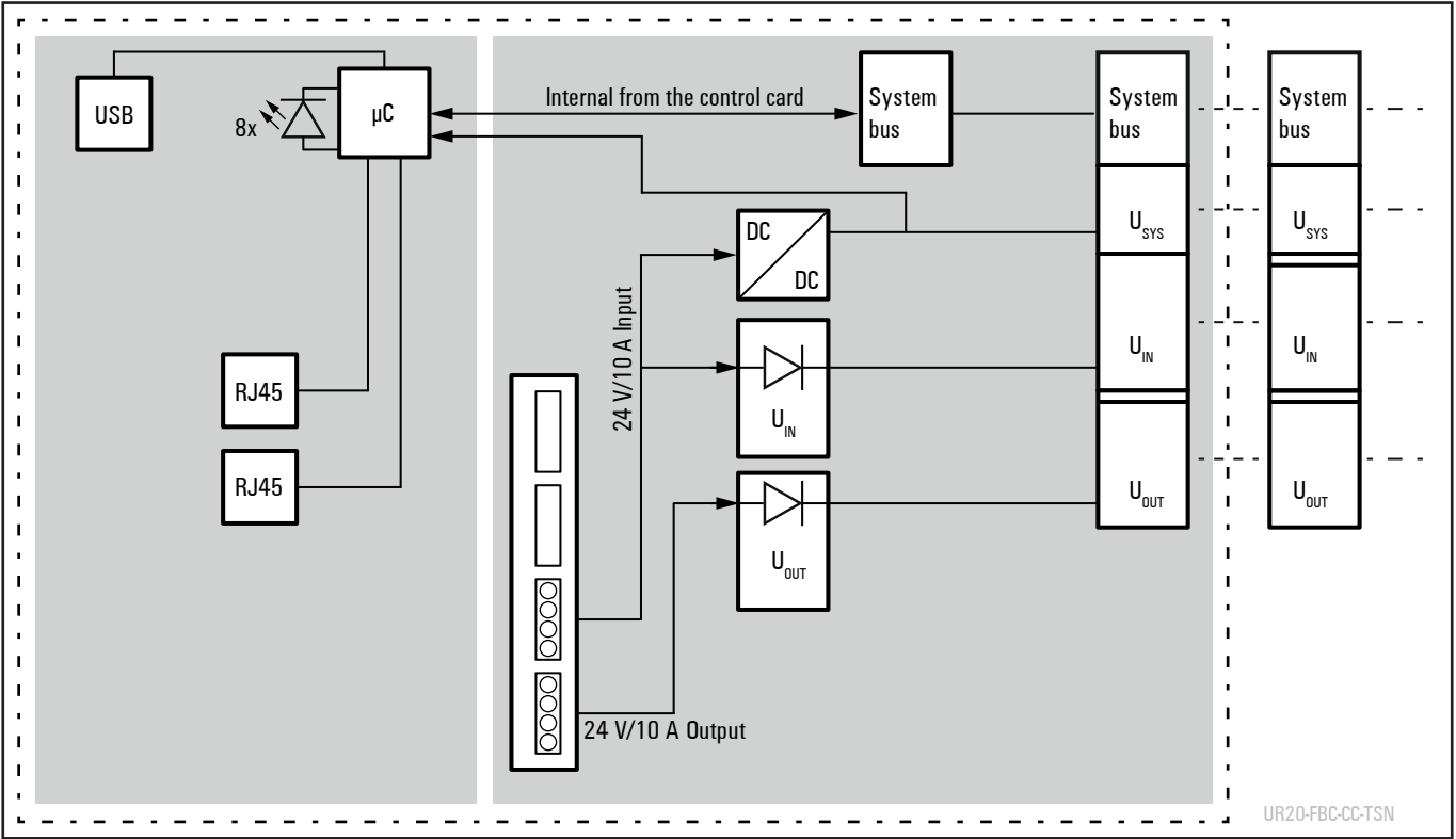
Block diagram UR20-FBC-CC-TSN
