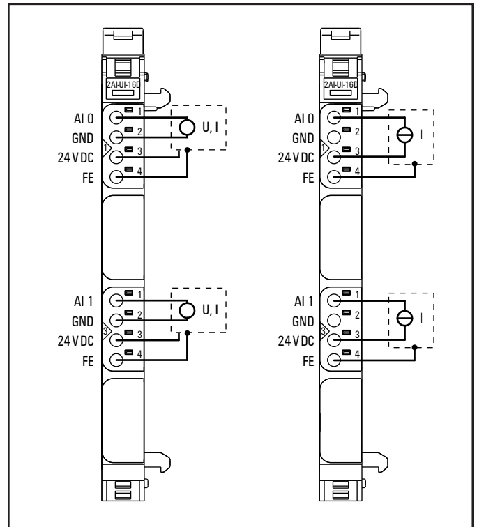
Connection diagram UR20-2AI-UI-16-DIAG (left 3/4-wire sensor with sensor wiring via electronics, right: 2-wire sensor with sensor wiring via electronics)
