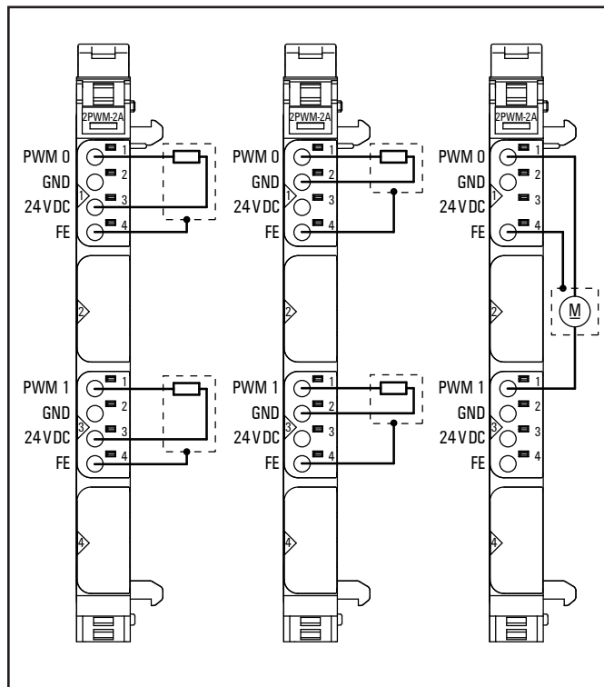
Connection diagram UR20-2PWM-PN-2A
