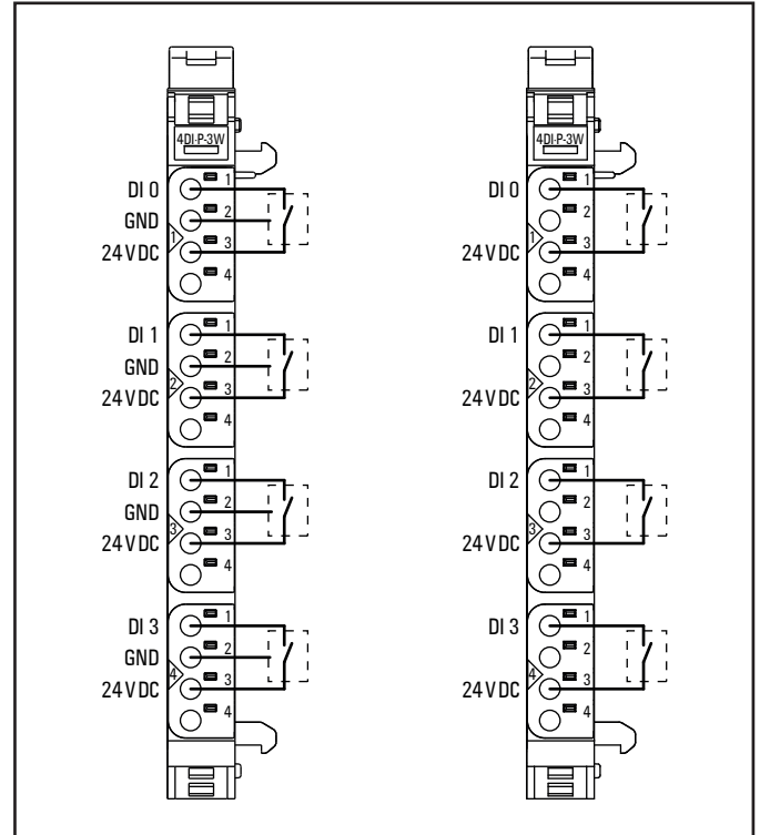
Connection diagram UR20-4DI-P-3W
