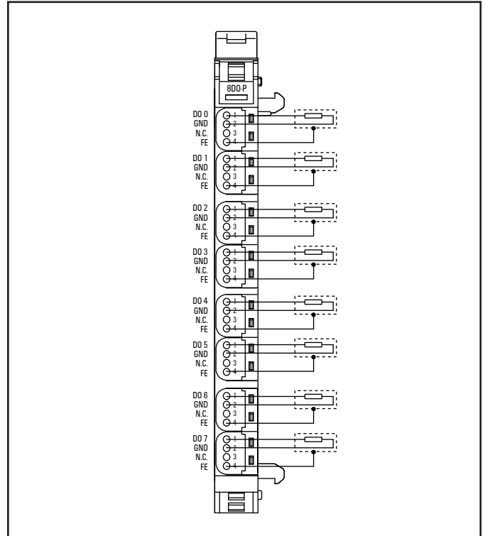
Connection diagram UR20-8DO-P-2W-HD
