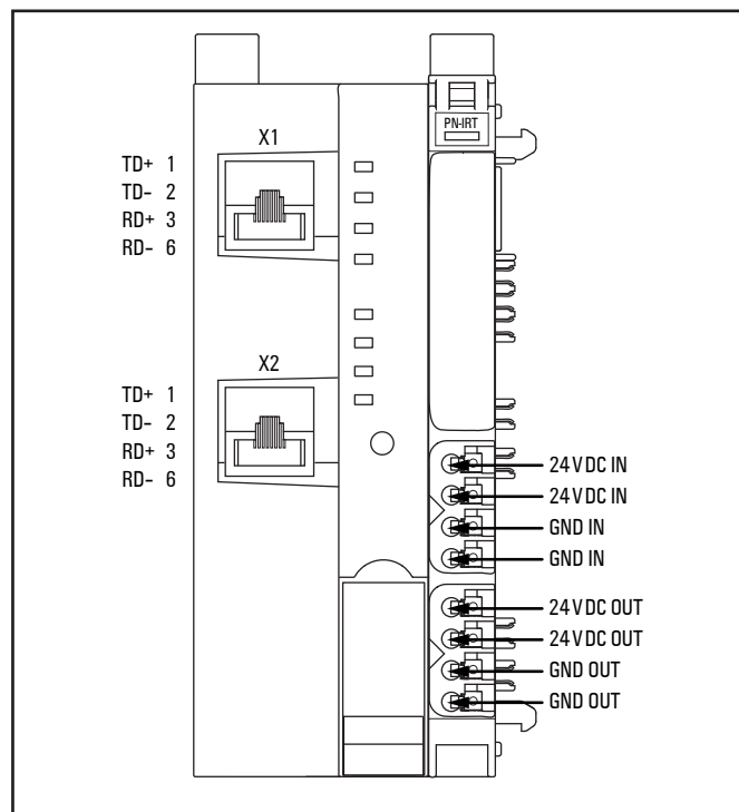
Connection diagram UR20-FBC-PN-IRT, UR20-FBC-PN-IRT-V2
