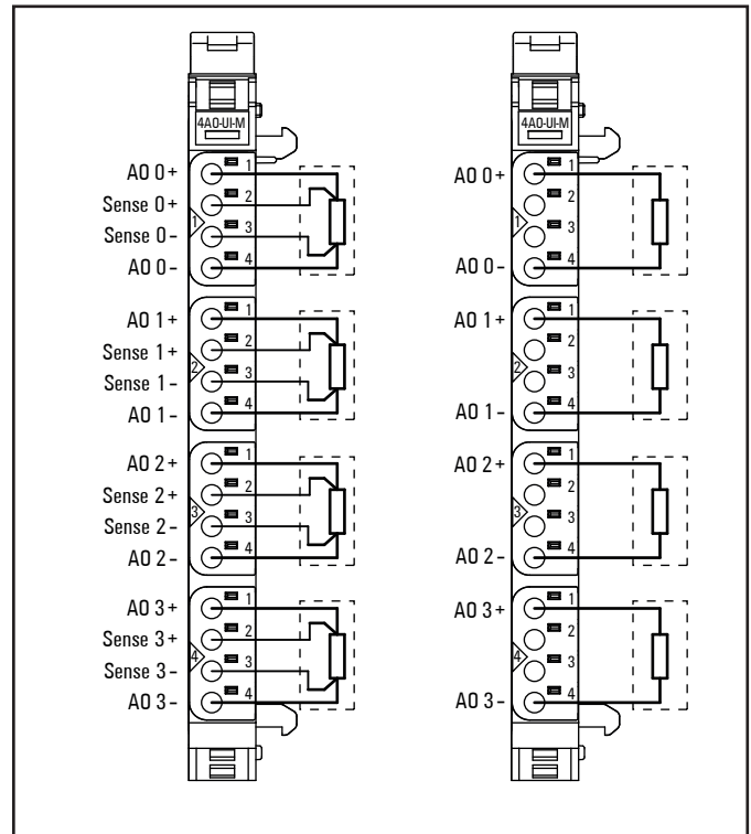
Connection diagram UR20-4AO-UI-16-M
