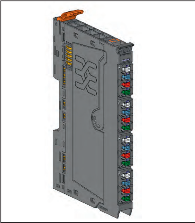
Analogue input module UR20-4AI-I-HART-16-DIAG (Order No. 2617520000)
