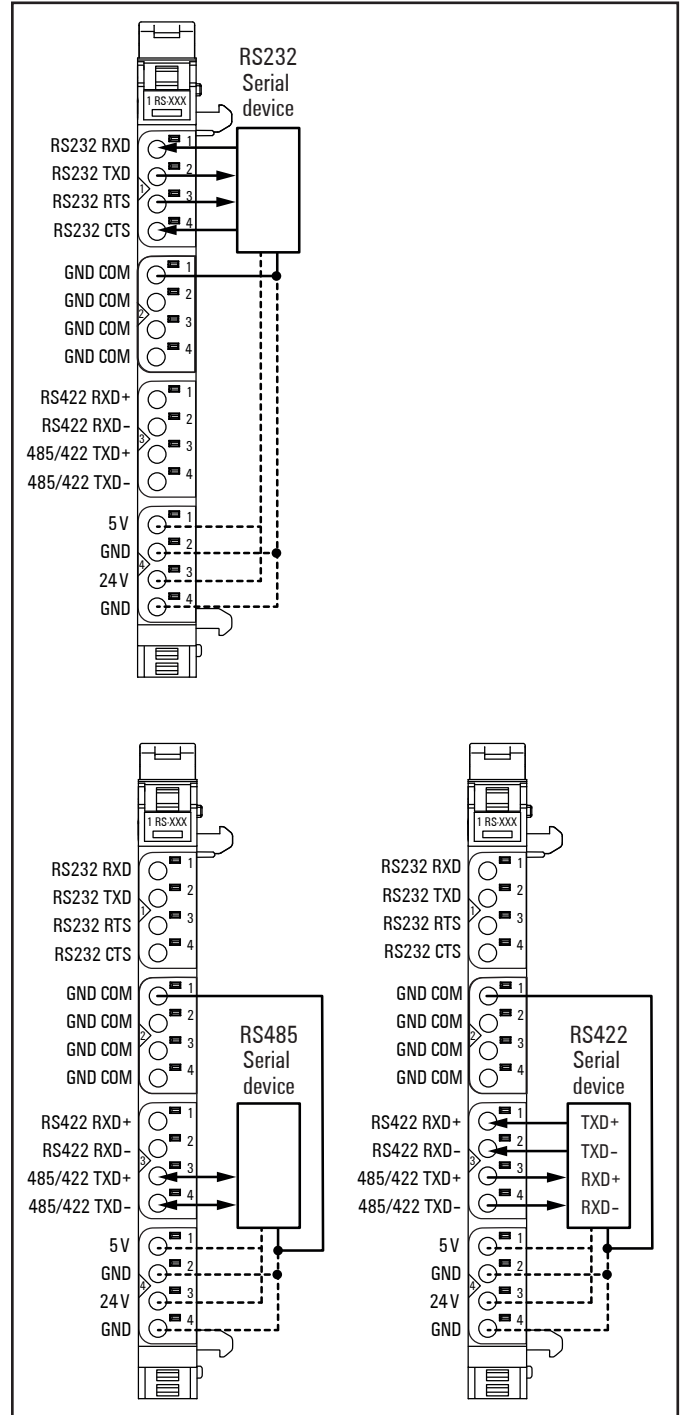
Connection diagram UR20-1COM-232-485-422-V2
