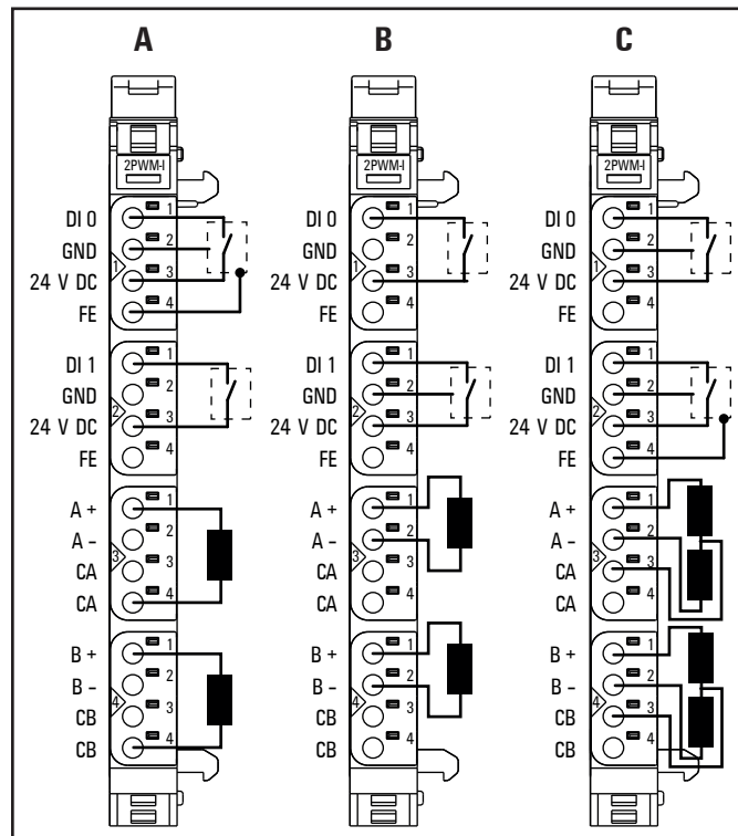
Connection diagram UR20-2PWM-I-2.5A-2DI-P (A: 2 coils unipolar, B: 2 coils bipolar, C: 2 × 2 coils unipolar in 3-wire technology)
