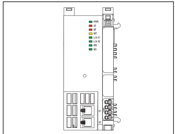
LED status indicators UR20-FBC-EIP-ECO, error messages see Chapter 12
