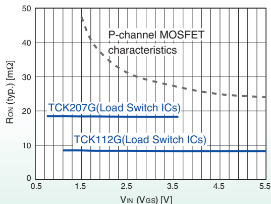
On-Resistance Characteristics of Load Switch ICs
